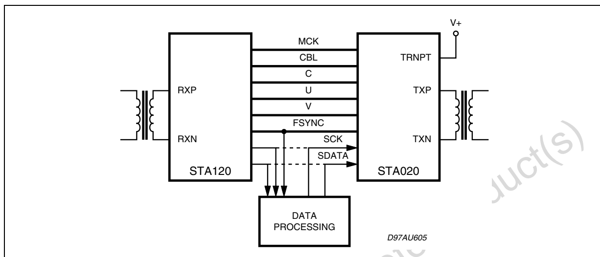
Figure 5. Transparent Mode Interface.
