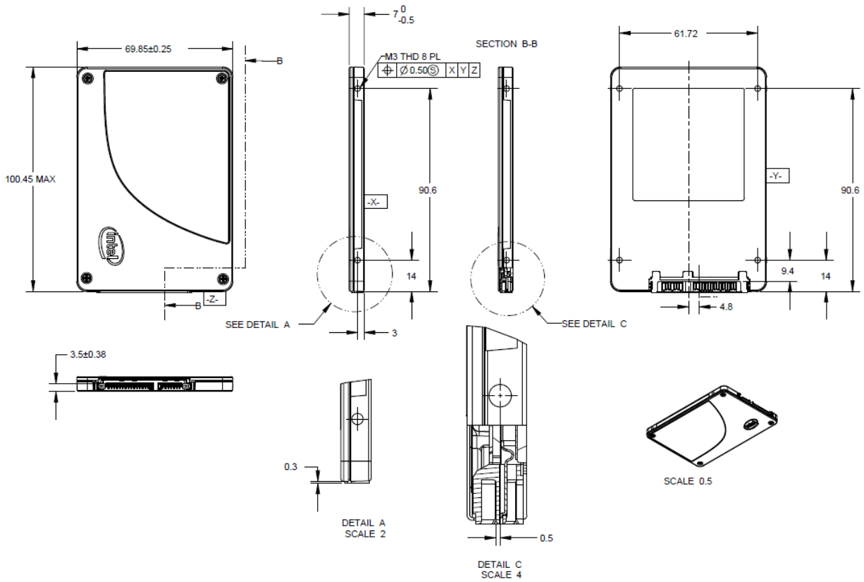
Figure 1: Intel SSD DC S3500 Series 2.5-inch Dimensions
