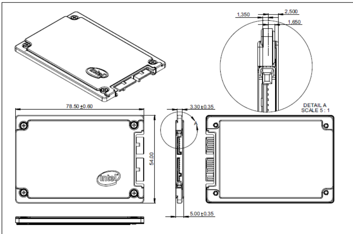
Figure 2: Intel® SSD DC S3500 Series 1.8 inch Dimensions
