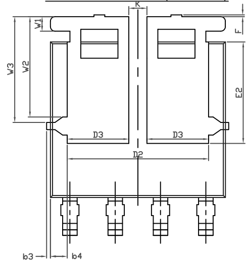
BACKSIDE VIEW(DUAL)
