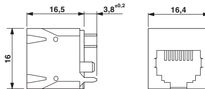
Dimensioned drawing
