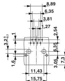
Drilling diagram
