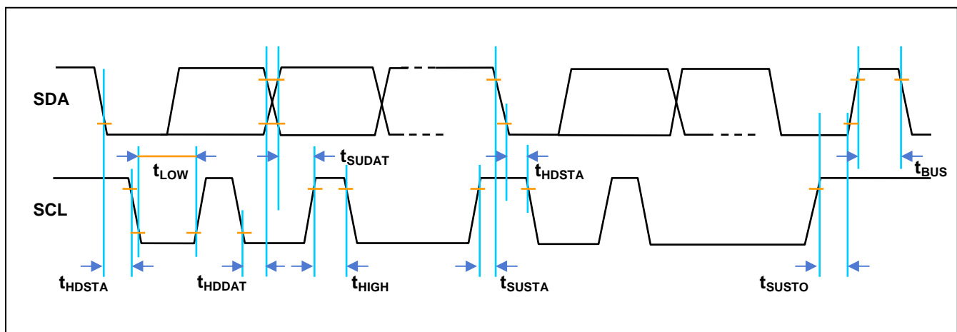
Figure 3.8 I 2 C Timing Diagram
