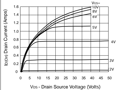
Output Characteristics
