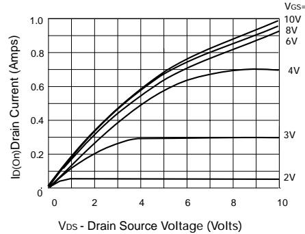
Saturation Characteristics
