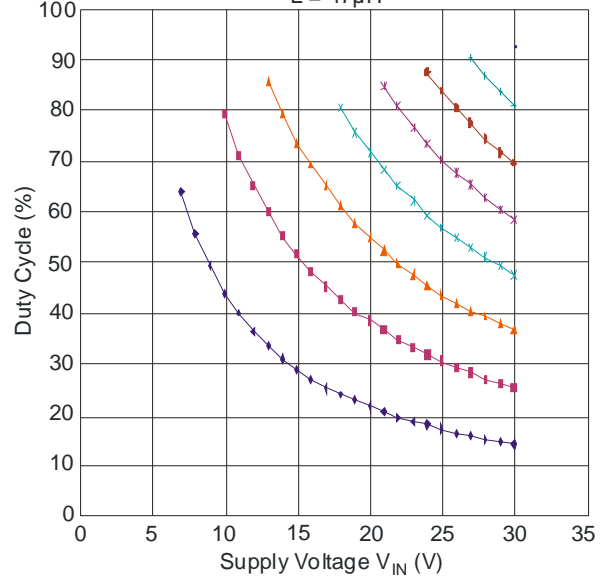
ZXLD1360 Duty Cycle L = 47μH
