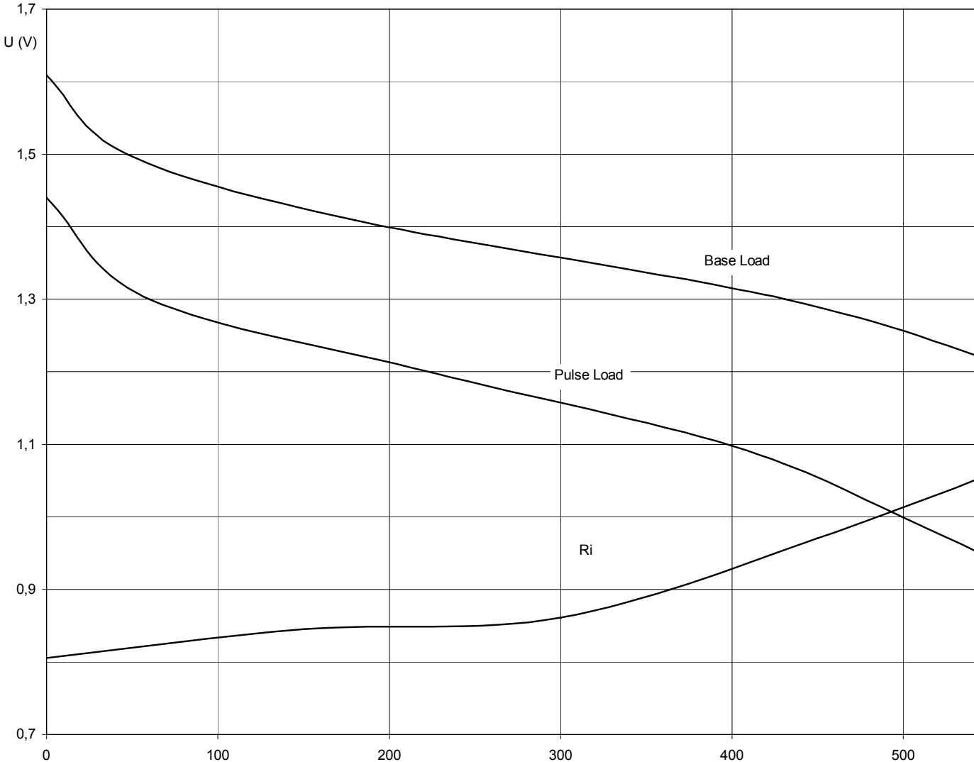
Internal Resistance at Continuous 1000 Ω, 1s/1h 2Ω
