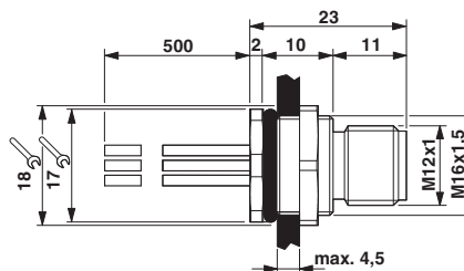
Dimensioned drawing
