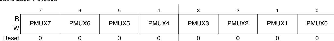
Figure 17-6. PIT Multiplex Register (PITMUX)
