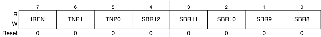
Figure 20-3. SCI Baud Rate Register (SCIBDH)
