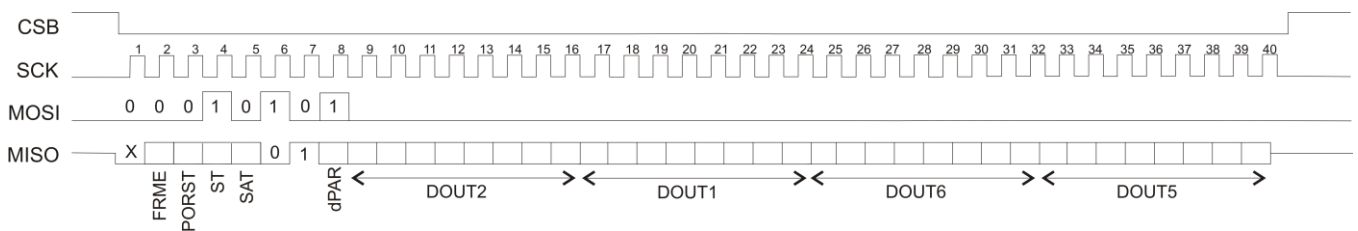
Figure 10: An example of decremental read operation.
