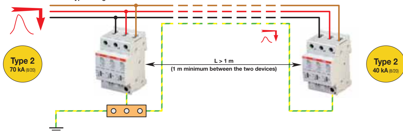
Coordination between Type 2 surge arresters
