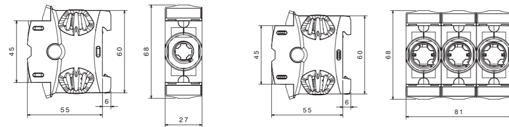
ISS 16/1 ISS 63/1
