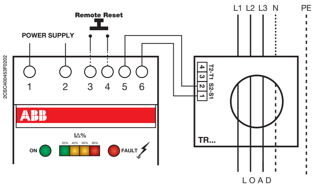
Toroid - relay connection
