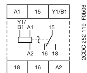
CT-TGD.12
