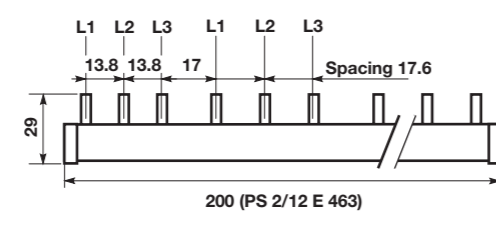
PS 3/12 E 463
