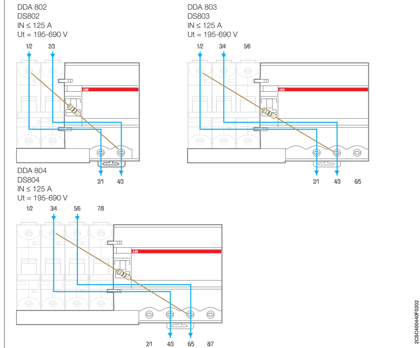
Maximum and minimum operating voltage of DDA 800 and DS800 test button
