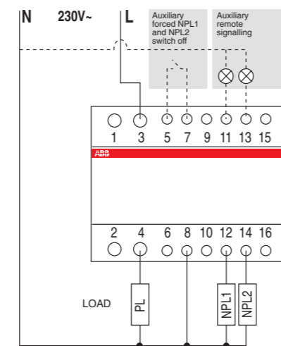
Single-phase wiring diagram
