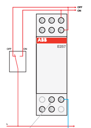
E 257 - permanently supplied It is possible to permanently supply the central command, for example using a change-over switch to control the relay.
