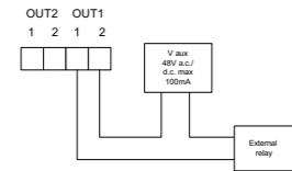
Digital output used as alarm with external relays for load command
