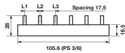
PS 3/6
