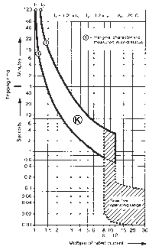
Characteristic S 700 K - K 63 to K 100
