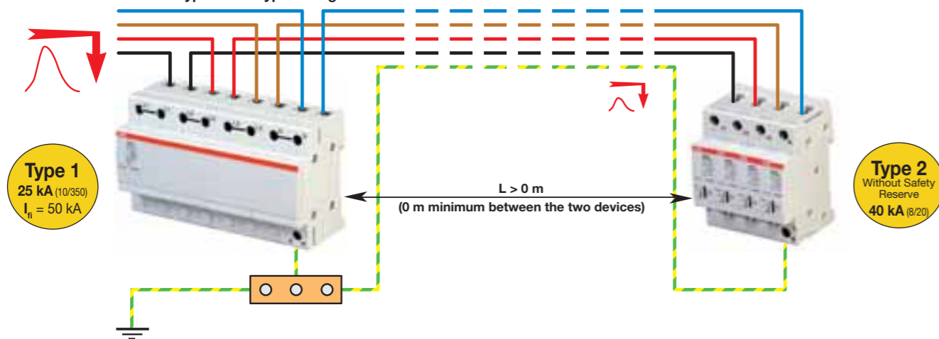
Coordination between Type 1 and Type 2 surge arrester
