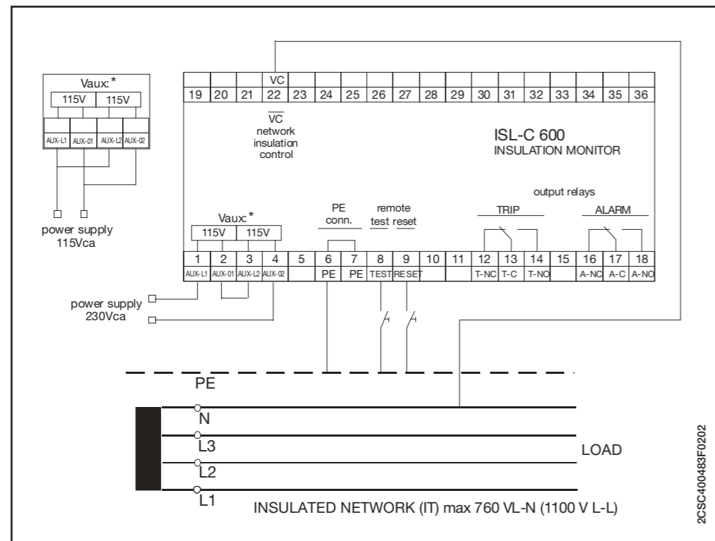
ISL-C 600
