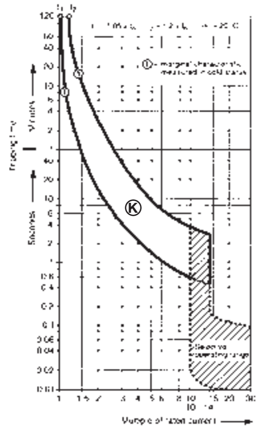
Characteristic S 700 K - K 16 to K 50
