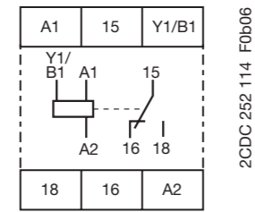
CT-MFD.12
