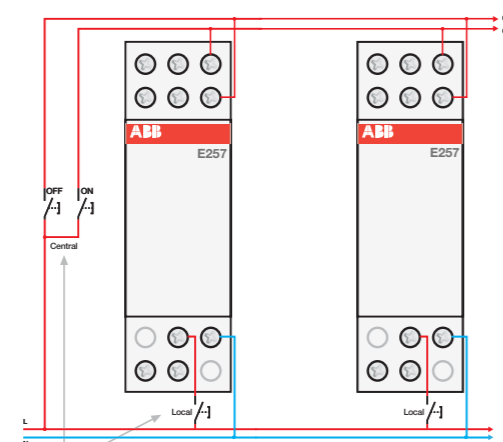
E 257 - local and central command by push-buttons Each local push-button controls a single relay. Pressing the central ON/OFF button puts all the relays in the ON (OFF) position irrespective of their previous state.
