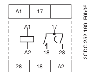
CT-SAD.22
