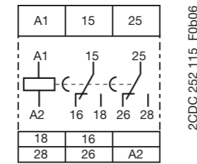
CT-ERD.22
