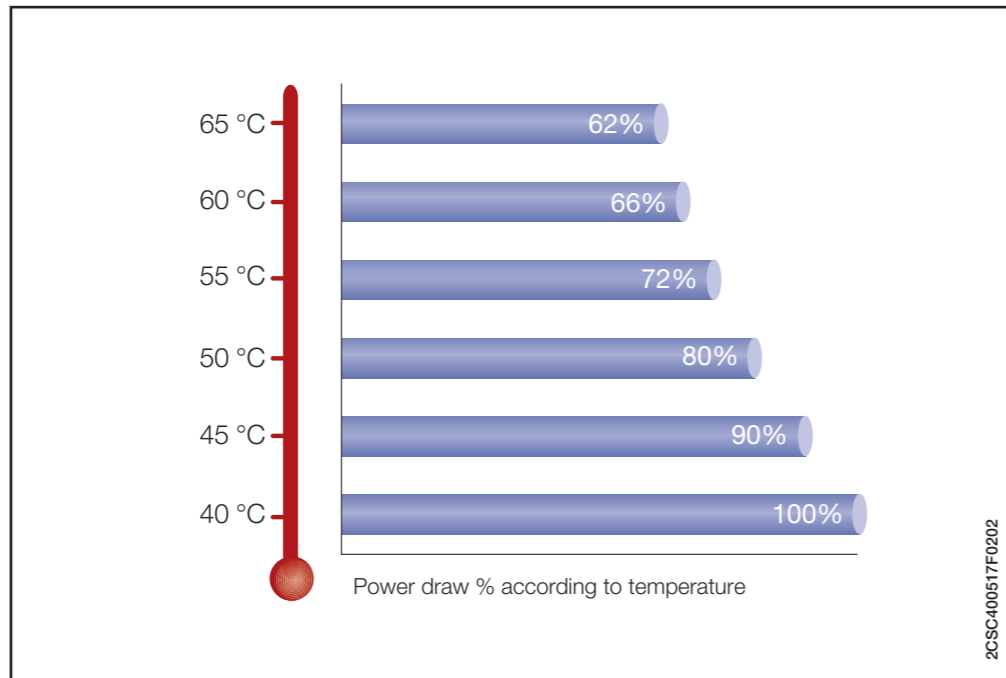
Power draw according to temperature and altitude
