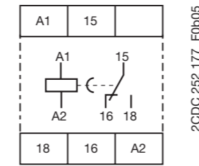
CT-ERD.12
