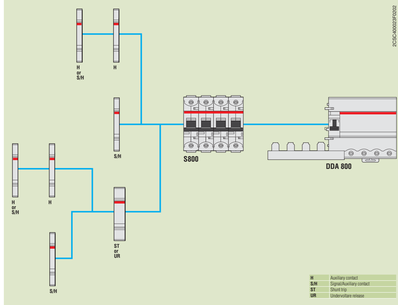
Combination between auxiliary elements and S800
