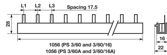
PS 3/60
