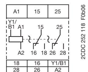
CT-TGD.22
