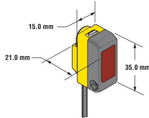
Opposed and Diffuse Models Suffix EB, RB, DB and W
