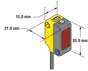
Adjustable-field Models Suffix AF100 and LAF
