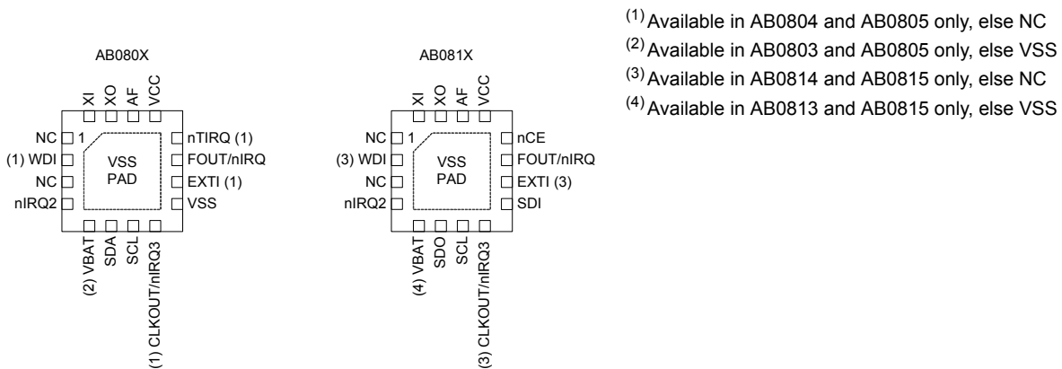
Figure 2. Pin Configuration Diagram
