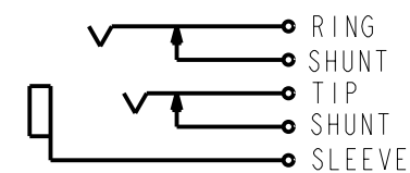
SCHEMATIC
