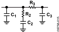
Figure 40. Third-Order Analog Loop Filter
