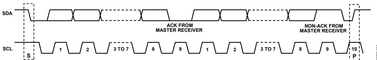
Figure 59. Data Transfer Process (Master Read Mode, 2-Byte Transfer)
