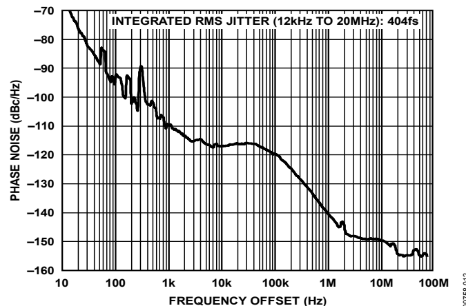
Figure 12. Absolute Phase Noise (Output Driver = HSTL), f_R = 19.44 MHz, f_{OUT} = 312.5 MHz, DPLL Loop BW = 0.1 Hz, f_{SYS} = 19.2 MHz TCXO
