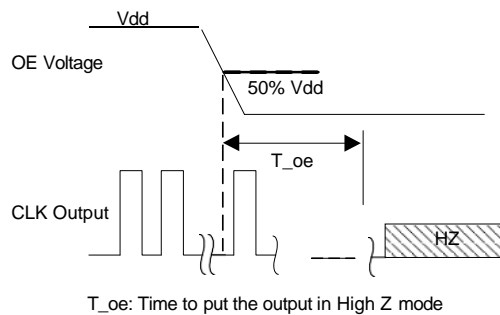
Figure 7. OE Disable Timing (OE Mode Only)
