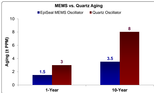
Figure 2. Aging Comparison [2]
