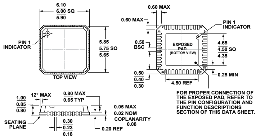
COMPLIANT TO JEDEC STANDARDS MO-220-VJJD-2 Figure 58. 40-Lead Lead Frame Chip Scale Package [LFCSP_VQ] 6 mm × 6 mm Body, Very Thin Quad (CP-40-13) Dimensions shown in millimeters
