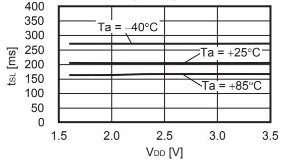
3.8 Sleep mode time ( t_{SL} ) vs. Power supply voltage ( V_{DD} )
