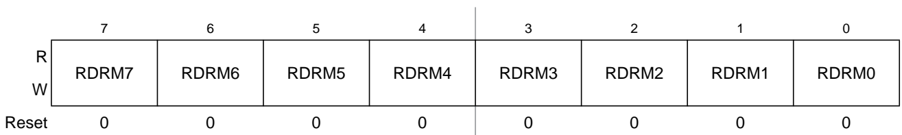
Figure 24-31. Port M Reduced Drive Register (RDRM)
