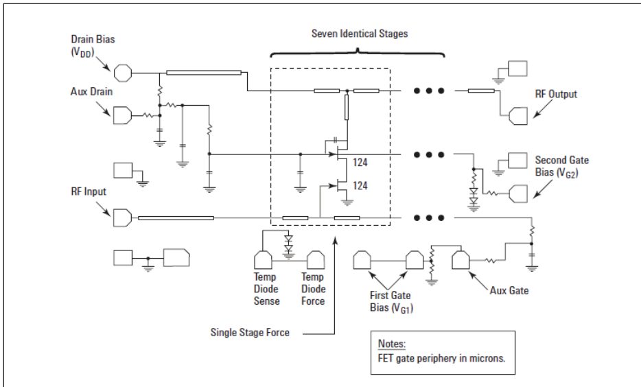
Figure 1. Schematic
