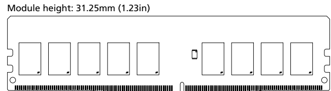
Figure 1: 288-Pin UDIMM (MO-309, R/C D1)
