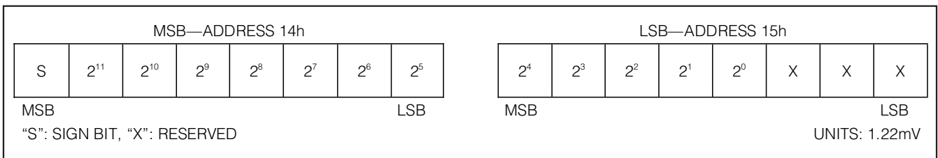
Figure 18. Initial Voltage Register Format
