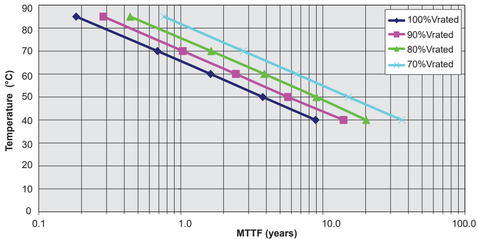
Expected Lifetime at Various Voltages SCM Series, 4.6V/4.2V, 6.4V Rated
