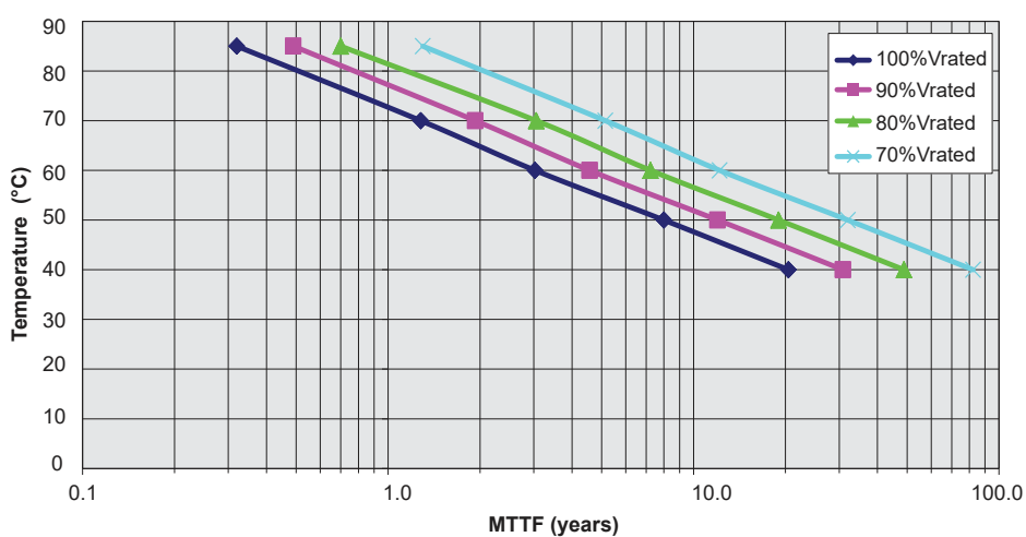
Expected Lifetime at Various Voltages SCM Series, 4.6V/4.2V, 6.4V Rated
