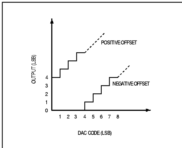
Figure 10. Single-Supply Offset
