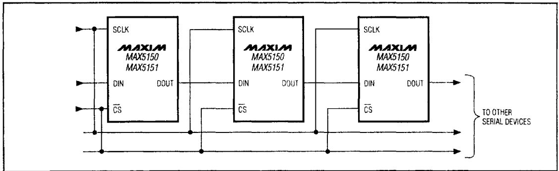
Figure 7. Daisy Chaining MAX5150/MAX5151s
