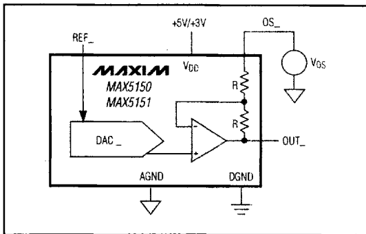
Figure 10. Setting OS 1 for Output Offset
