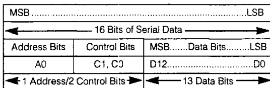
Figure 4. Serial-Data Format
