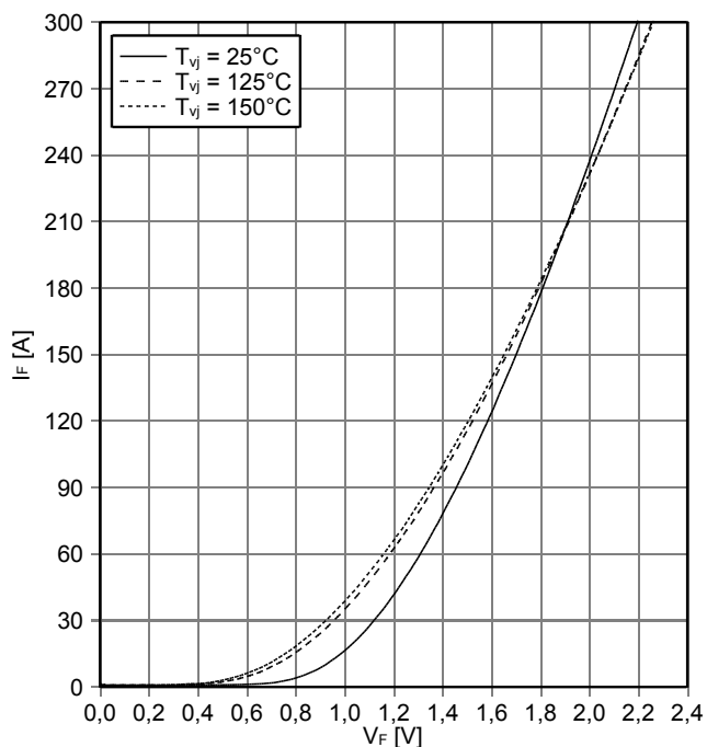
正向偏压特性 Diode-斩波器 (典型) forward characteristic of Diode-Chopper (typical)
