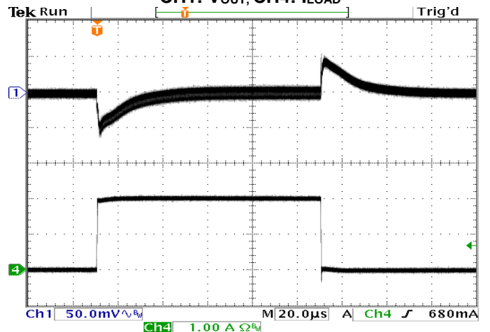
Transient Response at V_{IN} = 5\text{ V} V_{OUT} = 3.3\text{ V} , C_{OUT} = 1 \times 47\ \mu\text{F} (0-2 A Load Step, slew rate \geq 10\text{ A}/\mu\text{s} ) CH1: V_{OUT} , CH4: I_{LOAD}
