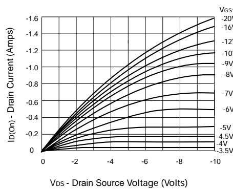
Saturation Characteristics
