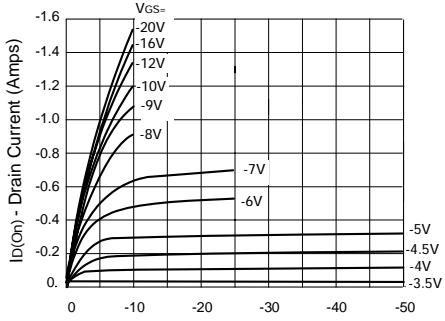
Output Characteristics
