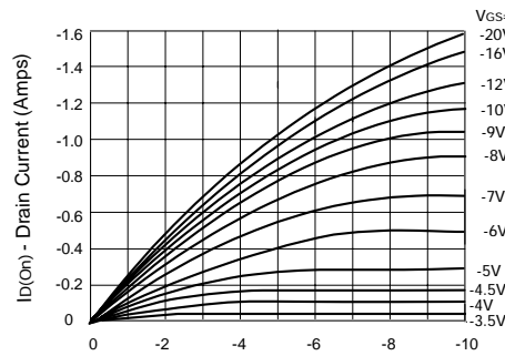
Saturation Characteristics
