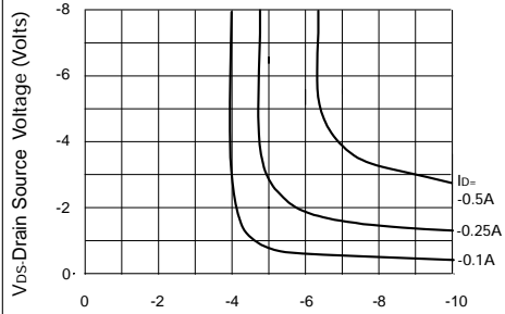
Voltage Saturation Characteristics
