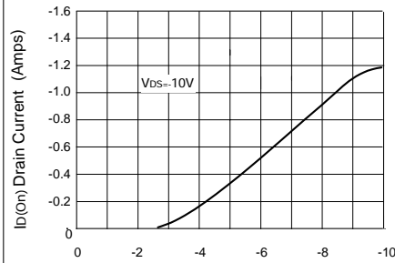
Transfer Characteristics
