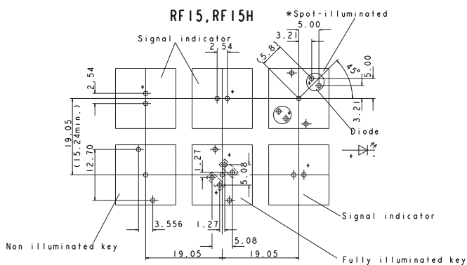
View on component side, all hole diameters 1.1 \pm 0.1 mm
