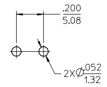
RECOMMENDED PCB HOLE LAYOUT
