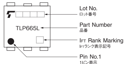
(b) 5 pin DIP6 Package (TLP665L)
