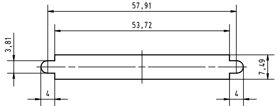
Panel cutout
