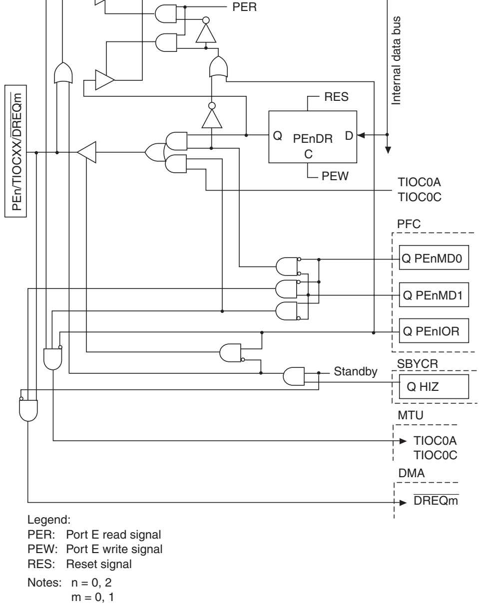
Figure B.24 PEn/TIOCXX/DREQm Block Diagram
