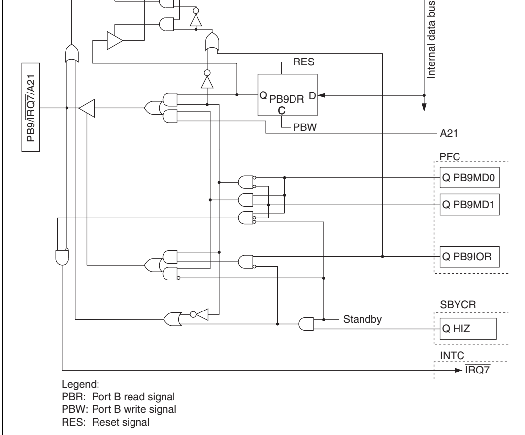
Figure B.15 PB9/IRQ7/A21 Block Diagram
