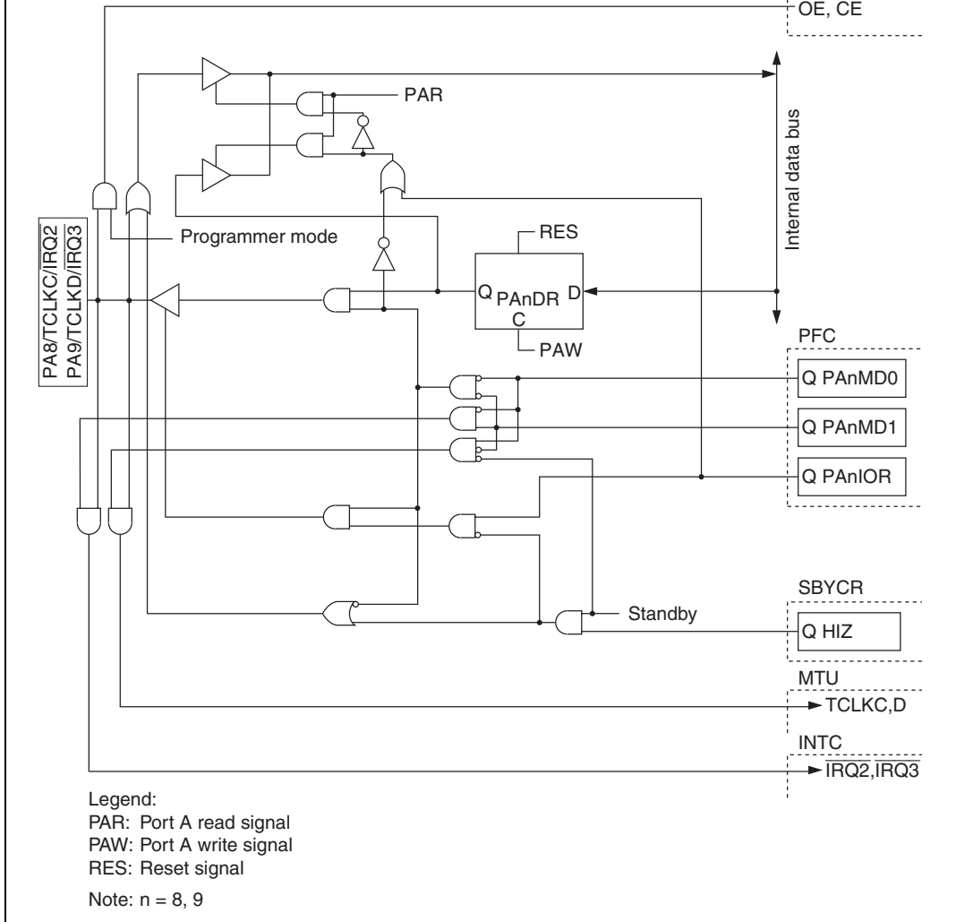
Figure B.6 PAn/TCLKm/IRQx Block Diagram (F-ZTAT Version)
