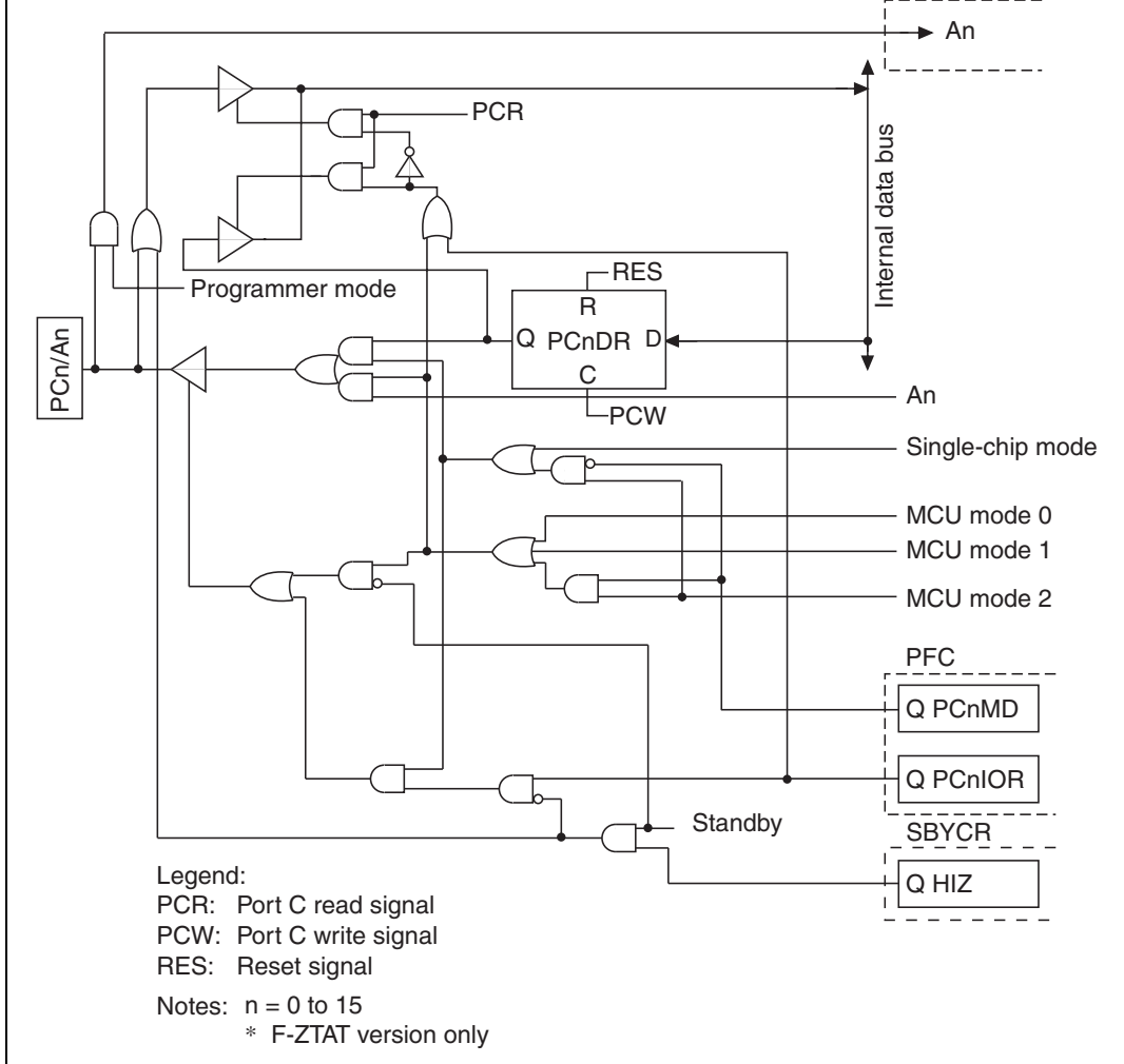
Figure B.17 PCn/An Block Diagram
