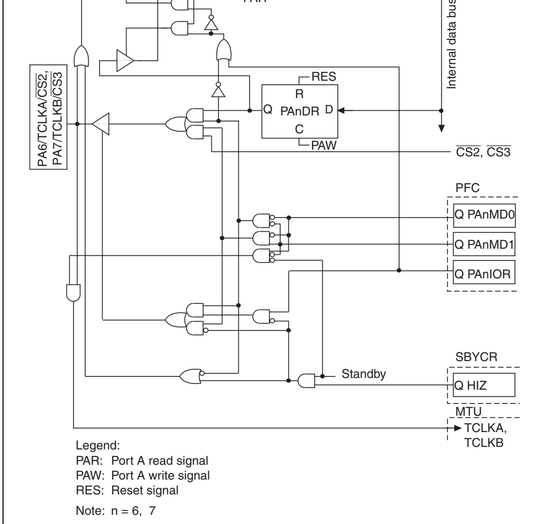
Figure B.3 PA6/TCLKA/CS2, PA7/TCLKB/CS3 (SH7014, Mask) Block Diagram
