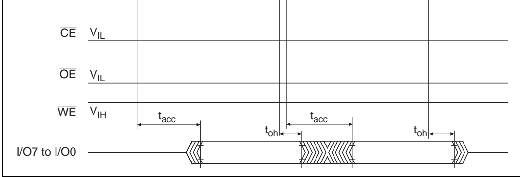
Figure 18.22 \overline{CE} and \overline{OE} Enable State Read Timing Waveforms
