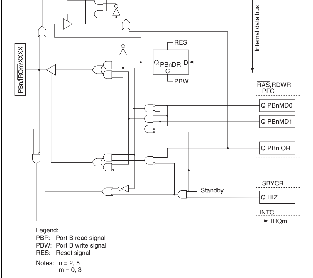
Figure B.16 \overline{\text{PBn}}/\overline{\text{IRQm}}/\text{XXXX} Block Diagram
