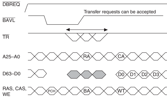
Figure 14.39 Write to Synchronous DRAM Non-Precharge Bank (Row Miss)
