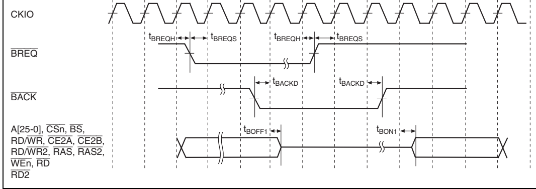
Figure 22.13 Control Signal Timing
