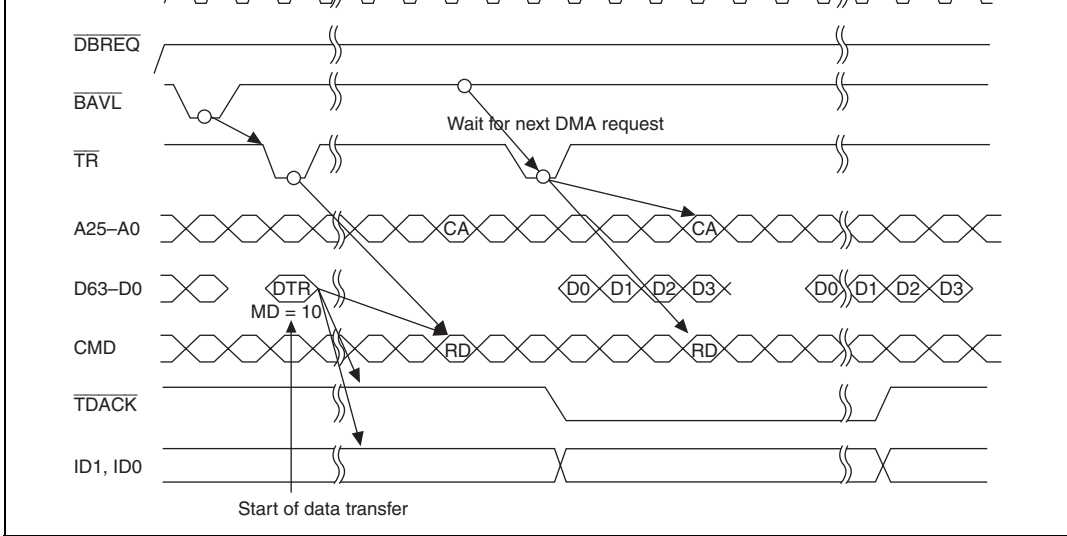
Figure 14.44 Single Address Mode/Burst Mode/Level Detection/ External Bus → External Device Data Transfer
