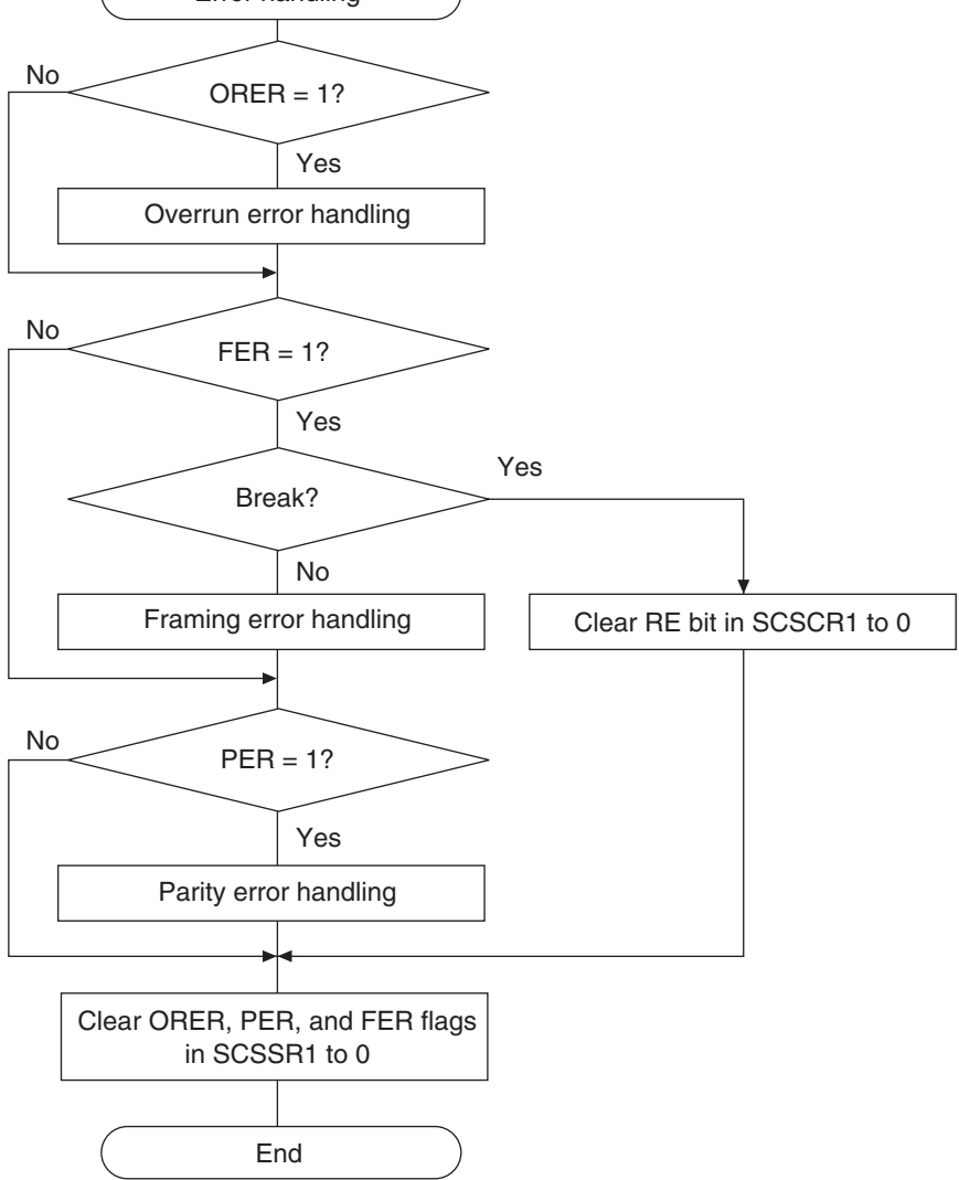
Figure 15.10 Sample Serial Reception Flowchart (2)
