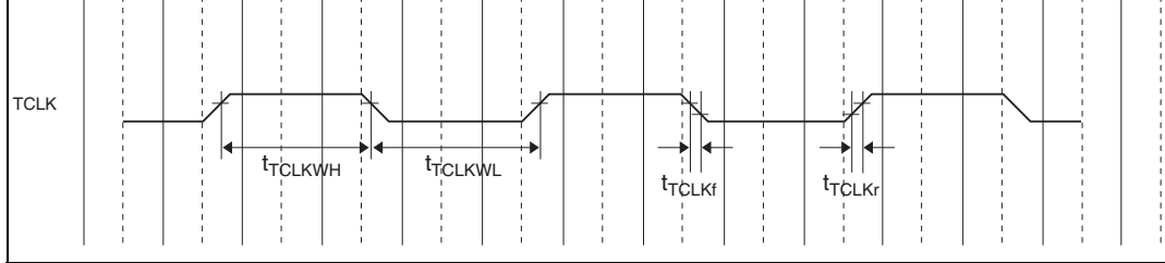
Figure 22.61 TCLK Input Timing
