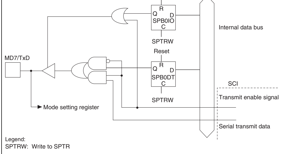
Figure 15.3 MD7/TxD Pin
