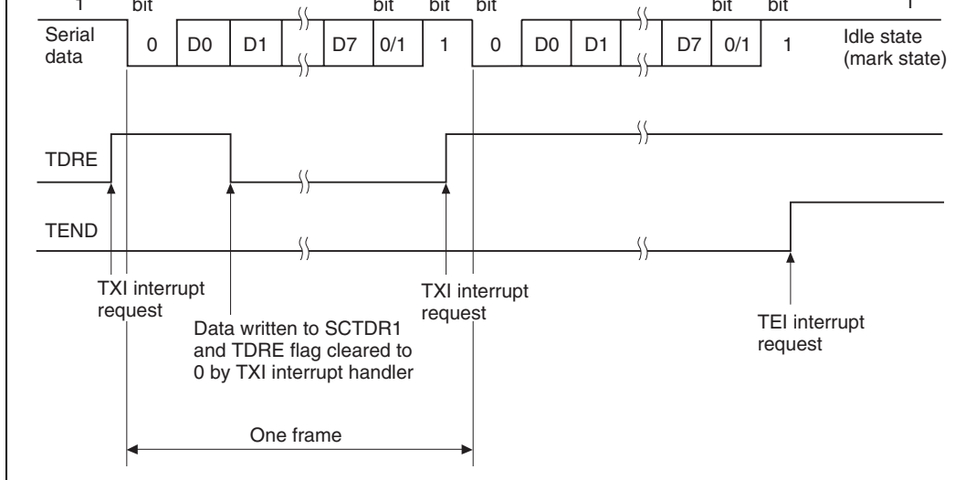
Figure 15.9 Example of Transmit Operation in Asynchronous Mode (Example with 8-Bit Data, Parity, One Stop Bit)
