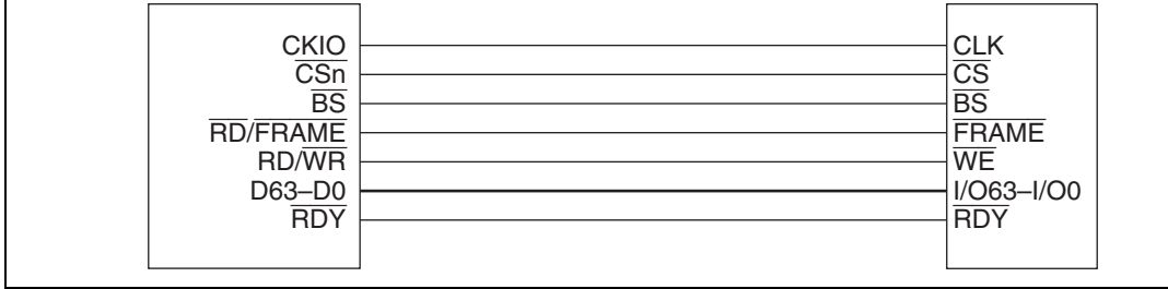
Figure 13.57 Example of 64-Bit Data Width MPX Connection
