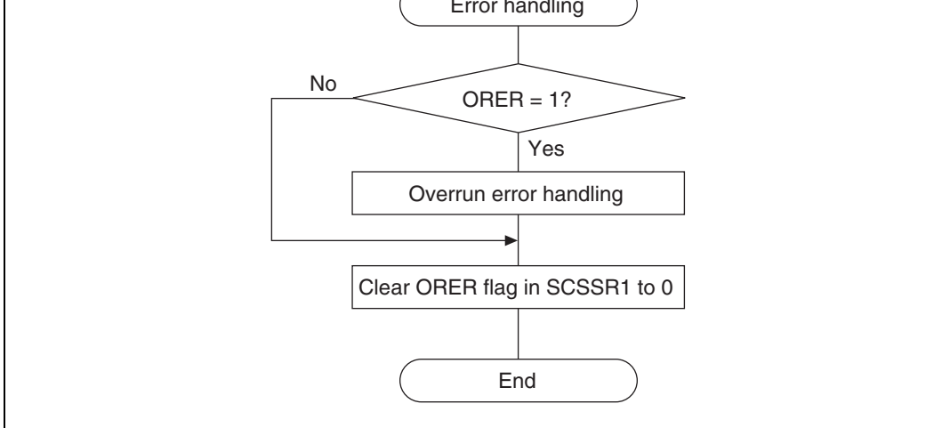
Figure 15.21 Sample Serial Reception Flowchart (2)
