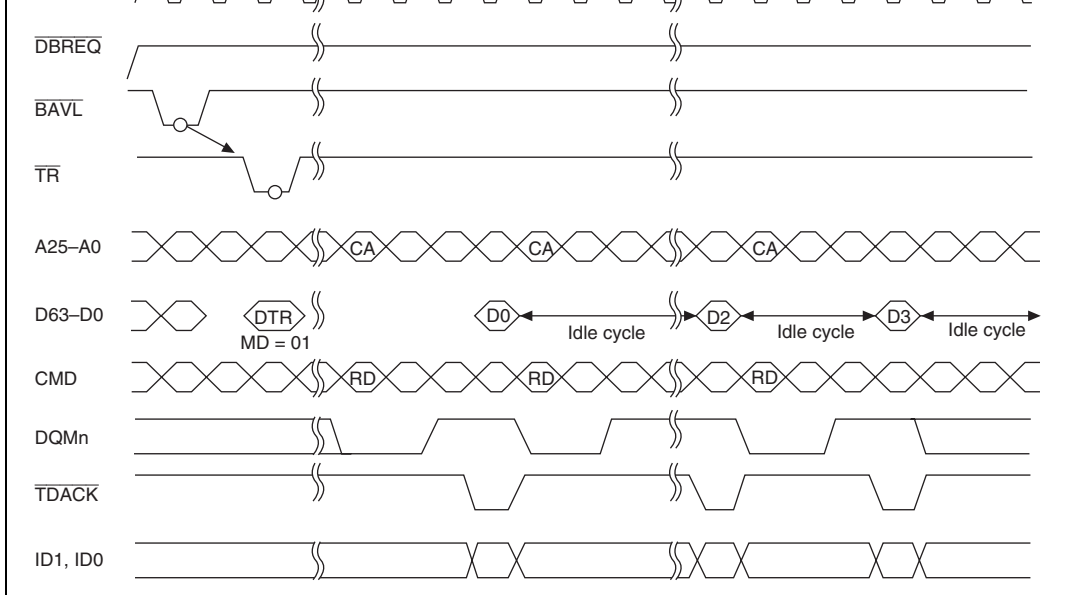
Figure 14.45 Single Address Mode/Burst Mode/Edge Detection/Byte, Word, Longword, Quadword/External Bus → External Device Data Transfer
