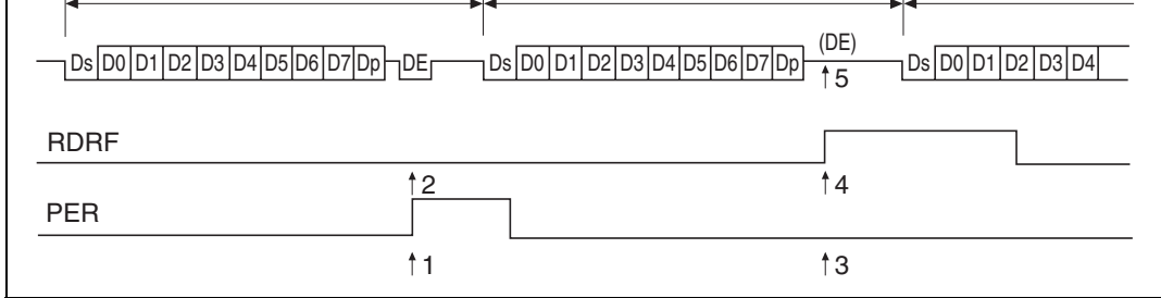
Figure 17.11 Retransfer Operation in SCI Receive Mode
