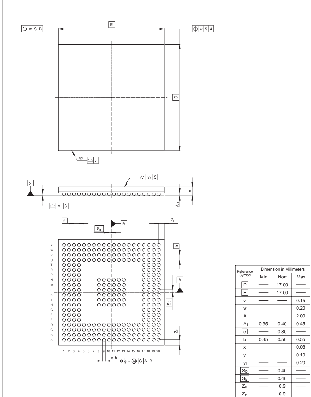
Figure B.4 Package Dimensions (292-Pin BGA)
