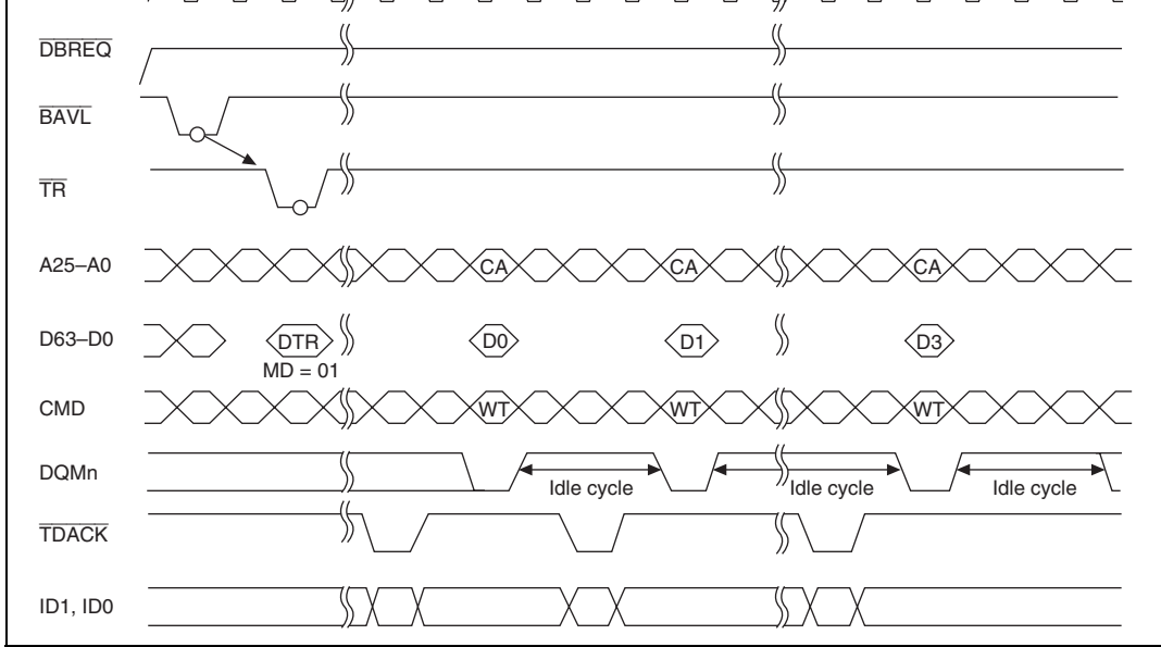
Figure 14.46 Single Address Mode/Burst Mode/Edge Detection/Byte, Word, Longword, Quadword/External Device → External Bus Data Transfer
