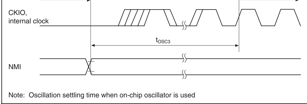
Figure 22.7 Standby Return Oscillation Settling Time (Return by NMI)
