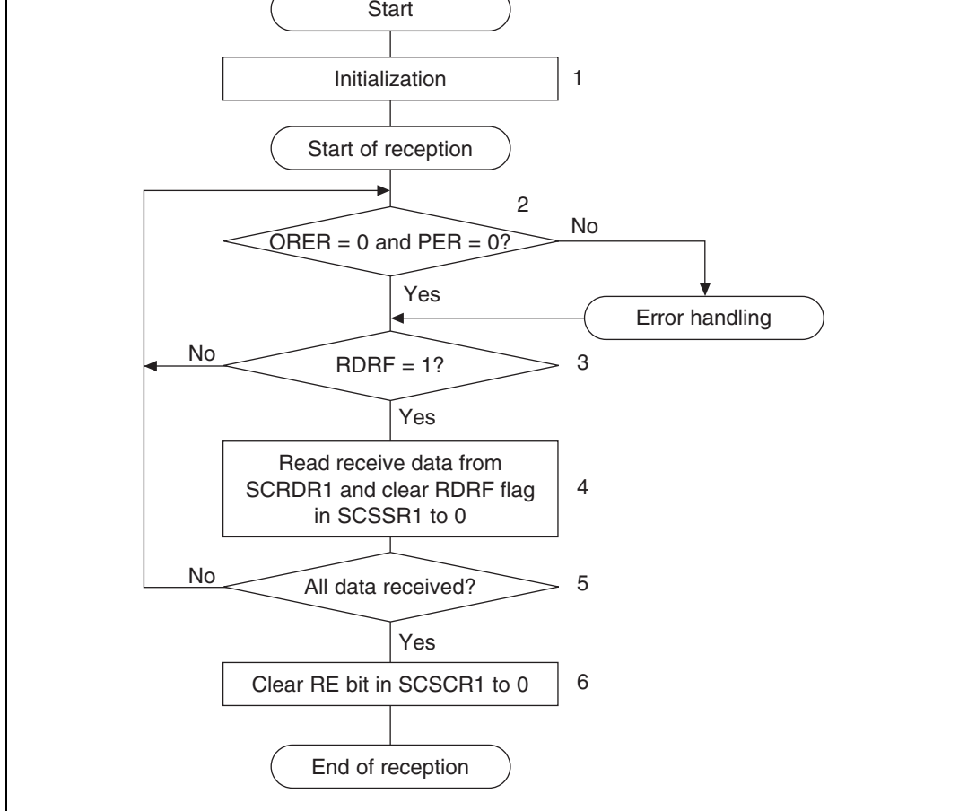
Figure 17.9 Sample Reception Processing Flowchart
