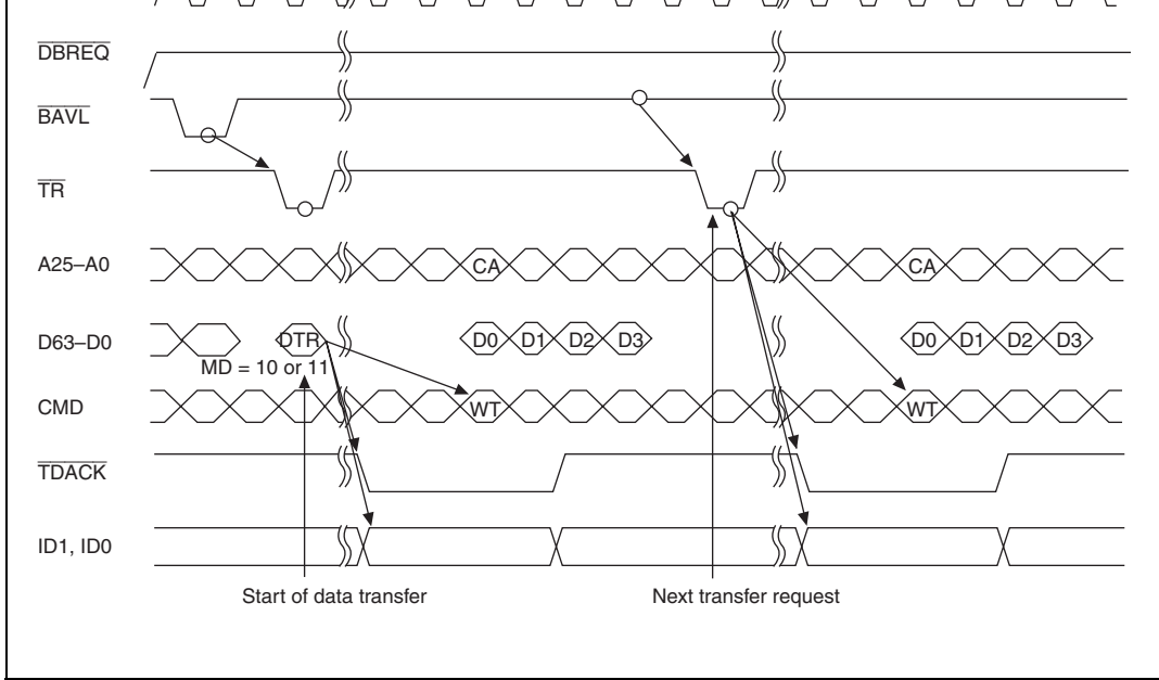
Figure 14.34 Handshake Protocol without Use of Data Bus (Channel 0 On-Demand Data Transfer)
