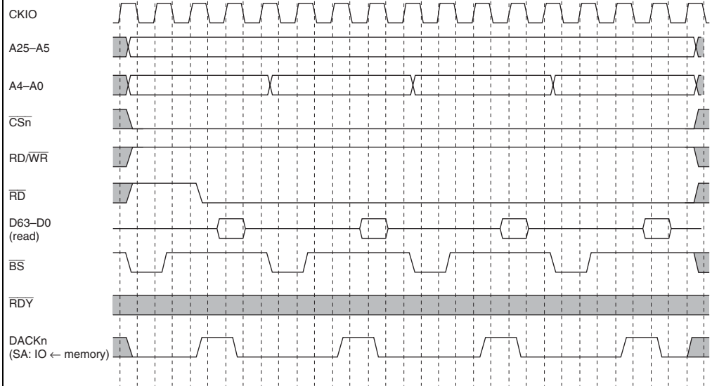
Figure 13.49 Burst ROM Wait Access Timing
