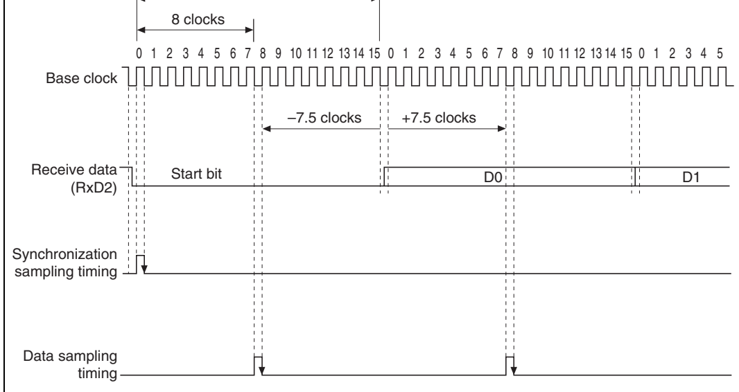
Figure 16.13 Receive Data Sampling Timing in Asynchronous Mode
