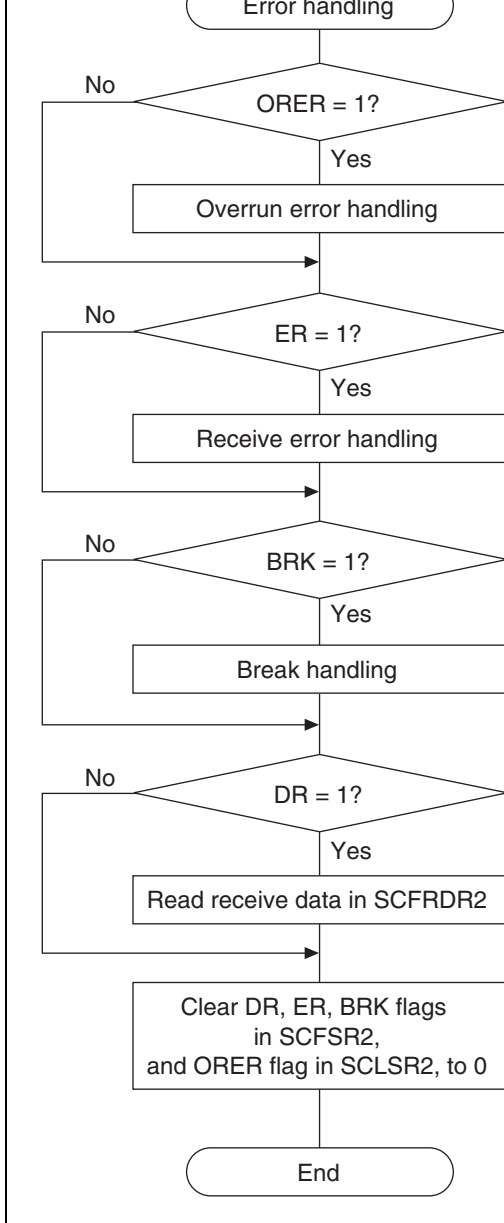
Figure 16.10 Sample Serial Reception Flowchart (2)
