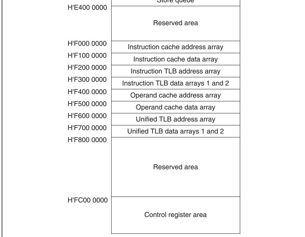
Figure 3.4 P4 Area
