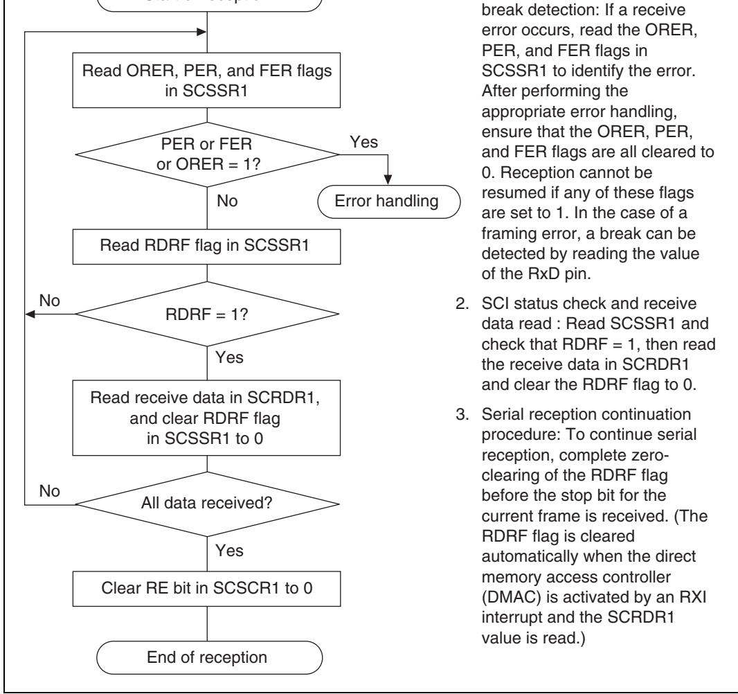
Figure 15.10 Sample Serial Reception Flowchart (1)
