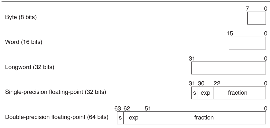
Figure 2.1 Data Formats
