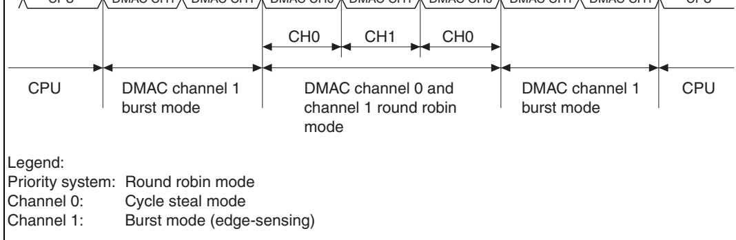
Figure 14.11 Bus Handling with Two DMAC Channels Operating
