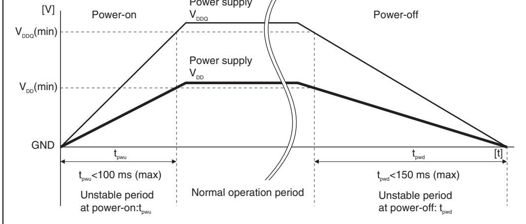
Figure H.2 Power-On Procedure 2
