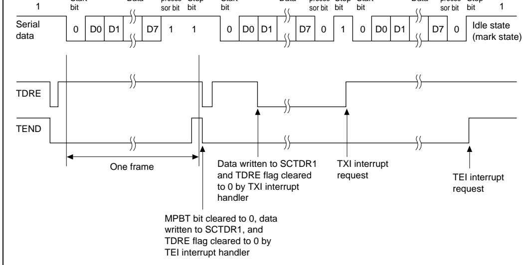
Figure 15.14 Example of SCI Transmit Operation (Example with 8-Bit Data, Multiprocessor Bit, One Stop Bit)
