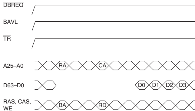
Figure 14.35 Read from Synchronous DRAM Precharge Bank
