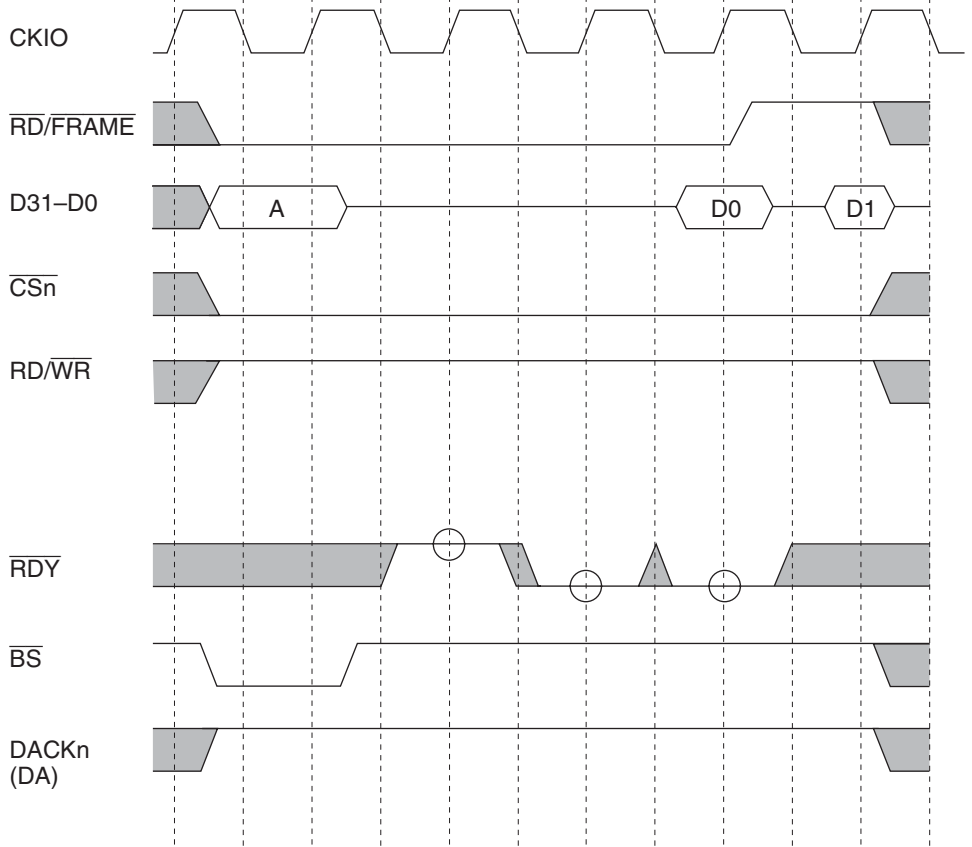
Figure 13.67 MPX Interface Timing 10 (Burst Read Cycle, AnW = 0, One External Wait Inserted, Bus Width: 32 Bits, Transfer Data Size: 64 Bits)
