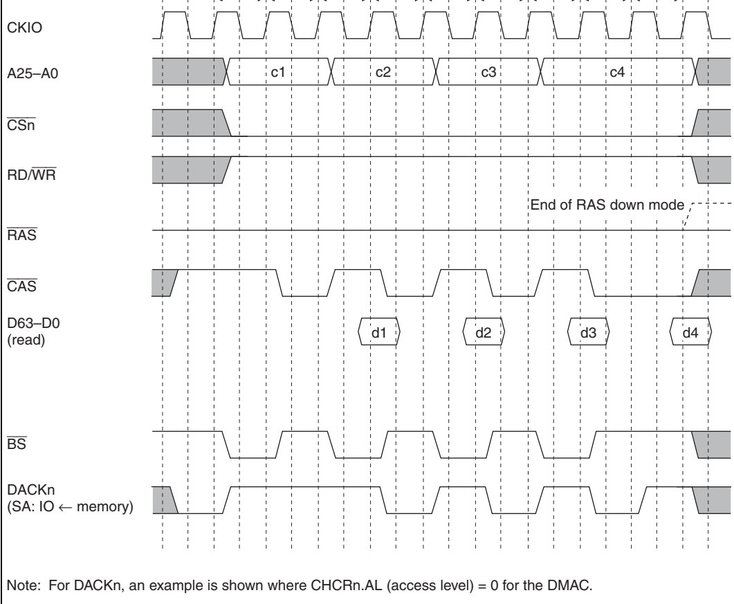
Figure 13.22 (4) DRAM Burst Bus Cycle, RAS Down Mode Continuation (EDO Mode, RCD = 0, AnW = 0)
