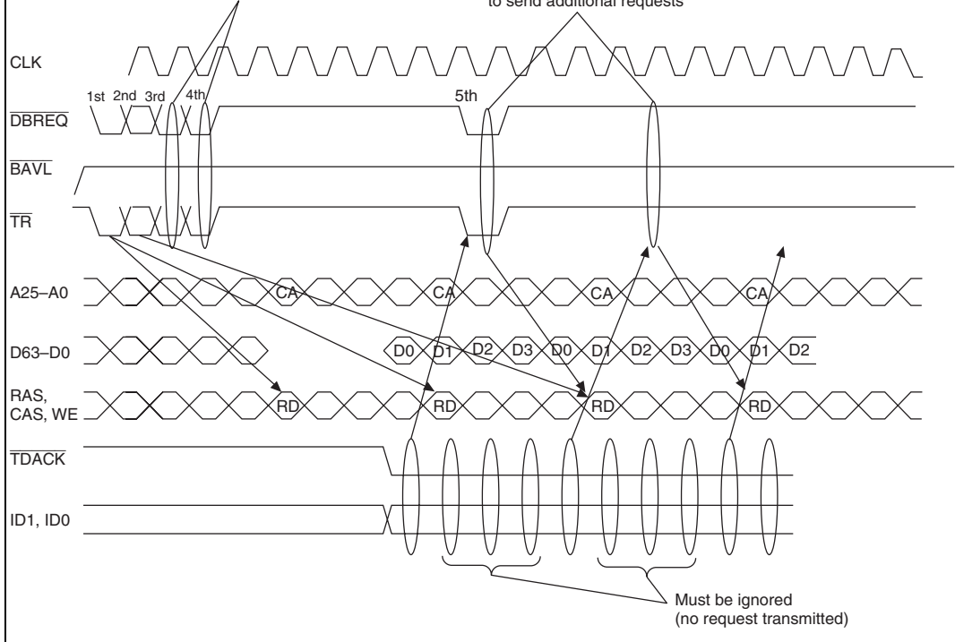
Figure 14.51 Single Address Mode/Burst Mode/External Bus → External Device Data Transfer (Active Bank Address)/Direct Data Transfer Request to Channel 2
