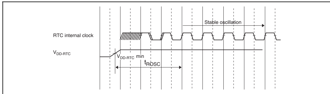
Figure 22.62 RTC Oscillation Settling Time at Power-On
