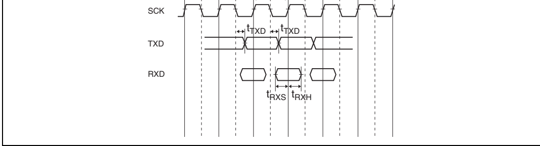
Figure 22.64 SCI I/O Synchronous Mode Clock Timing
