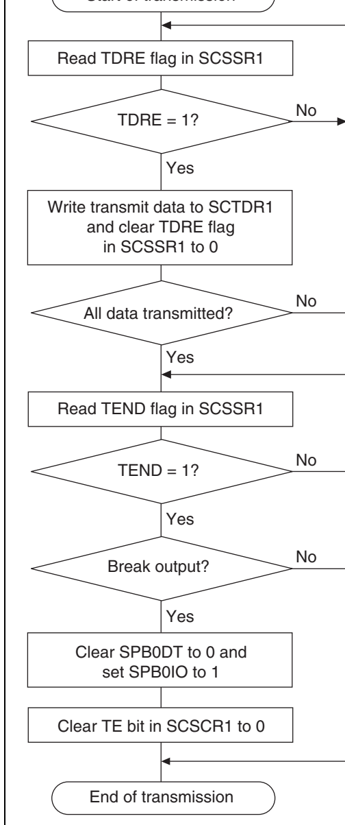
Figure 15.8 Sample Serial Transmission Flowchart
