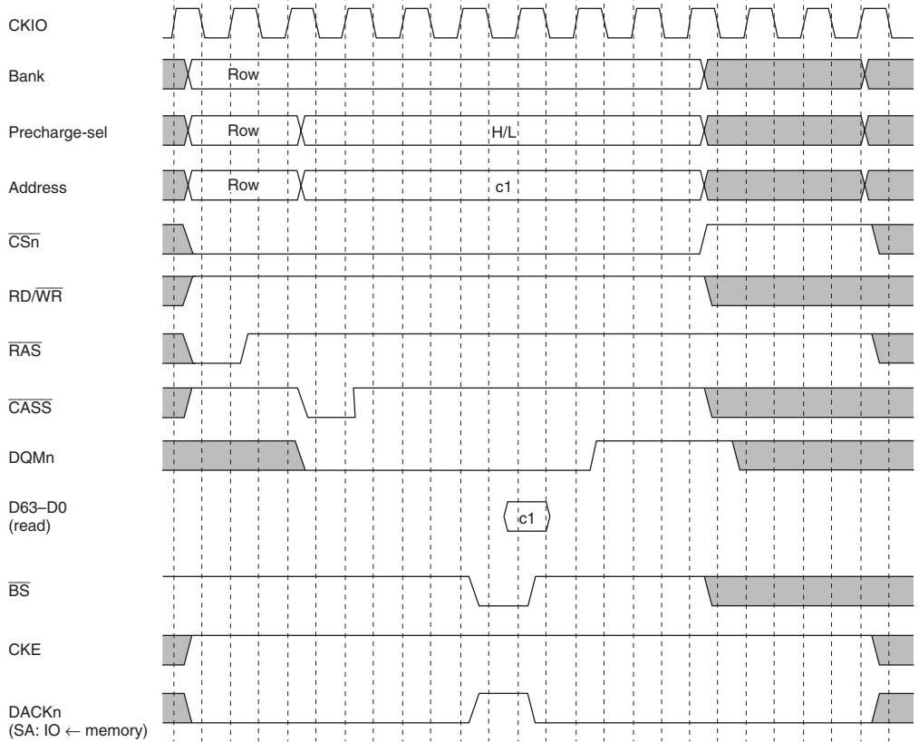
Figure 13.29 Basic Timing for Synchronous DRAM Single Read
