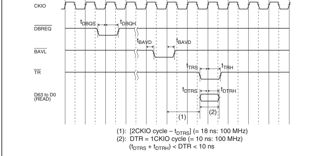
Figure 22.66 (b) \overline{\text{DBREQ}}/\overline{\text{TR}} Input Timing and \overline{\text{BAVL}} Output Timing
