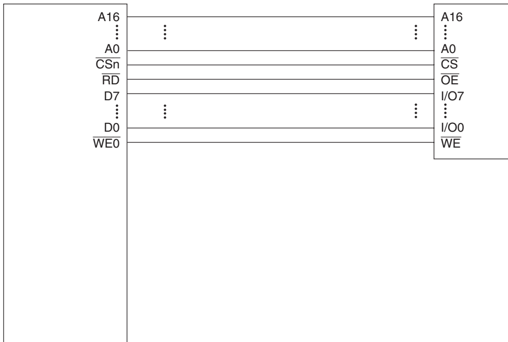
Figure 13.10 Example of 8-Bit Data Width SRAM Connection
