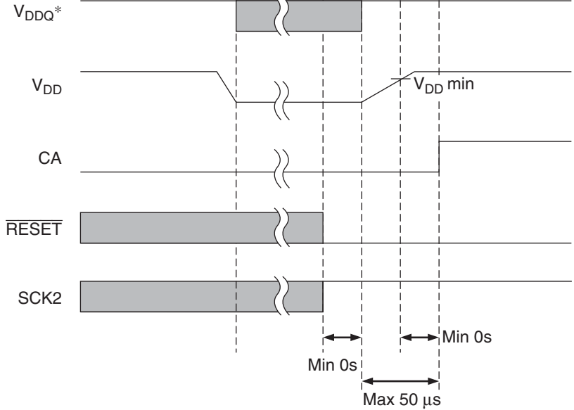
Figure 9.14 Timing When Power Other than VDD-RTC Is Off
