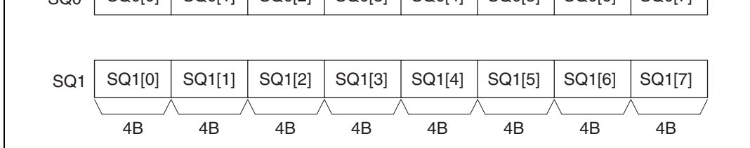
Figure 4.16 Store Queue Configuration
