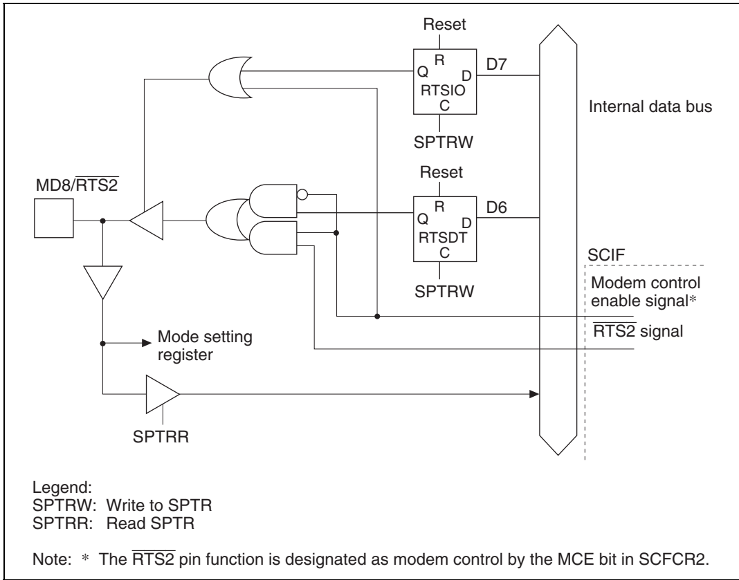
Figure 16.2 MD8/RTS2 Pin
