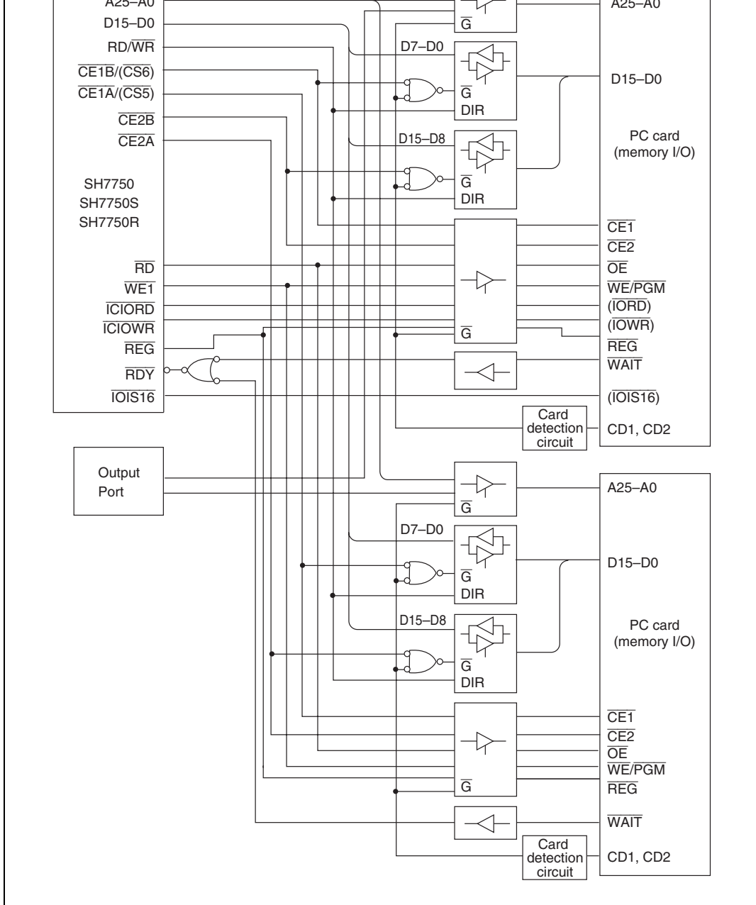
Figure 13.50 Example of PCMCIA Interface
