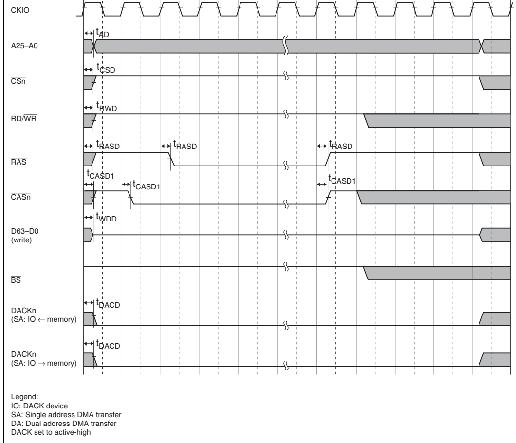
Figure 22.51 DRAM Bus Cycle: DRAM Self-Refresh (TRC[2:0] = 001)
