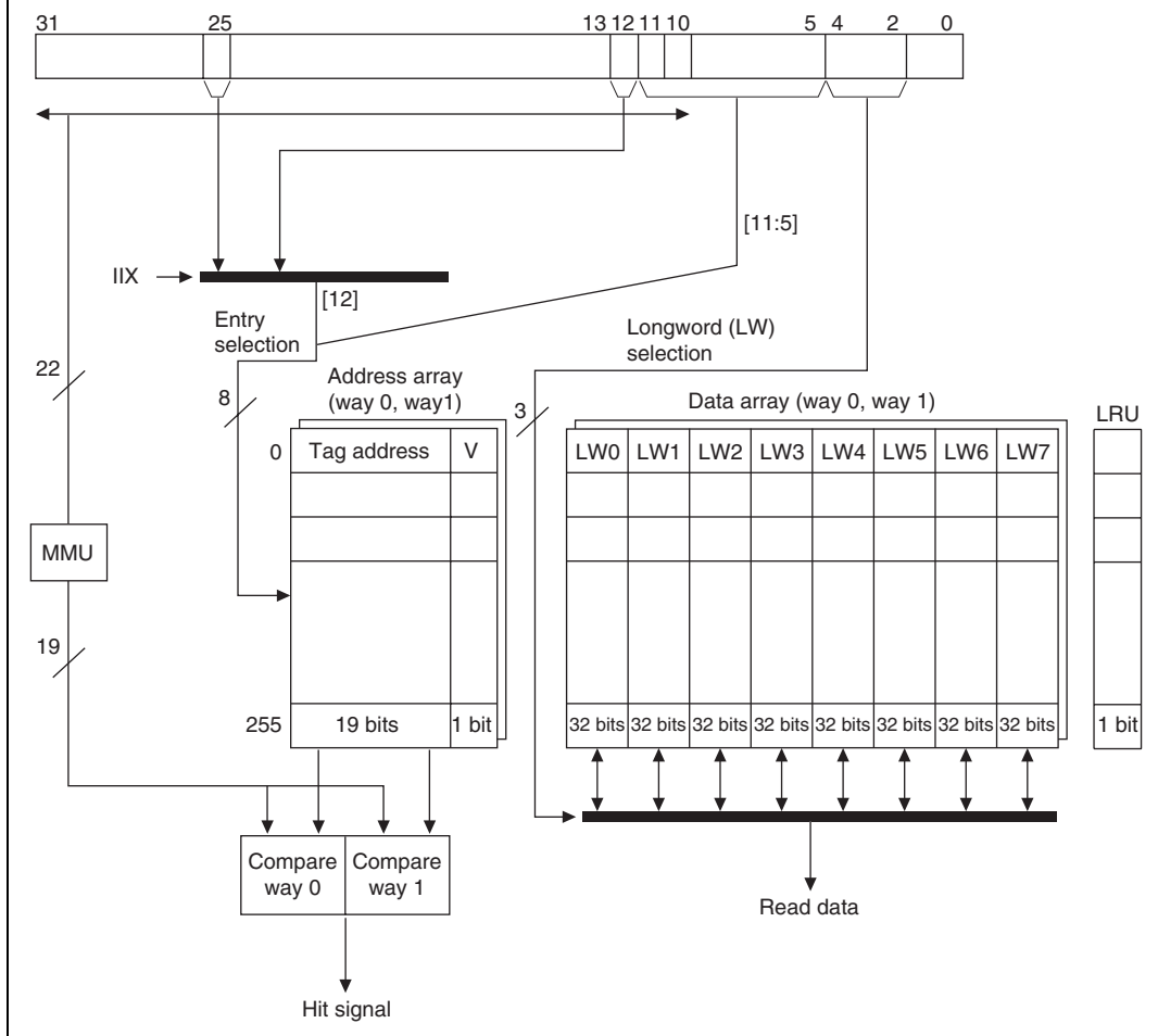
Figure 4.7 Configuration of Instruction Cache (SH7750R)
