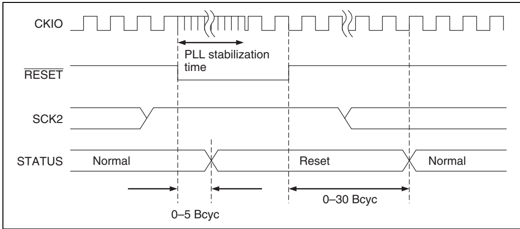
Figure 9.1 STATUS Output in Power-On Reset
