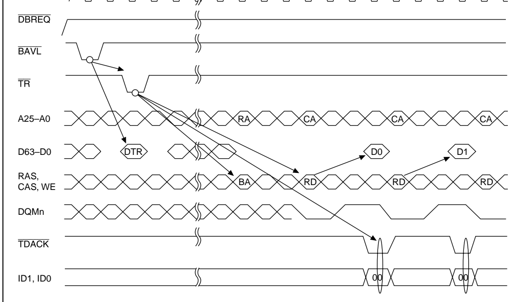
Figure 14.31 Single Address Mode/Burst Mode/External Bus → External Device 32-Bit Transfer/Channel 0 On-Demand Data Transfer
