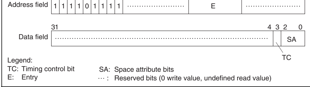
Figure 3.18 Memory-Mapped UTLB Data Array 2
