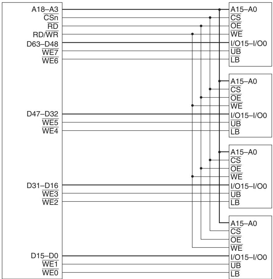
Figure 13.74 Example of 64-Bit Data Width Byte Control SRAM
