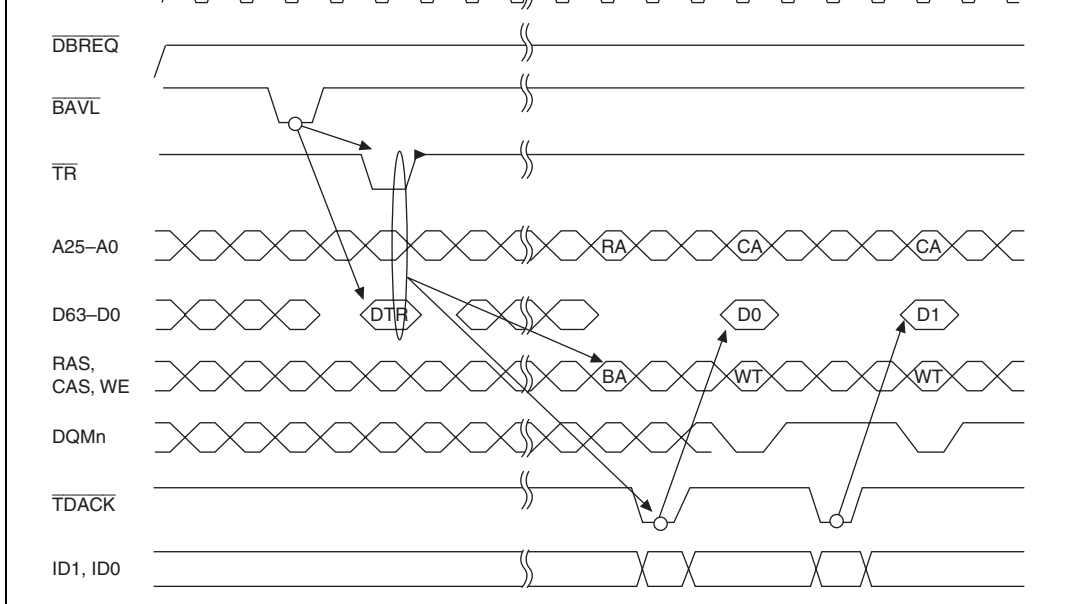
Figure 14.32 Single Address Mode/Burst Mode/External Device → External Bus 32-Bit Transfer/Channel 0 On-Demand Data Transfer
