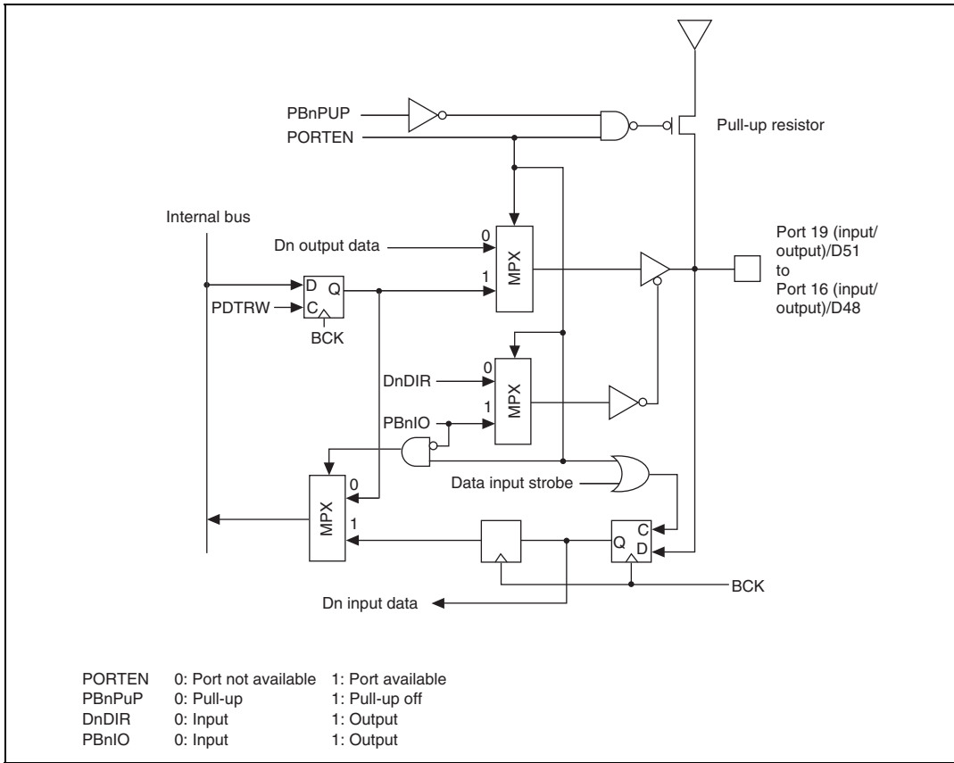
Figure 18.2 4-Bit Port
