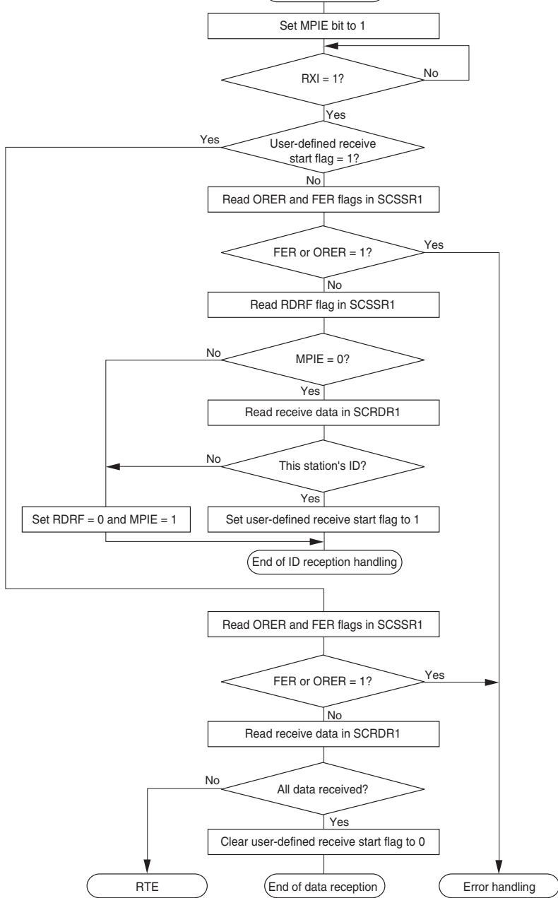
Figure 15.15 Sample Multiprocessor Serial Reception Flowchart (1)
