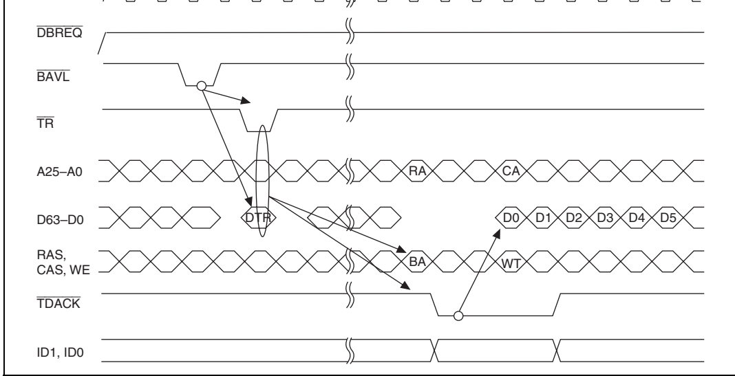
Figure 14.30 Single Address Mode/Burst Mode/External Device → External Bus 32-Byte Block Transfer/Channel 0 On-Demand Data Transfer
