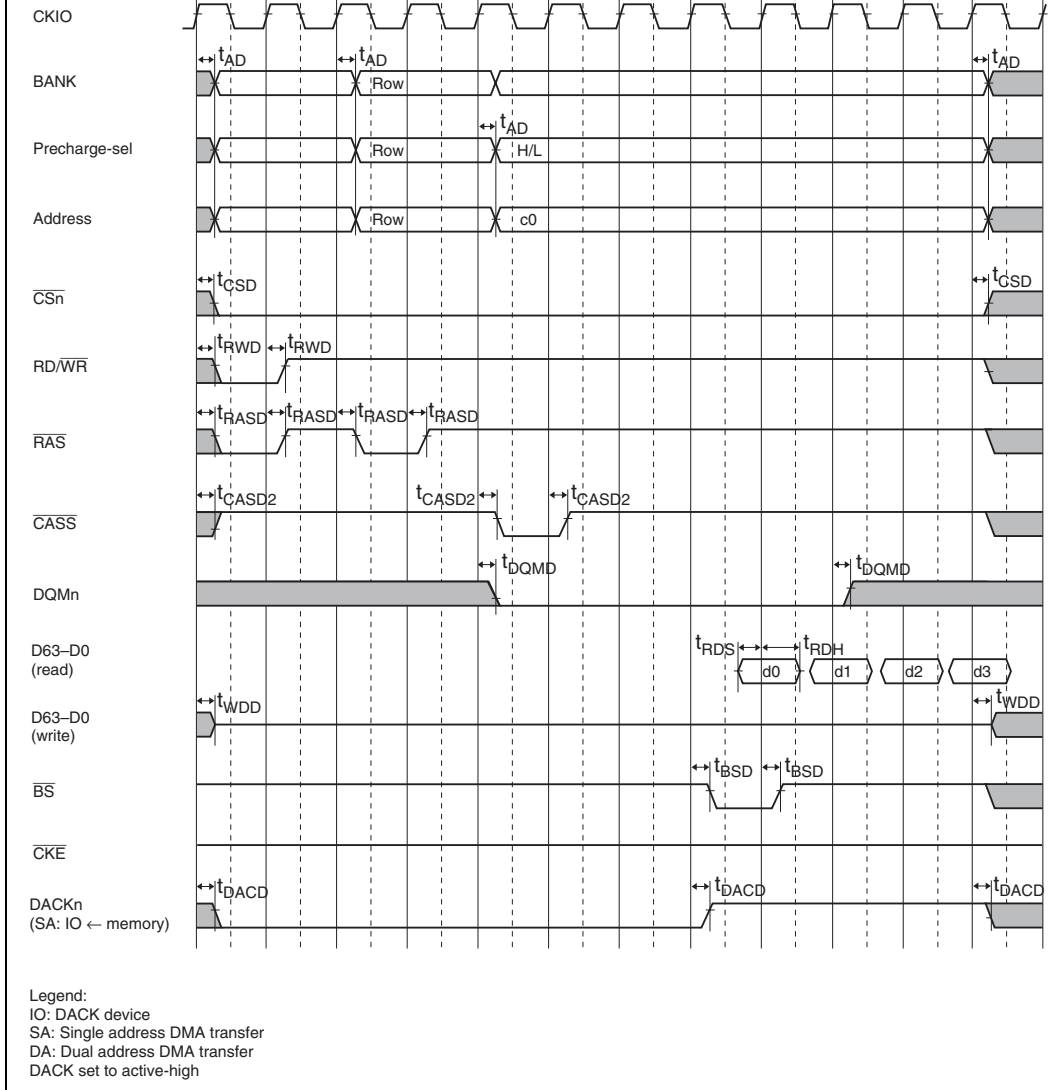
Figure 22.26 Synchronous DRAM Normal Read Bus Cycle: PRE + ACT + READ Commands, Burst ((RASD = 1, RCD[1:0] = 01, TPC[2:0] = 001, CAS Latency = 3)
