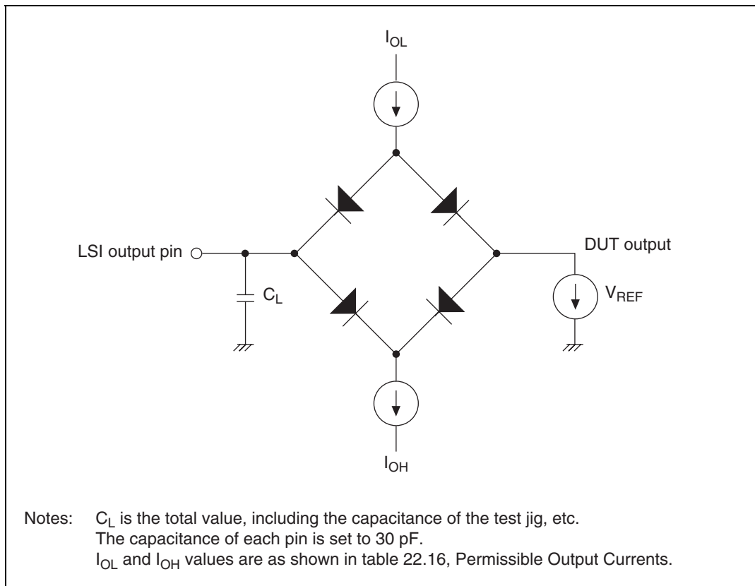
Figure 22.72 Output Load Circuit
