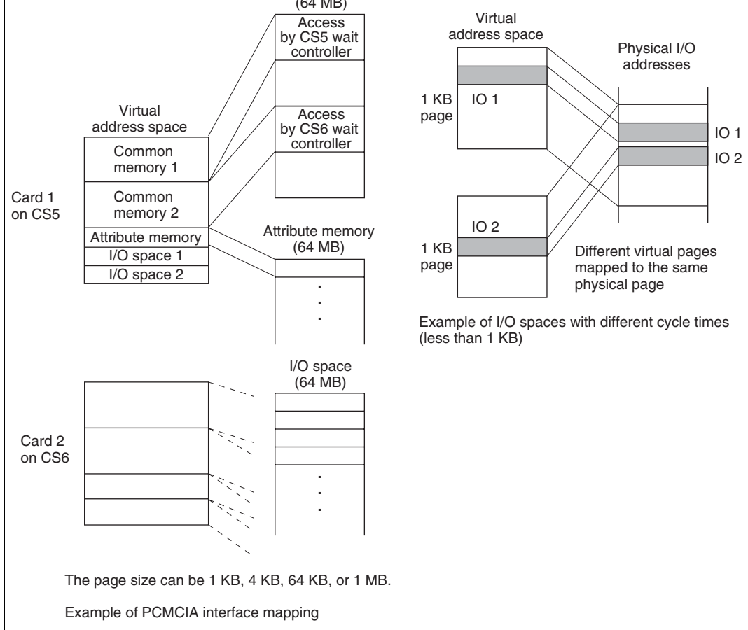
Figure 13.53 PCMCIA Space Allocation
