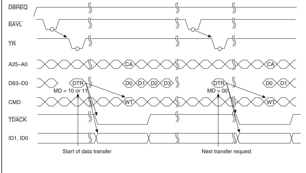
Figure 14.33 Handshake Protocol Using Data Bus (Channel 0 On-Demand Data Transfer)
