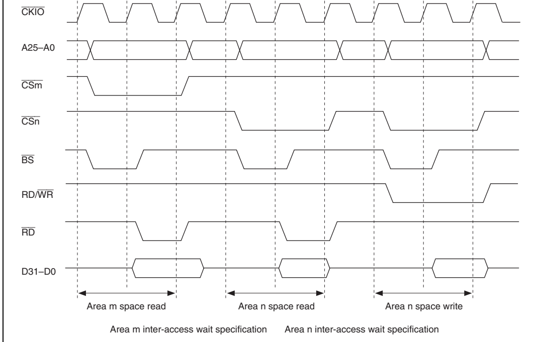
Figure 13.78 Waits between Access Cycles
