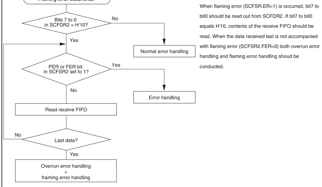
Figure 16.14 Overrun Error Flag
