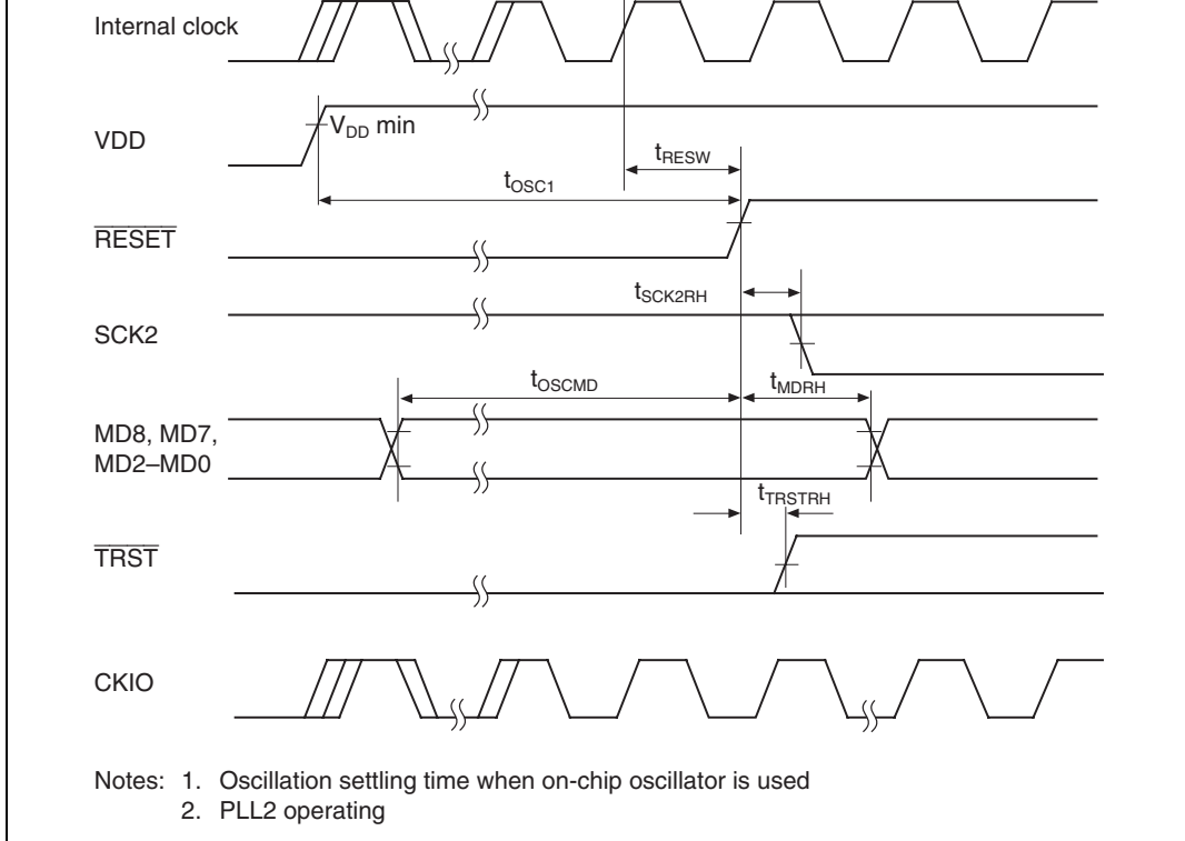
Figure 22.5 Power-On Oscillation Settling Time
