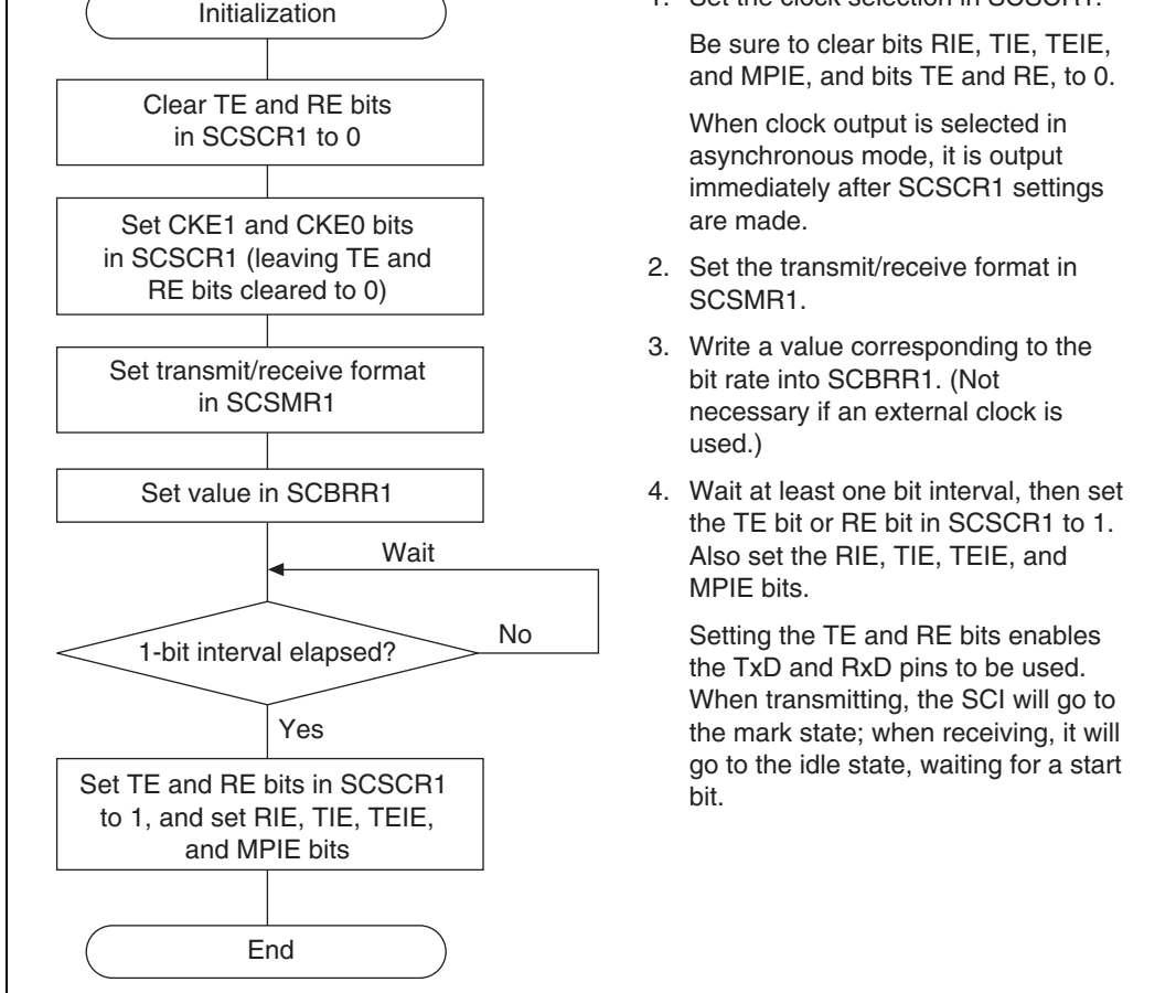
Figure 15.7 Sample SCI Initialization Flowchart
