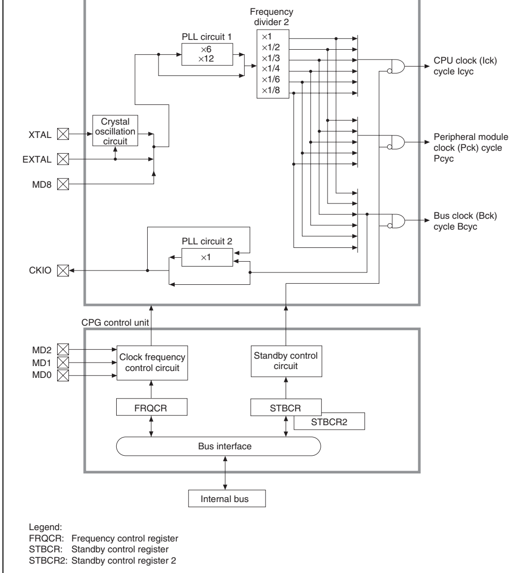
Figure 10.1 (2) Block Diagram of CPG (SH7750R)
