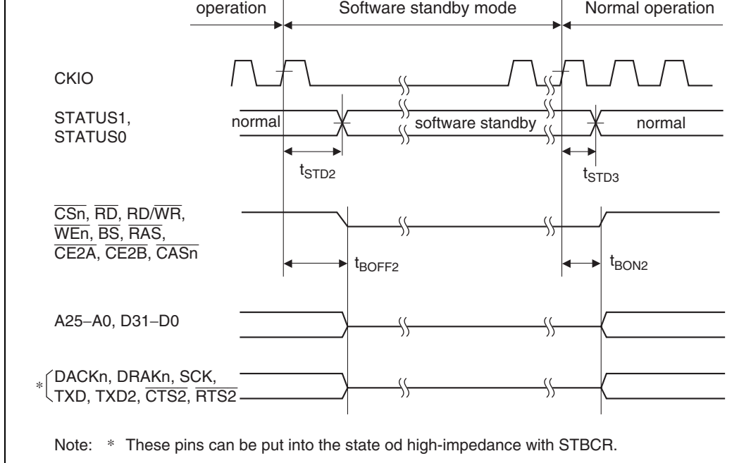
Figure 22.14 (2) Pin Drive Timing for Software Standby Mode
