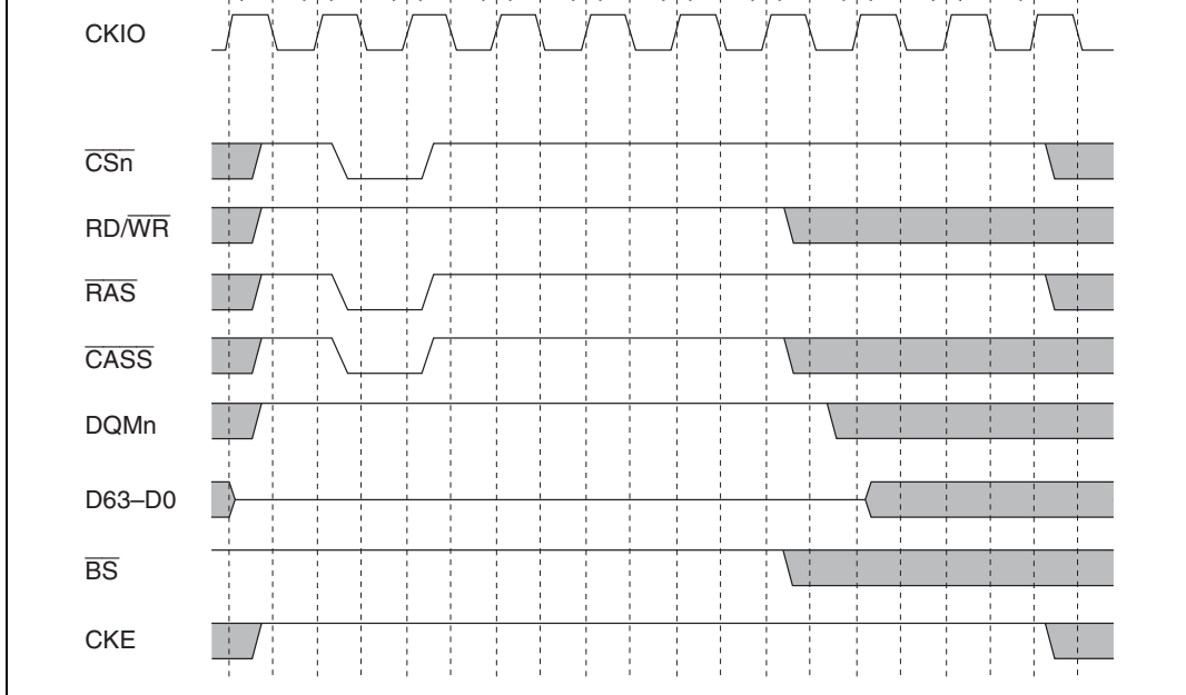
Figure 13.40 Synchronous DRAM Auto-Refresh Timing
