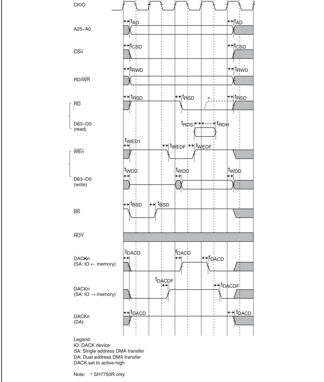
Figure 22.18 SRAM Bus Cycle: Basic Bus Cycle (No Wait, Address Setup/Hold Time Insertion, AnS = 1, AnH = 1)
