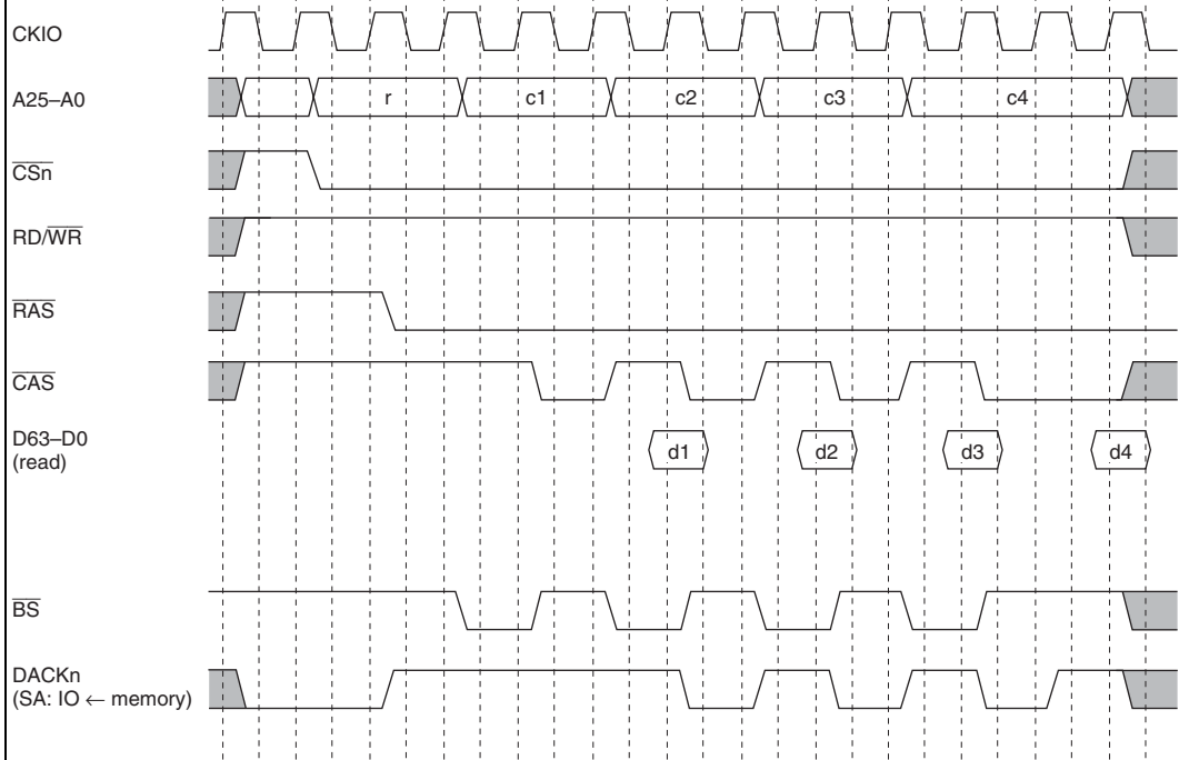
Figure 13.22 (3) DRAM Burst Bus Cycle, RAS Down Mode Start (EDO Mode, RCD = 0, AnW = 0)
