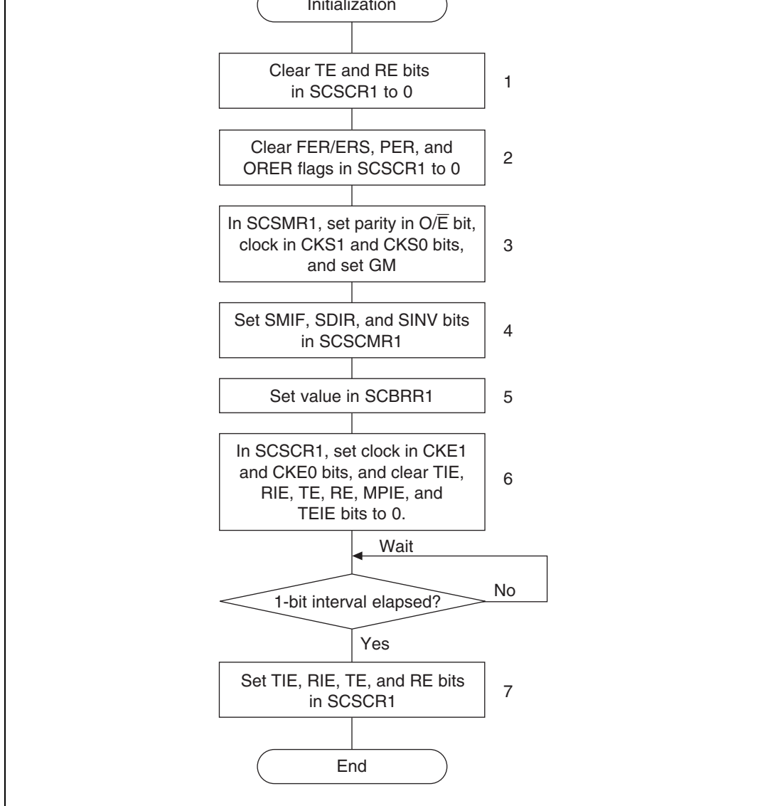
Figure 17.7 Sample Initialization Flowchart
