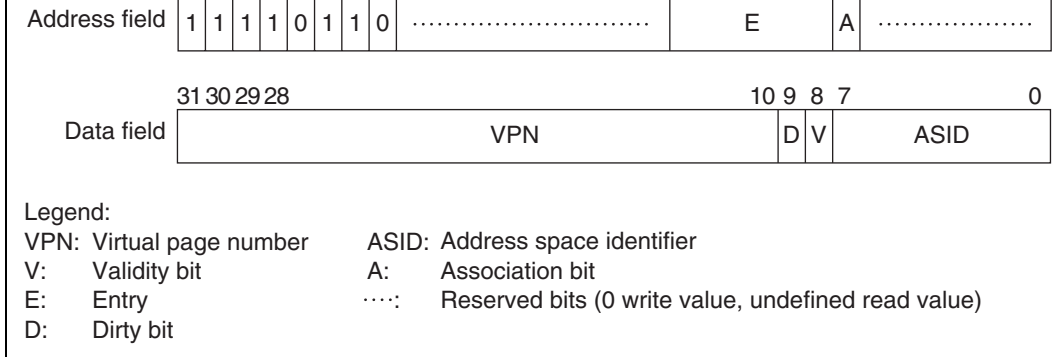
Figure 3.16 Memory-Mapped UTLB Address Array
