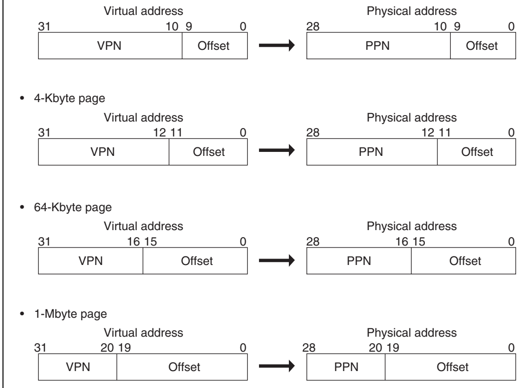
Figure 3.8 Relationship between Page Size and Address Format
