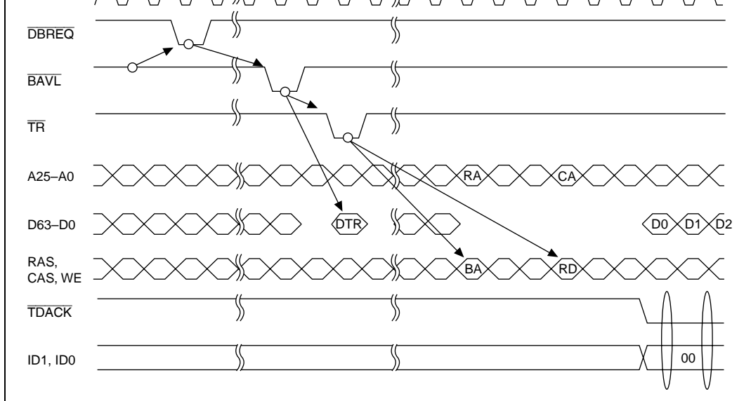
Figure 14.41 Single Address Mode/Burst Mode/External Bus → External Device 32-Byte Block Transfer/Channel 0 On-Demand Data Transfer
