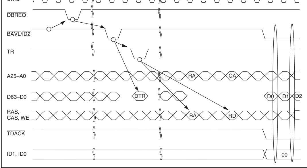
Figure 14.56 Single Address Mode/Burst Mode/External Bus → External Device/32-Byte Block Transfer/On-Demand Data Transfer on Channel 4
