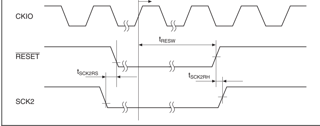
Figure 22.11 Manual Reset Input Timing
