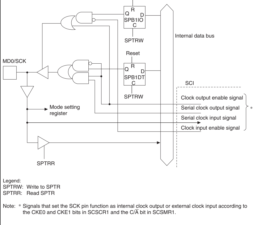
Figure 15.2 MD0/SCK Pin
