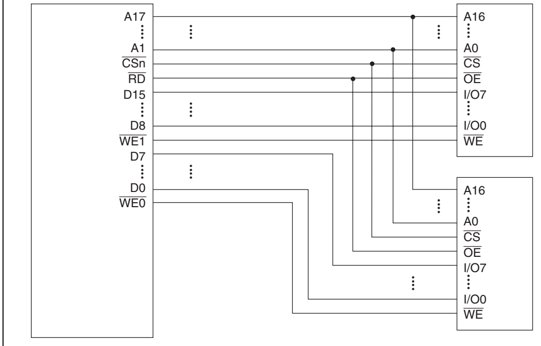
Figure 13.9 Example of 16-Bit Data Width SRAM Connection
