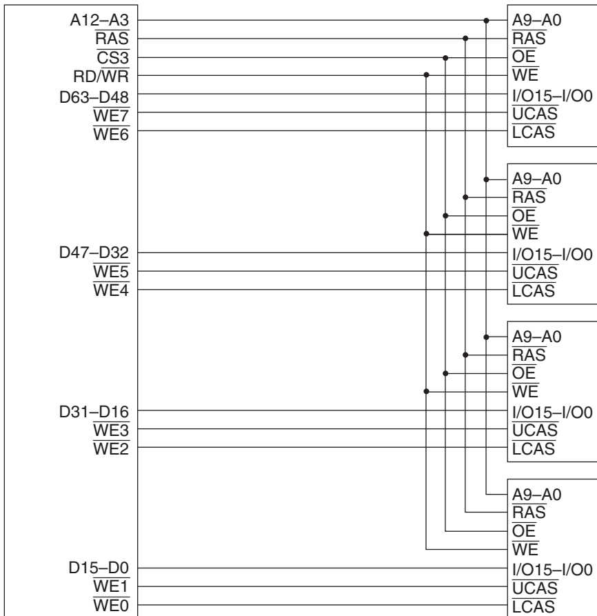
Figure 13.14 Example of DRAM Connection (64-Bit Data Width, Area 3)
