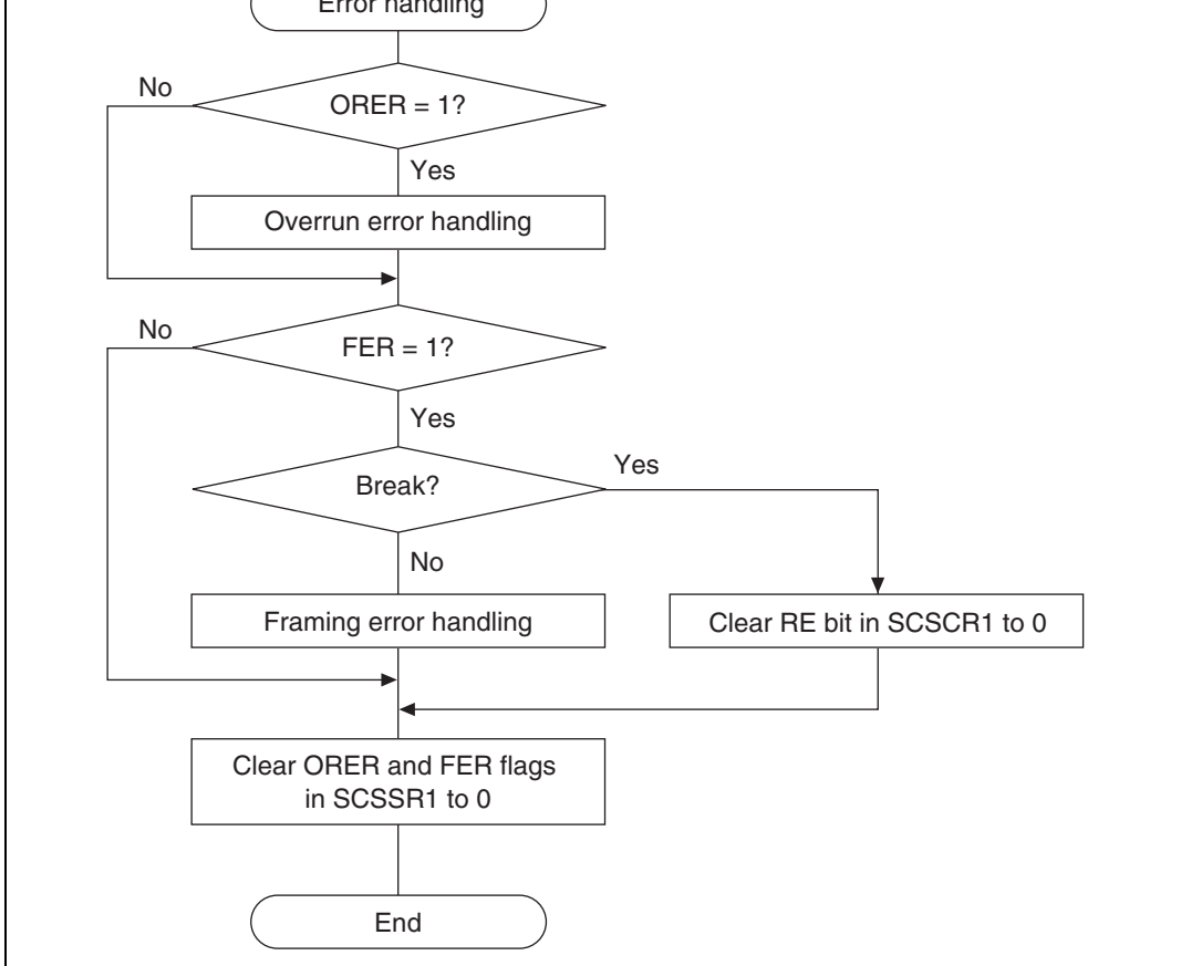
Figure 15.15 Sample Multiprocessor Serial Reception Flowchart (2)
