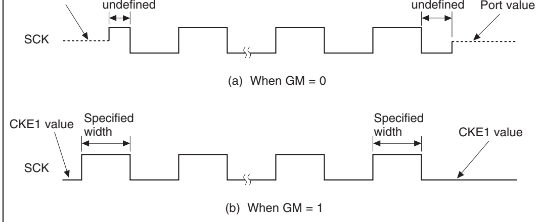
Figure 17.6 Difference in Clock Output According to GM Bit Setting
