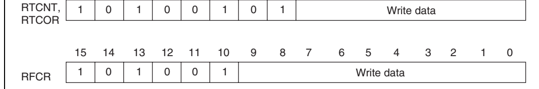
Figure 13.5 Writing to RTCSR, RTCNT, RTCOR, and RFCR
