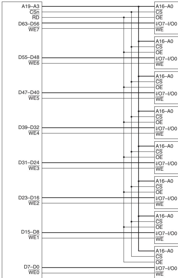
Figure 13.7 Example of 64-Bit Data Width SRAM Connection
