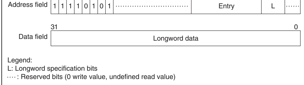
Figure 4.11 Memory-Mapped OC Data Array
