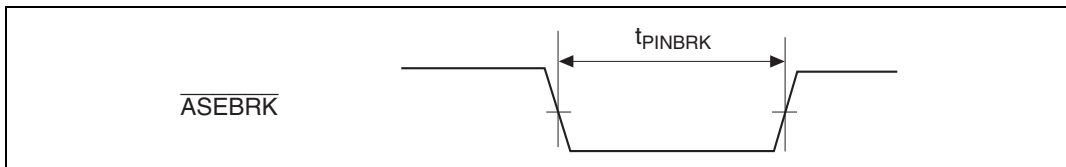
Figure 22.70 Pin Break Timing
