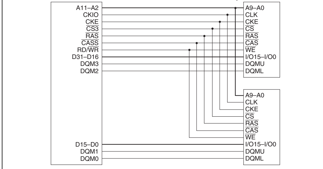
Figure 13.27 Example of 32-Bit Data Width Synchronous DRAM Connection (Area 3)
