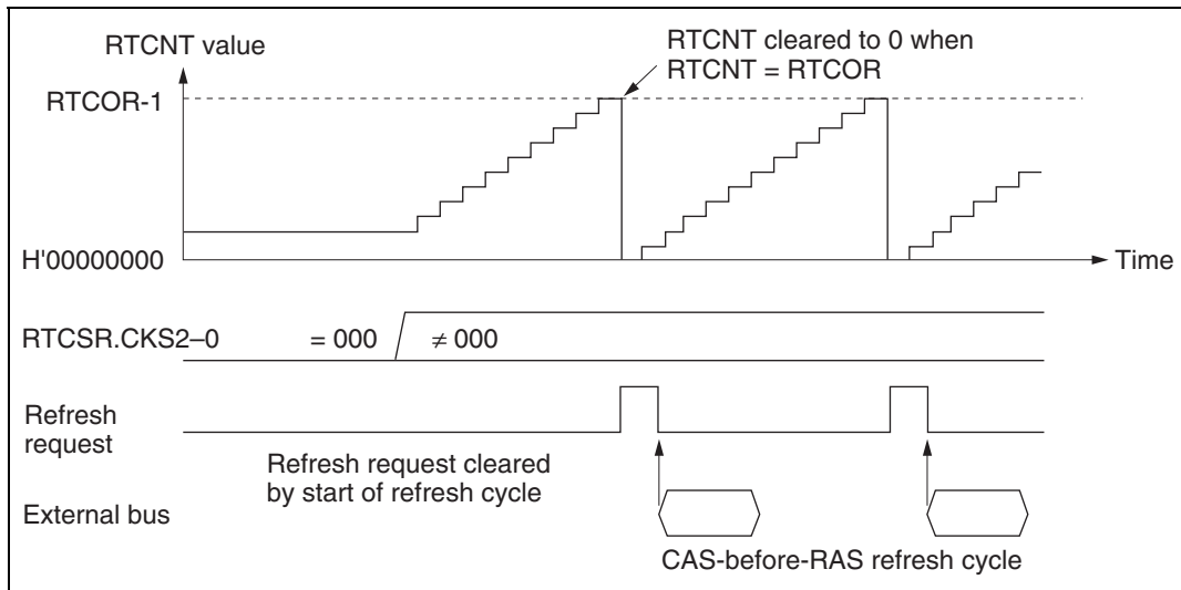
Figure 13.23 CAS-Before-RAS Refresh Operation
