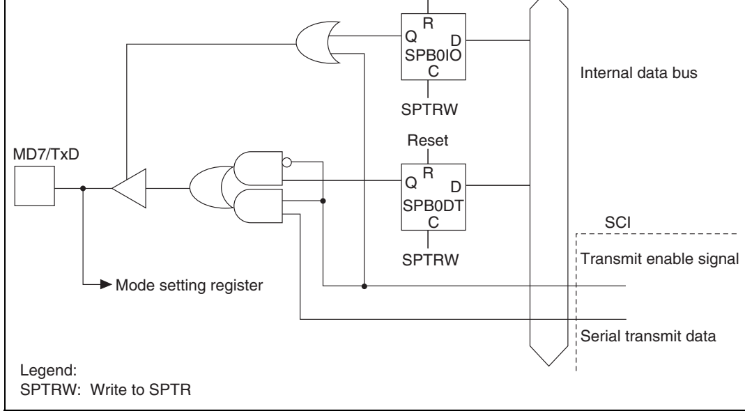
Figure 18.4 MD7/TxD Pin
