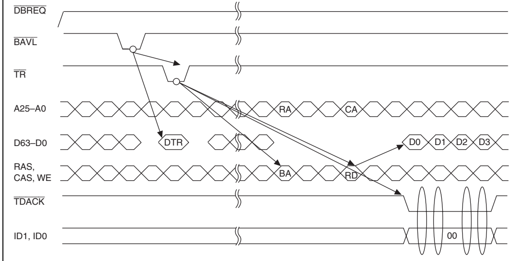
Figure 14.29 Single Address Mode/Burst Mode/External Bus → External Device 32-Byte Block Transfer/Channel 0 On-Demand Data Transfer
