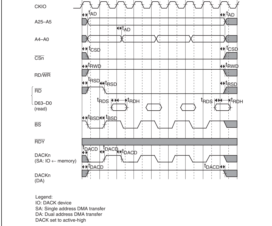
Figure 22.19 Burst ROM Bus Cycle (No Wait)
