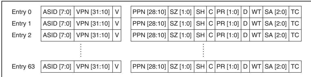
Figure 3.7 UTLB Configuration
