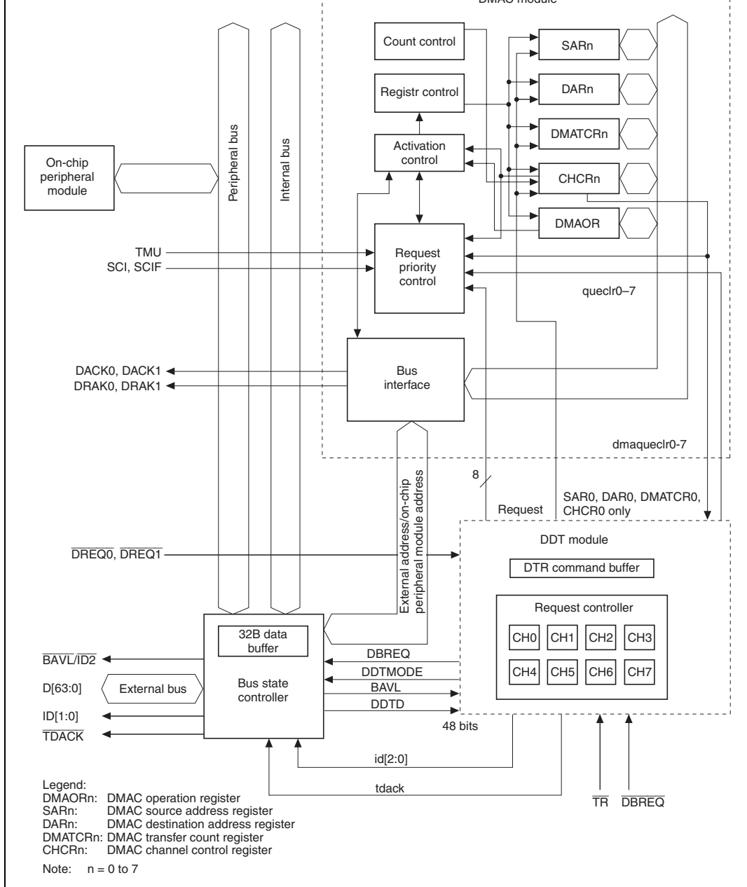
Figure 14.53 Block Diagram of the DMAC
