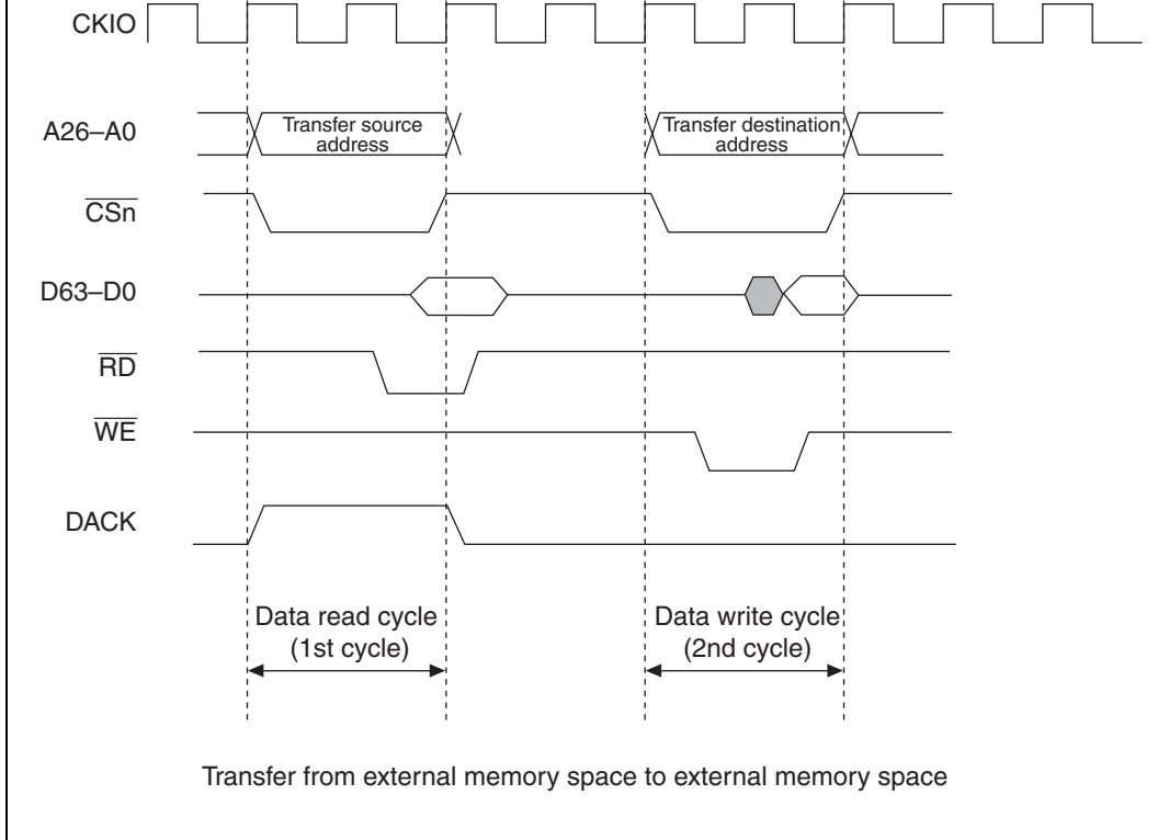
Figure 14.8 Example of Transfer Timing in Dual Address Mode
