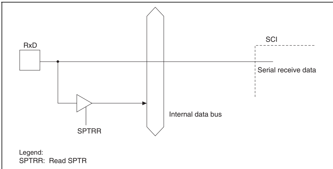
Figure 15.4 RxD Pin
