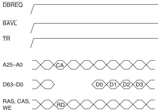
Figure 14.37 Read from Synchronous DRAM (Row Hit)
