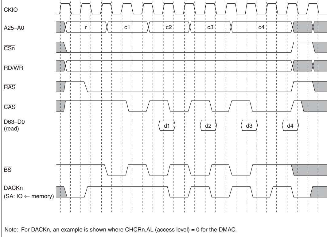
Figure 13.21 Burst Access Timing in DRAM EDO Mode
