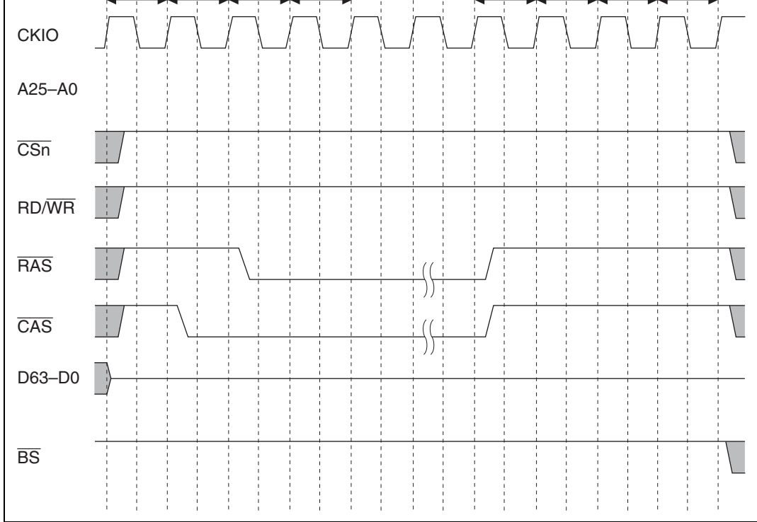
Figure 13.25 DRAM Self-Refresh Cycle Timing
