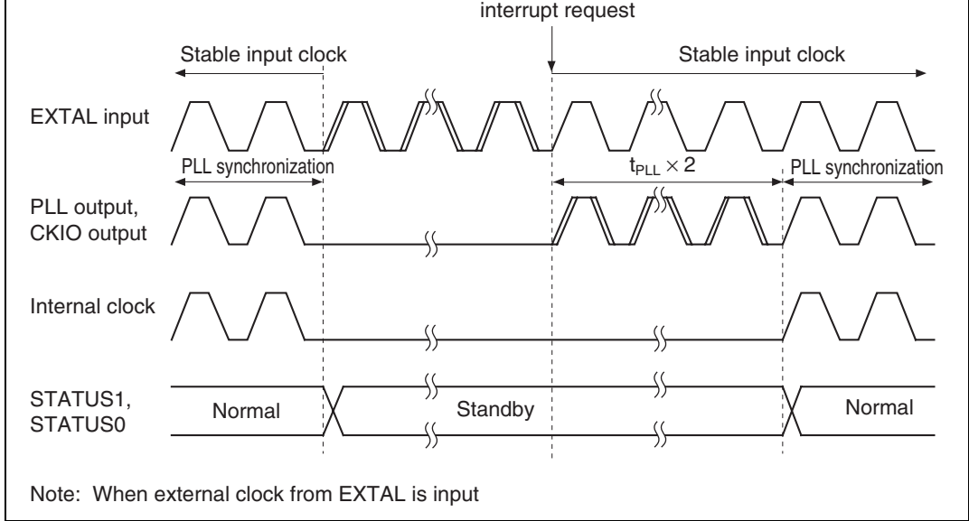
Figure 22.9 PLL Synchronization Settling Time in Case of \overline{\text{RESET}} or NMI Interrupt
