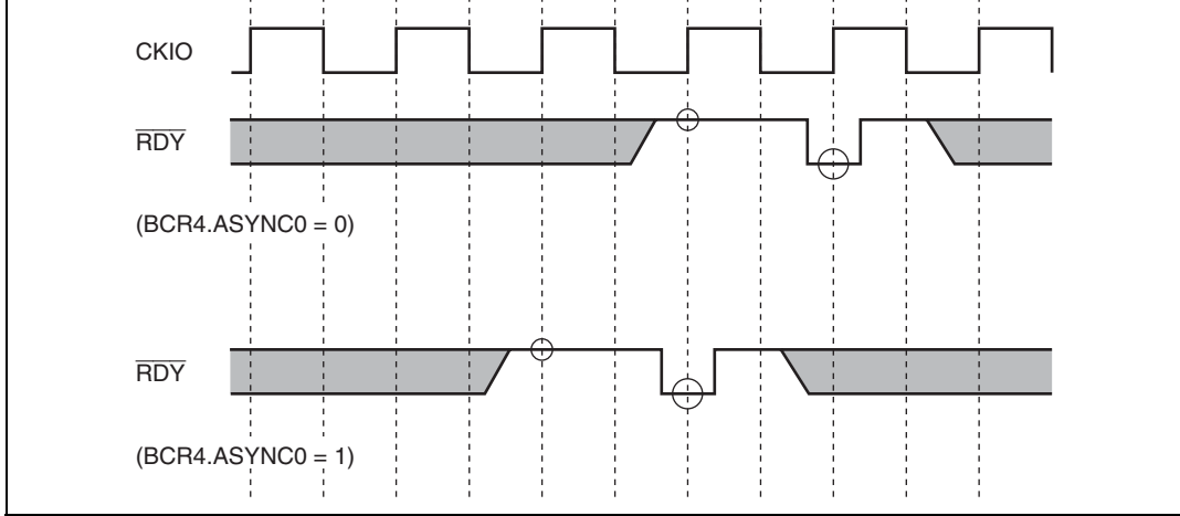
Figure 13.4 Example of \overline{\text{RDY}} Sampling Timing at which BCR4 Is Set (Two Wait Cycles Are Inserted by WCR2)
