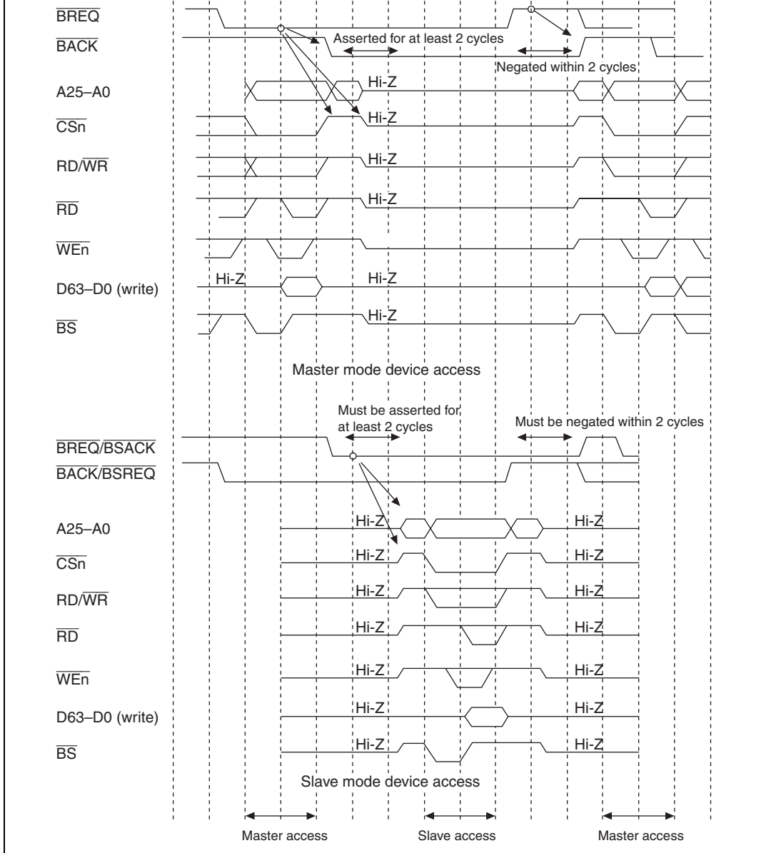
Figure 13.79 Arbitration Sequence
