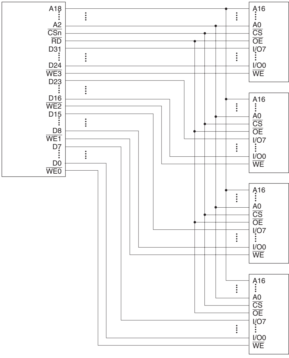
Figure 13.8 Example of 32-Bit Data Width SRAM Connection
