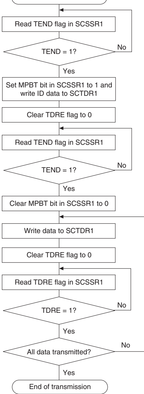
Figure 15.13 Sample Multiprocessor Serial Transmission Flowchart
