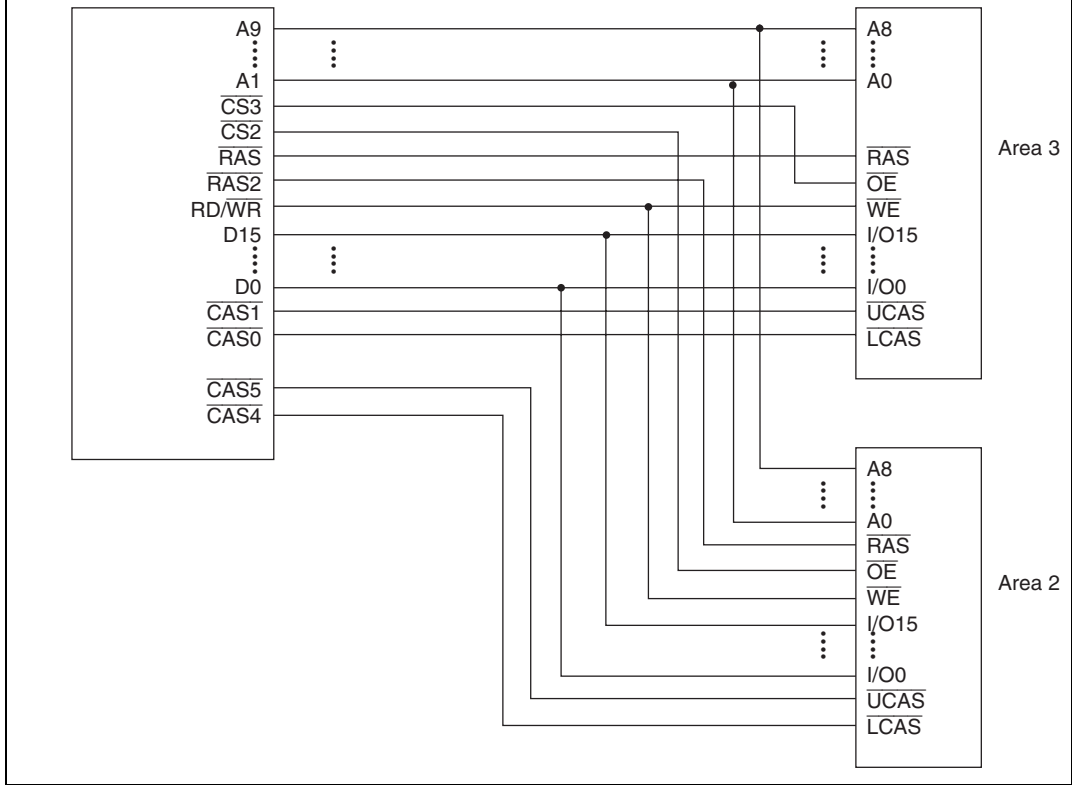
Figure 13.16 Example of DRAM Connection (16-Bit Data Width, Areas 2 and 3)
