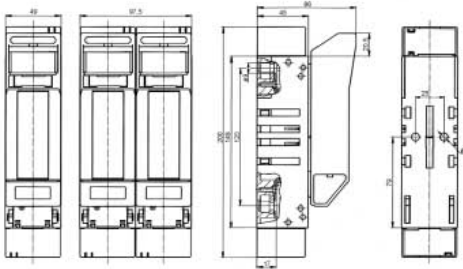
LBS00 1 Pole and 2 Pole
