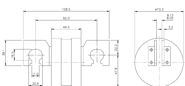
Dimensions for SJ31-6
