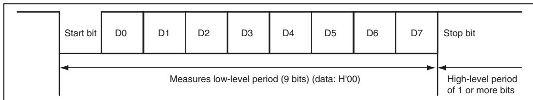
Figure 7.3 Automatic Adjustment of Bit Rates
