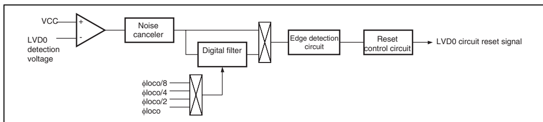
Figure 26.4 Block Diagram of LVD0 Reset Generation Circuit
