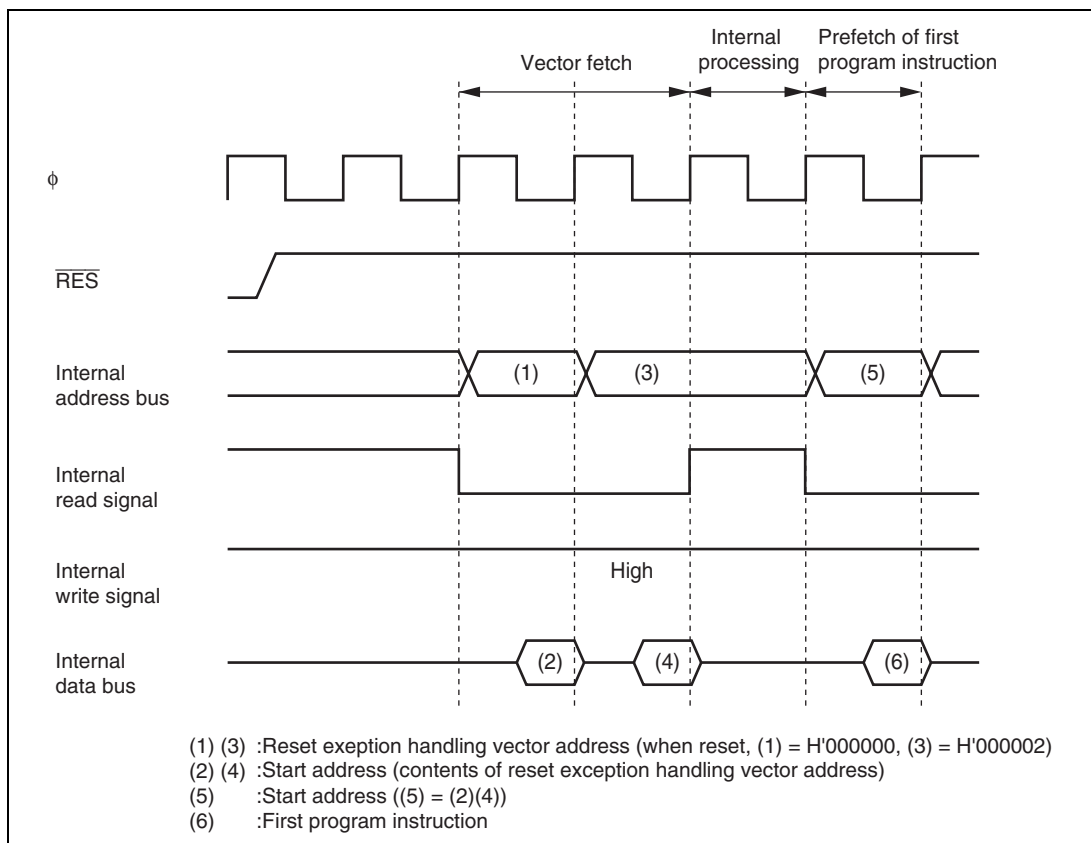
Figure 3.1 Reset Sequence
