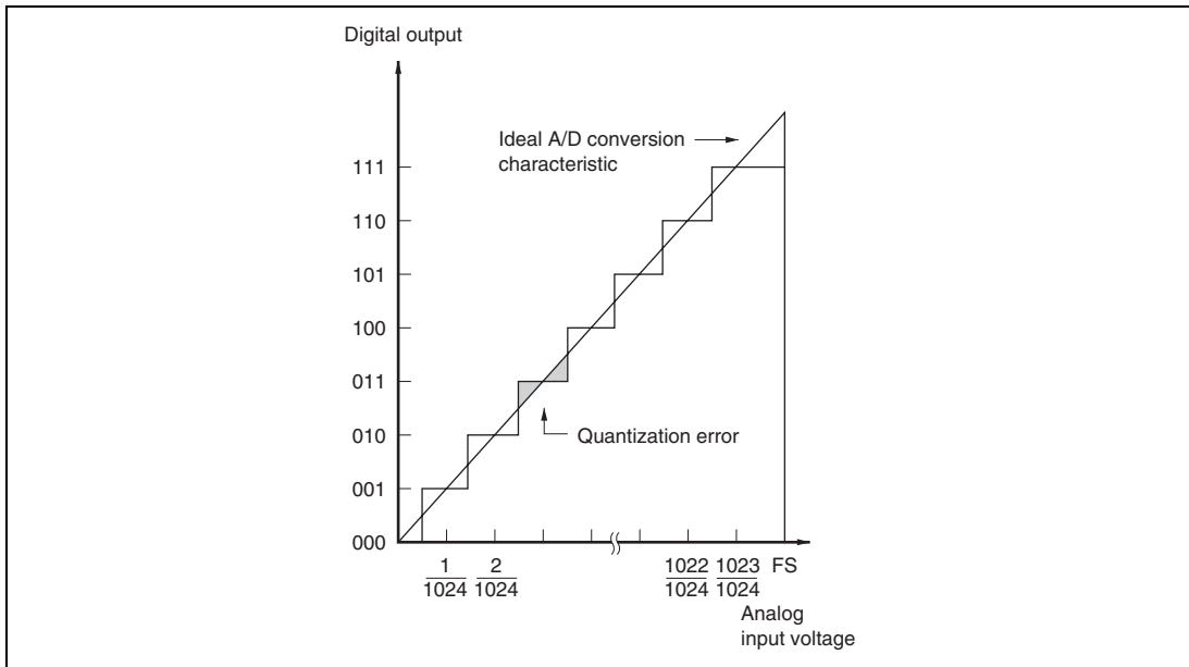
Figure 24.9 A/D Conversion Accuracy Definitions
