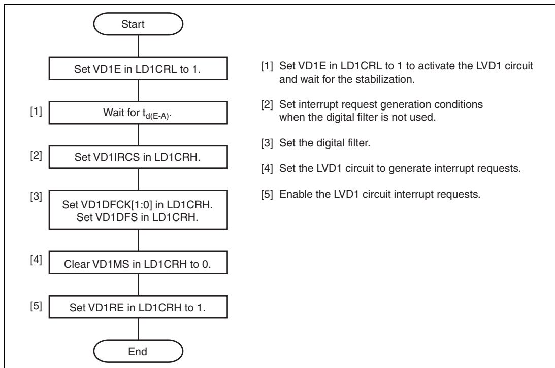
Figure 26.13 Procedure to Set LVDI1
