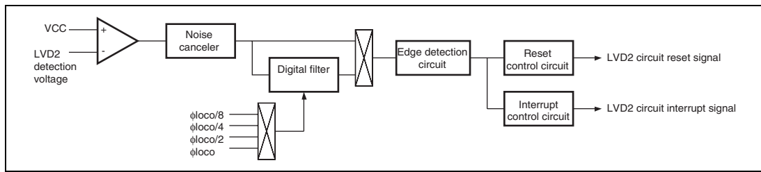
Figure 26.2 Block Diagram of LVD2 Interrupt/Reset Generation Circuit
