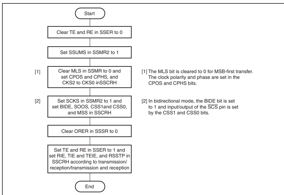
Figure 22.10 Initialization in Four-Line Bus Communication Mode
