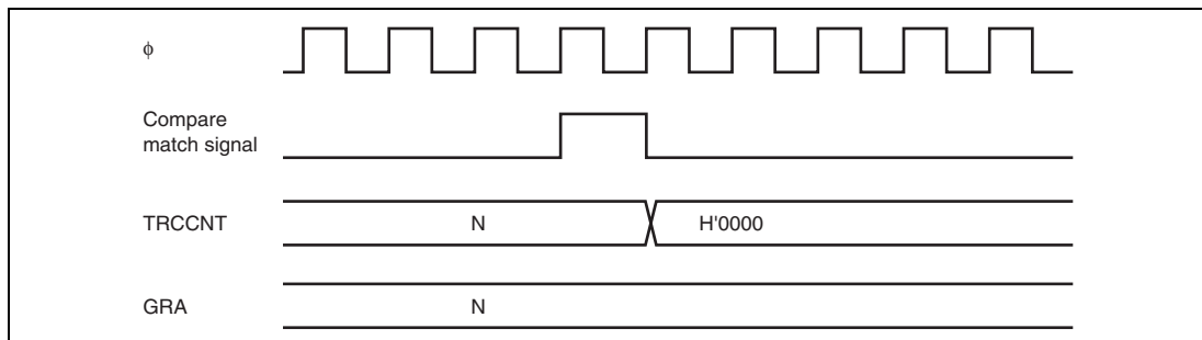
Figure 15.30 Timing of Counter Clearing by Compare Match
