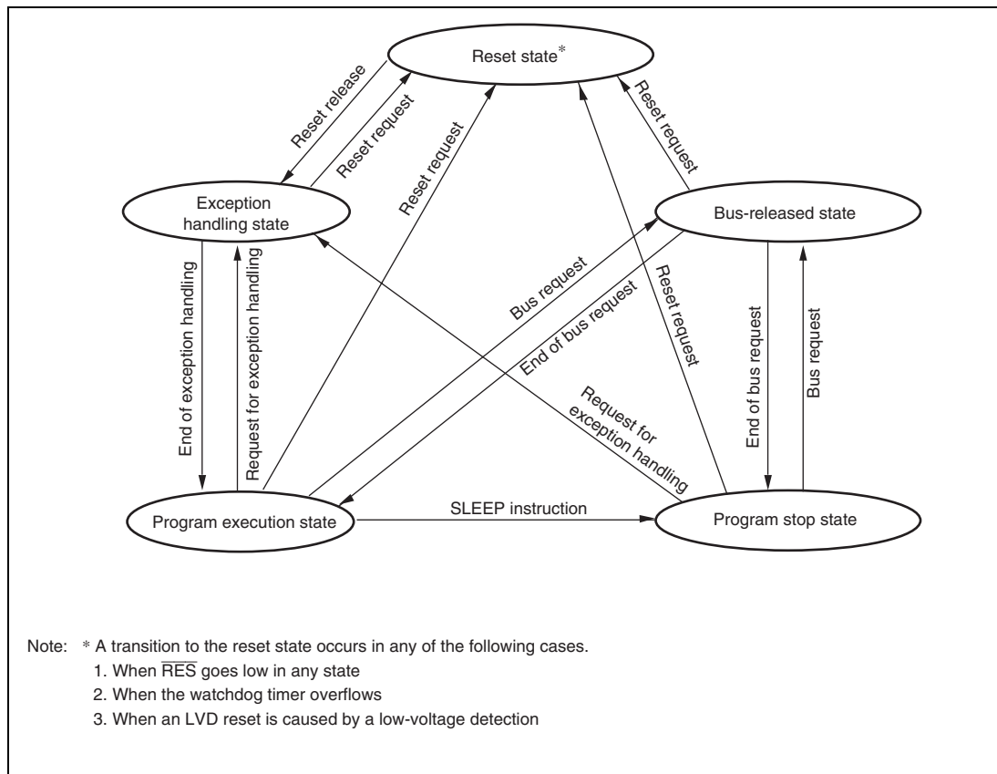
Figure 2.11 State Transitions
