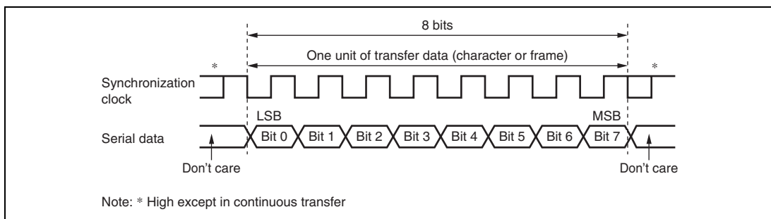
Figure 20.9 Data Format in Clocked Synchronous Communication
