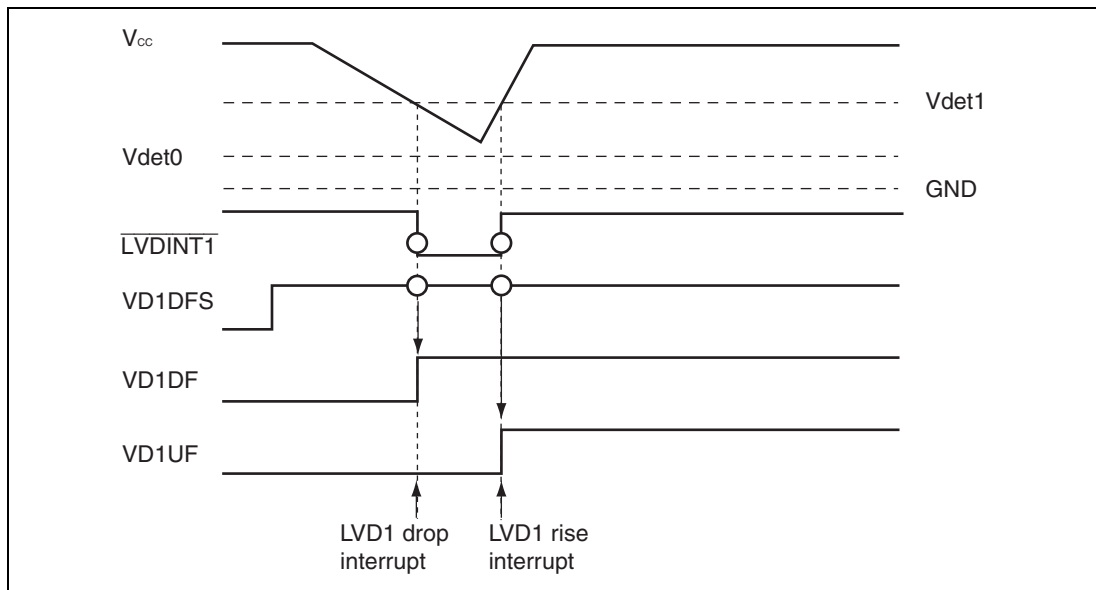
Figure 26.12 Operational Timing of LVDI1
