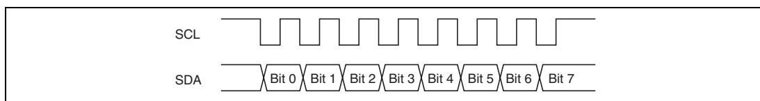
Figure 21.13 Clock Synchronous Serial Transfer Format
