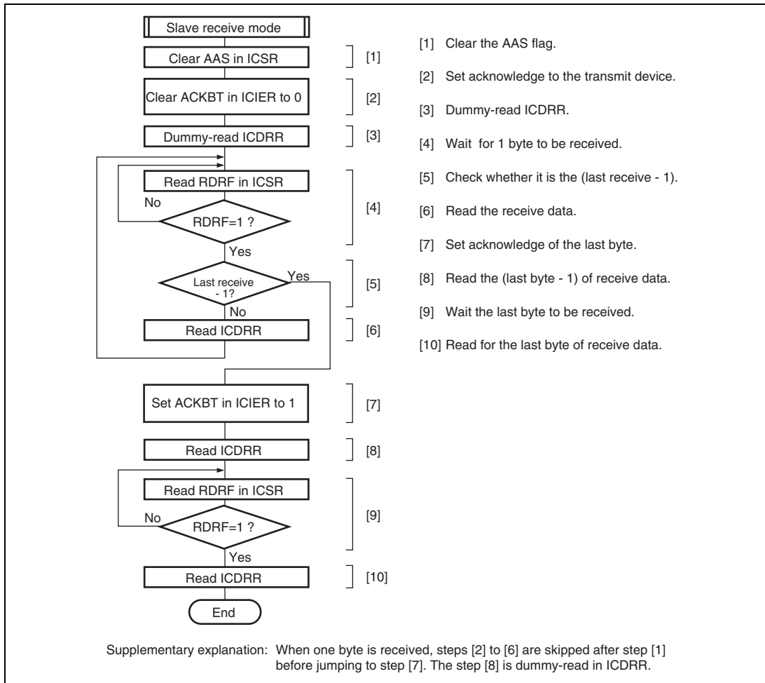
Figure 21.20 Sample Flowchart for Slave Receive Mode
