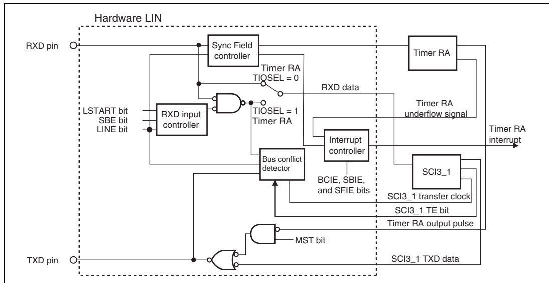
Figure 23.1 Block Diagram of Hardware LIN
