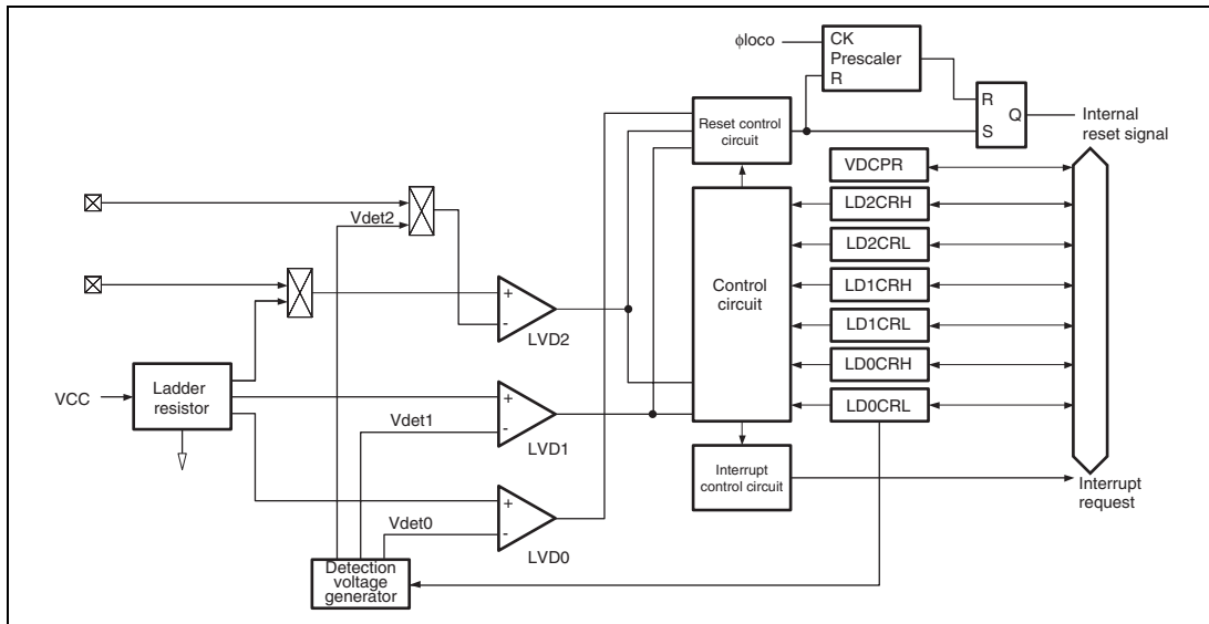
Figure 26.1 Block Diagram of Low-Voltage Detection Circuits
