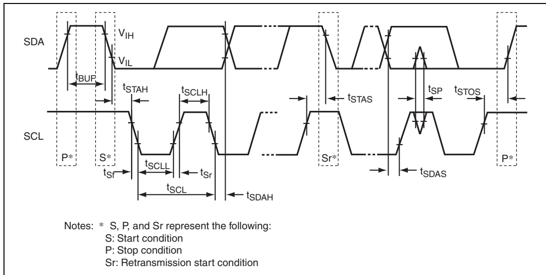
Figure 28.5 I 2 C Bus Interface Input/Output Timing
