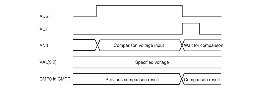
Figure 24.5 A/D Converter Operation in Compare Mode (When Channel 0 Is Selected in Single Mode)
