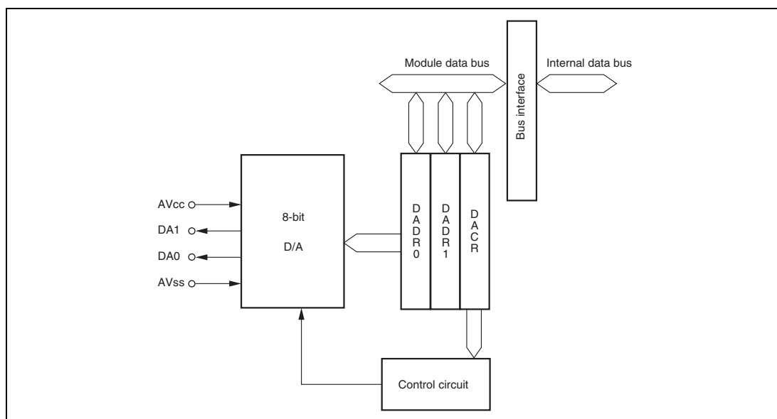
Figure 25.1 Block Diagram of D/A Converter
