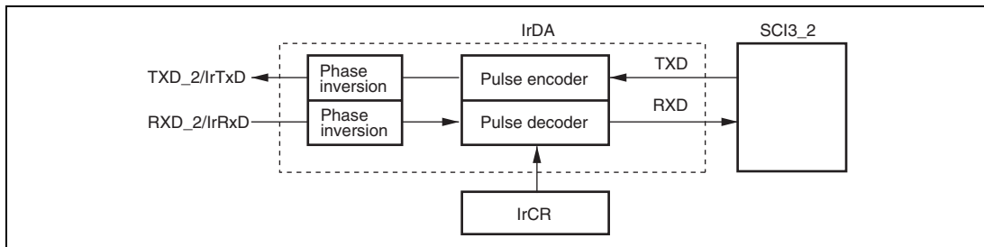
Figure 20.19 IrDA Block Diagram
