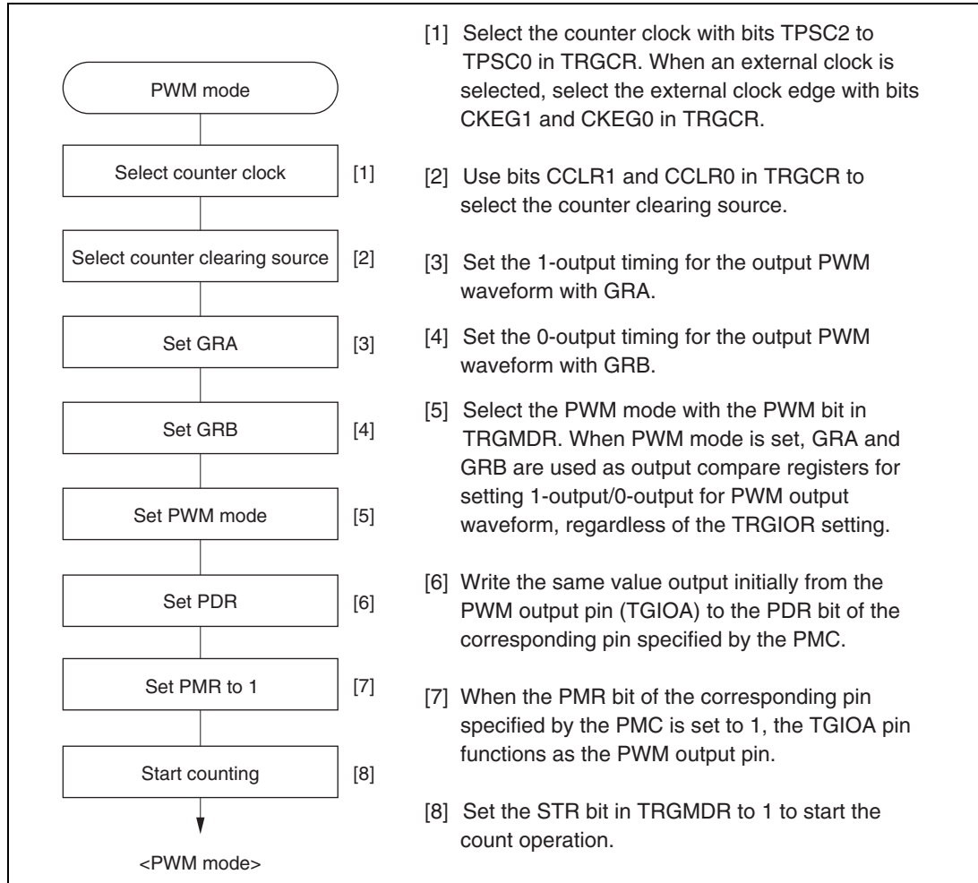
Figure 18.9 Example of PWM Mode Setting Procedure
