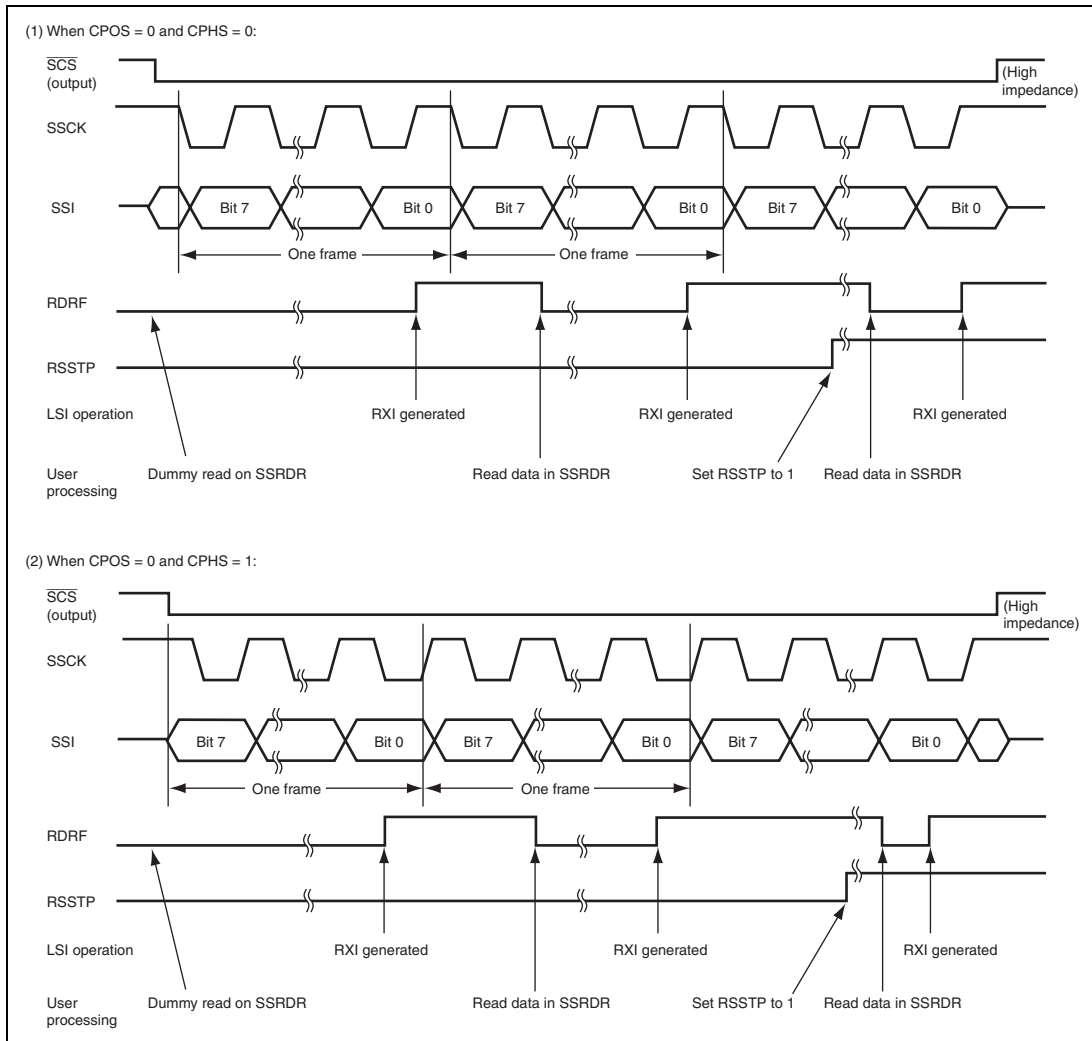
Figure 22.12 Example of Operation in Data Reception (MSS = 1)
