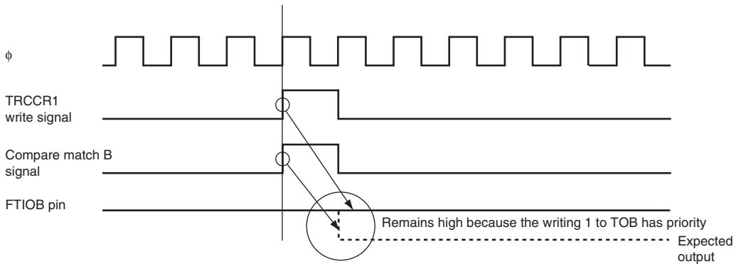
Figure 15.39 When Compare Match and Bit Manipulation Instruction to TRCCR1 Occur at the Same Timing
