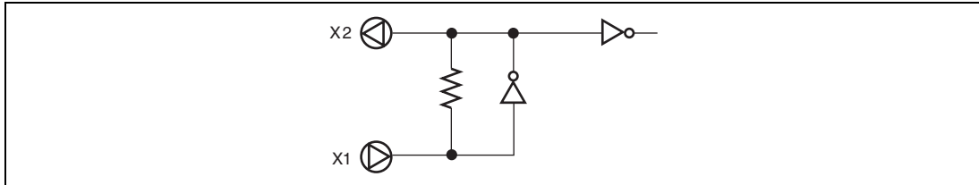
Figure 5.16 Block Diagram of Subclock Oscillator
