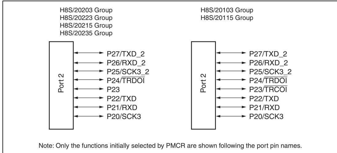
Figure 10.2 Port 2 Pin Configuration
