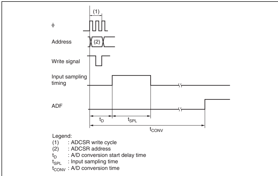
Figure 24.7 A/D Conversion Timing
