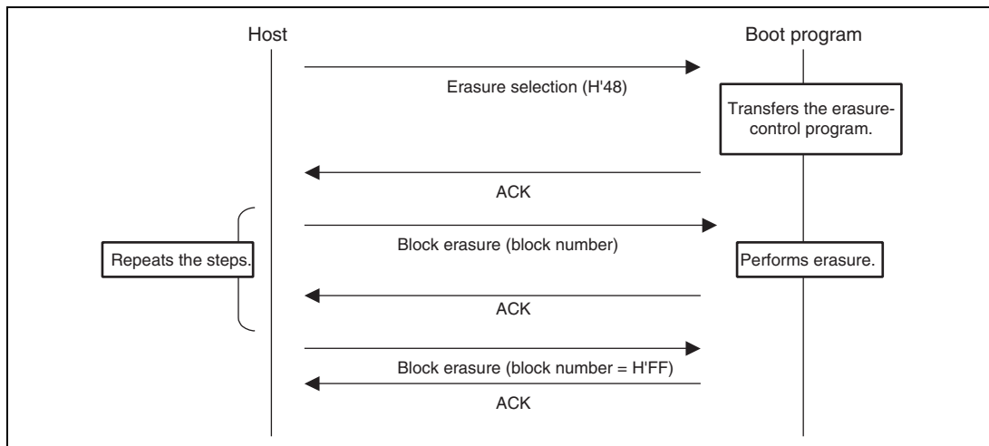
Figure 7.11 Erasure Sequence
