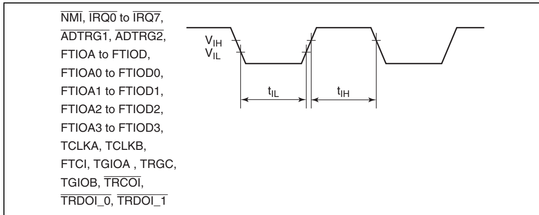
Figure 28.4 Input Timing
