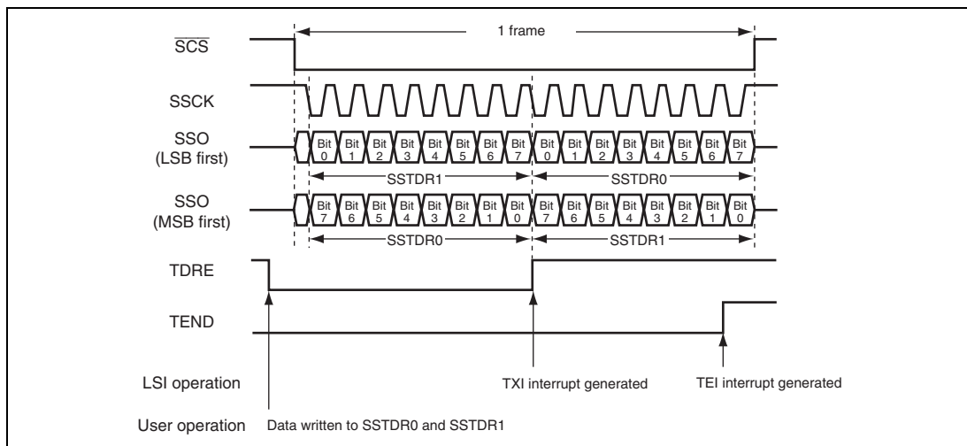
Figure 19.5 (2) Example of Transmission Operation (SSU Mode) When 16-Bit Data Length is Selected (SSTDRO and SSTDR1 are Valid) with CPOS = 0 and CPHS = 0
