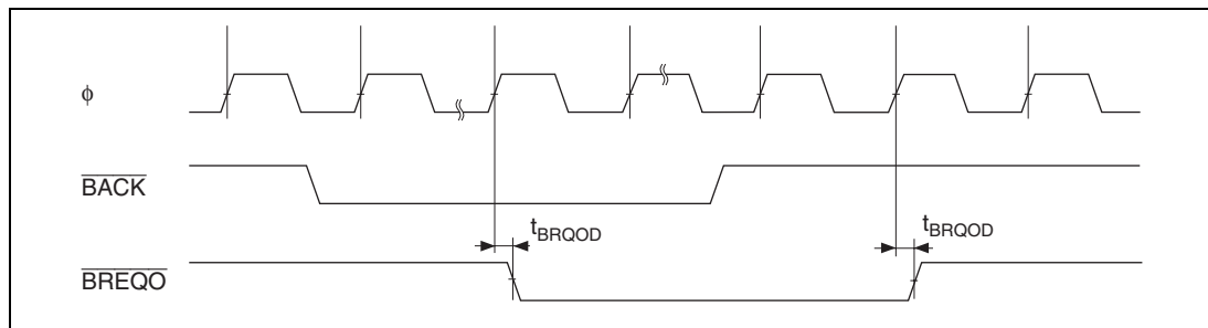
Figure 25.25 External Bus Request Output Timing
