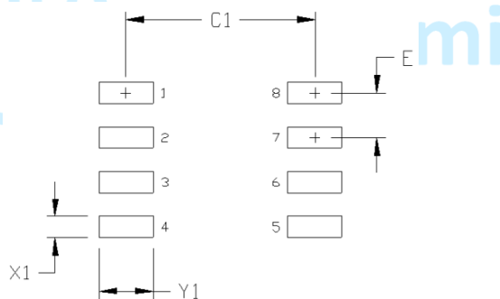
Figure 13.8-Lead Narrow Body SOIC [NB SOIC-8] Land Pattern
