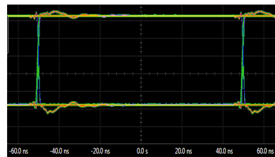
Figure 10. \pi 110M3x Eye Diagram
