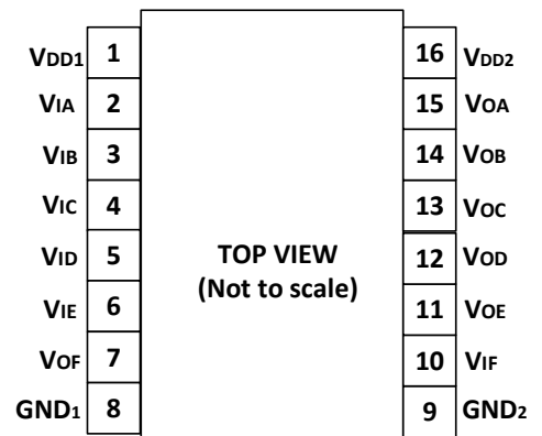
Figure4. \pi 161Uxx Pin Configuration
