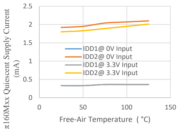
Figure 10. \pi 160Mxx Quiescent Supply Current with 3.3V Supply vs. Free-Air Temperature
