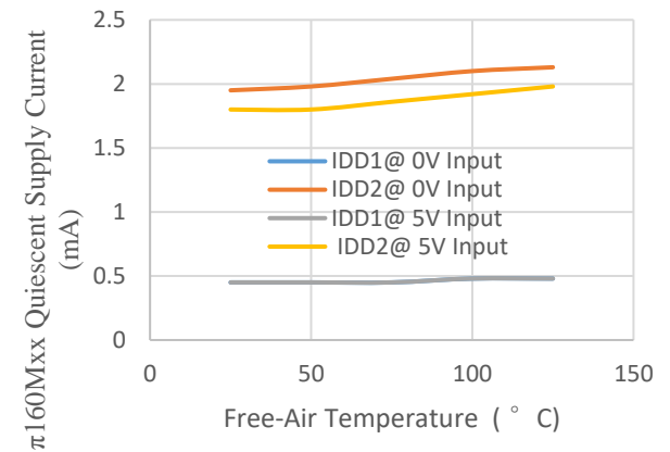
Figure 11. \pi 160Mxx Quiescent Supply Current with 5.0V Supply vs. Free-Air Temperature
