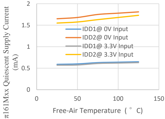
Figure 12. \pi 161Mxx Quiescent Supply Current with 3.3V Supply vs. Free-Air Temperature
