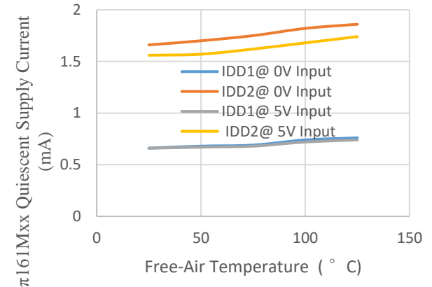
Figure 13. \pi 161Mxx Quiescent Supply Current with 5.0V Supply vs. Free-Air Temperature
