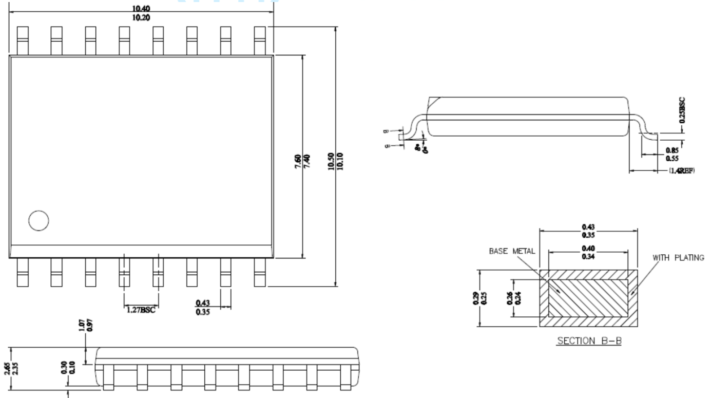
Figure23. 16-Lead Wide Body Outline Package [16-Lead SOIC_W]
