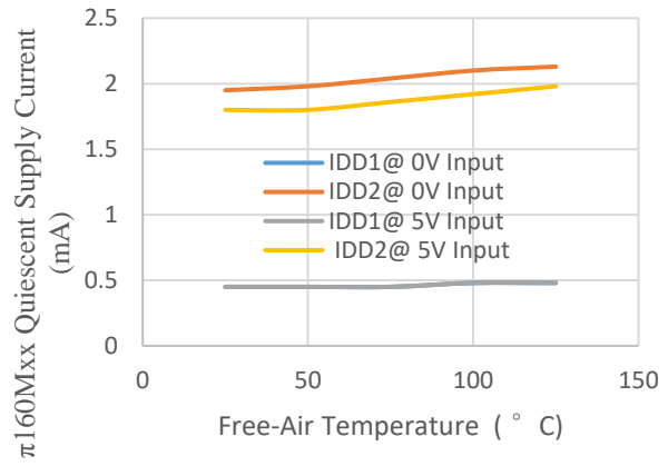
Figure 11. \pi 160Mxx Quiescent Supply Current with 5.0V Supply vs. Free-Air Temperature
