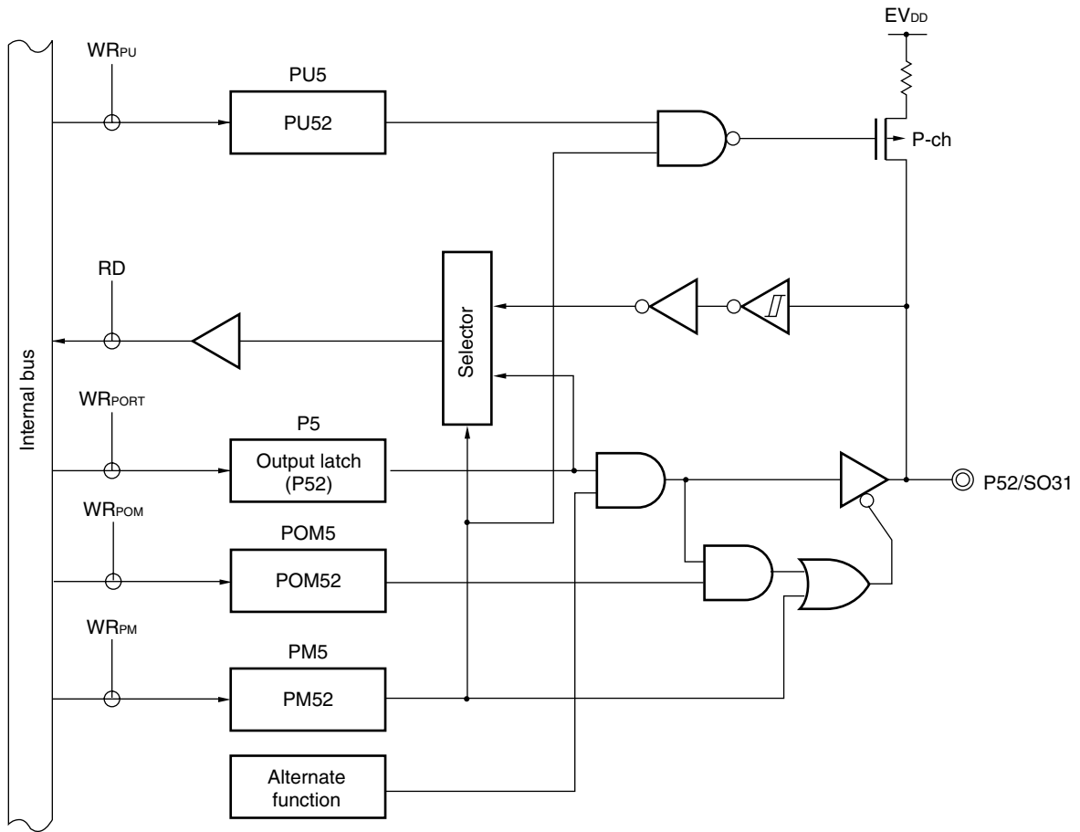
Figure 4-29. Block Diagram of P52
