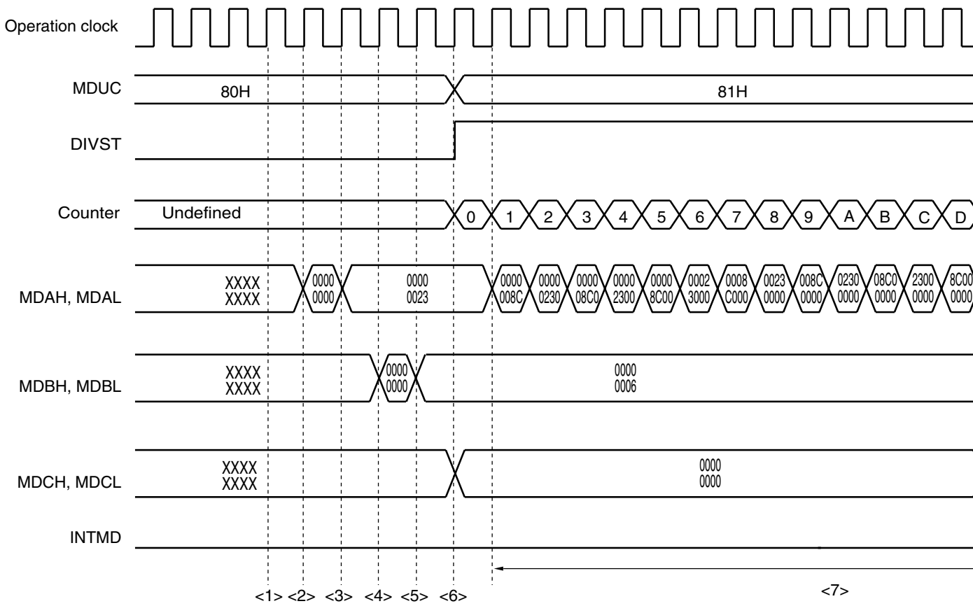
Figure 14-10. Timing Diagram of Division Operation (Example: 35 \div 6 = 5 , Remainder 5)
