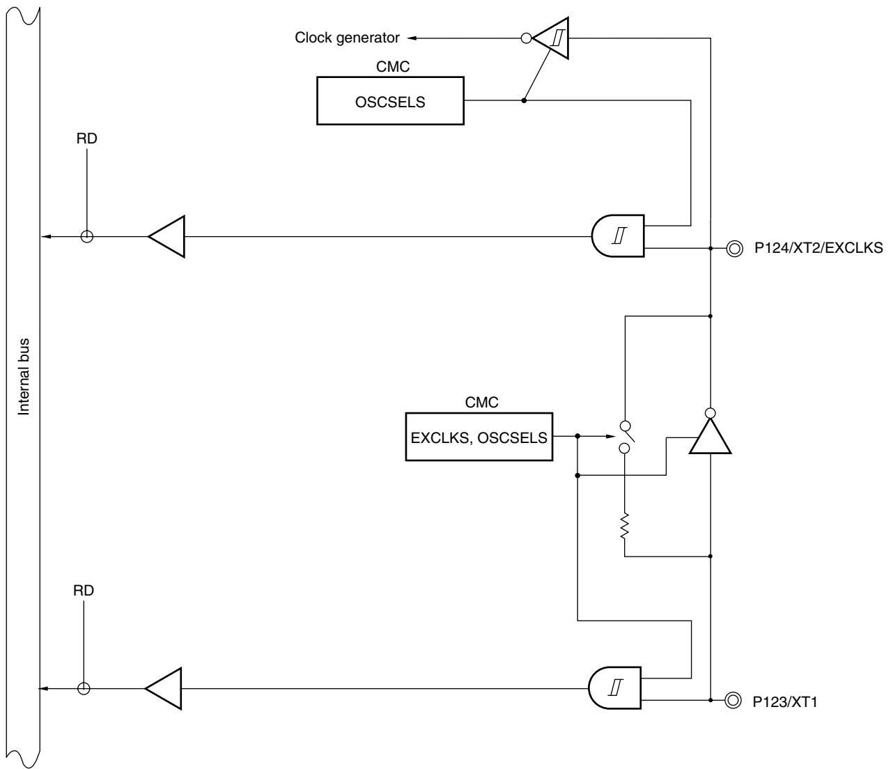
Figure 4-53. Block Diagram of P123 and P124
