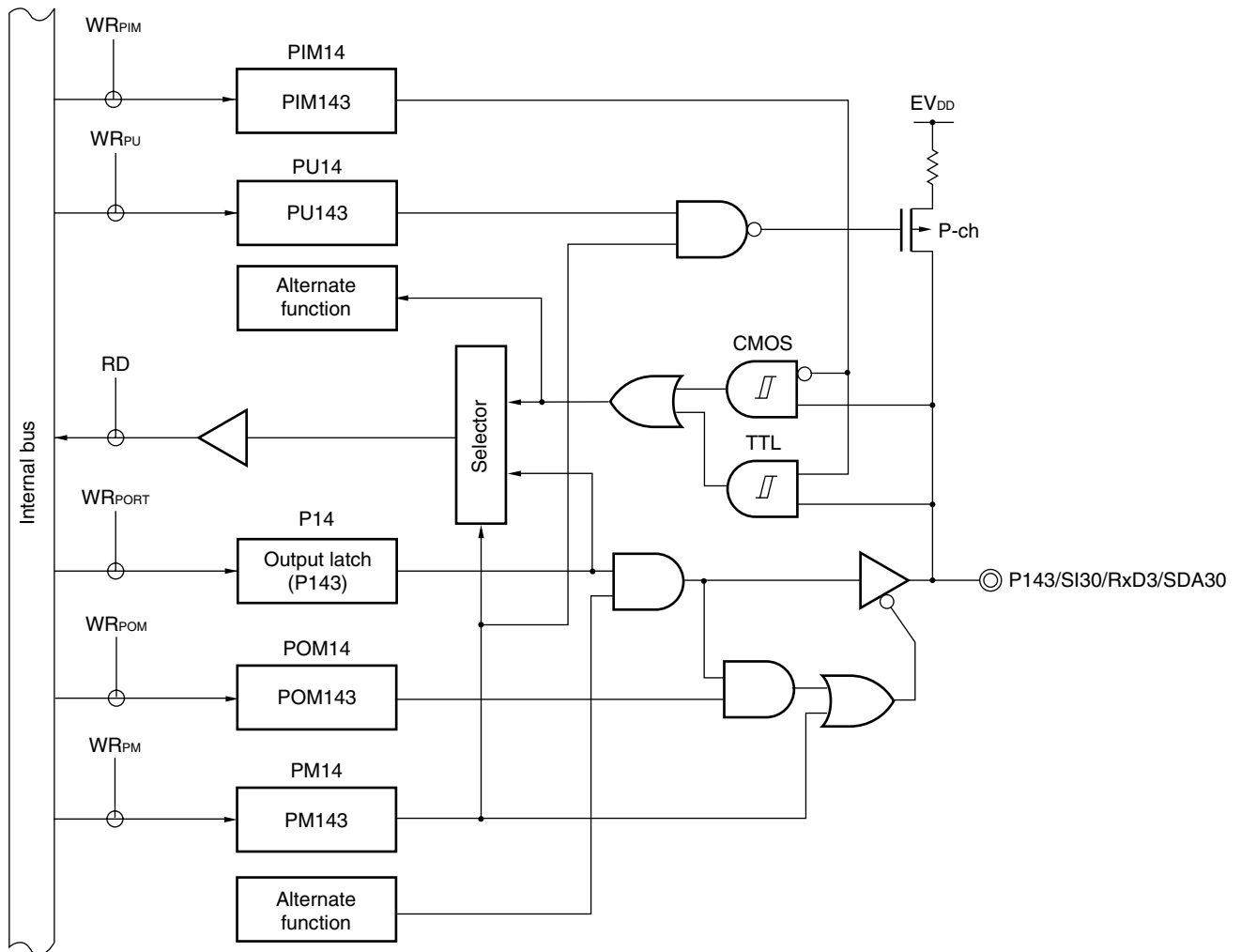
Figure 4-59. Block Diagram of P143
