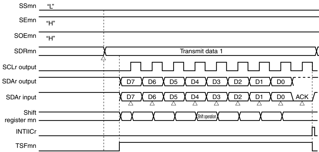
Figure 12-110. Timing Chart of Data Transmission
