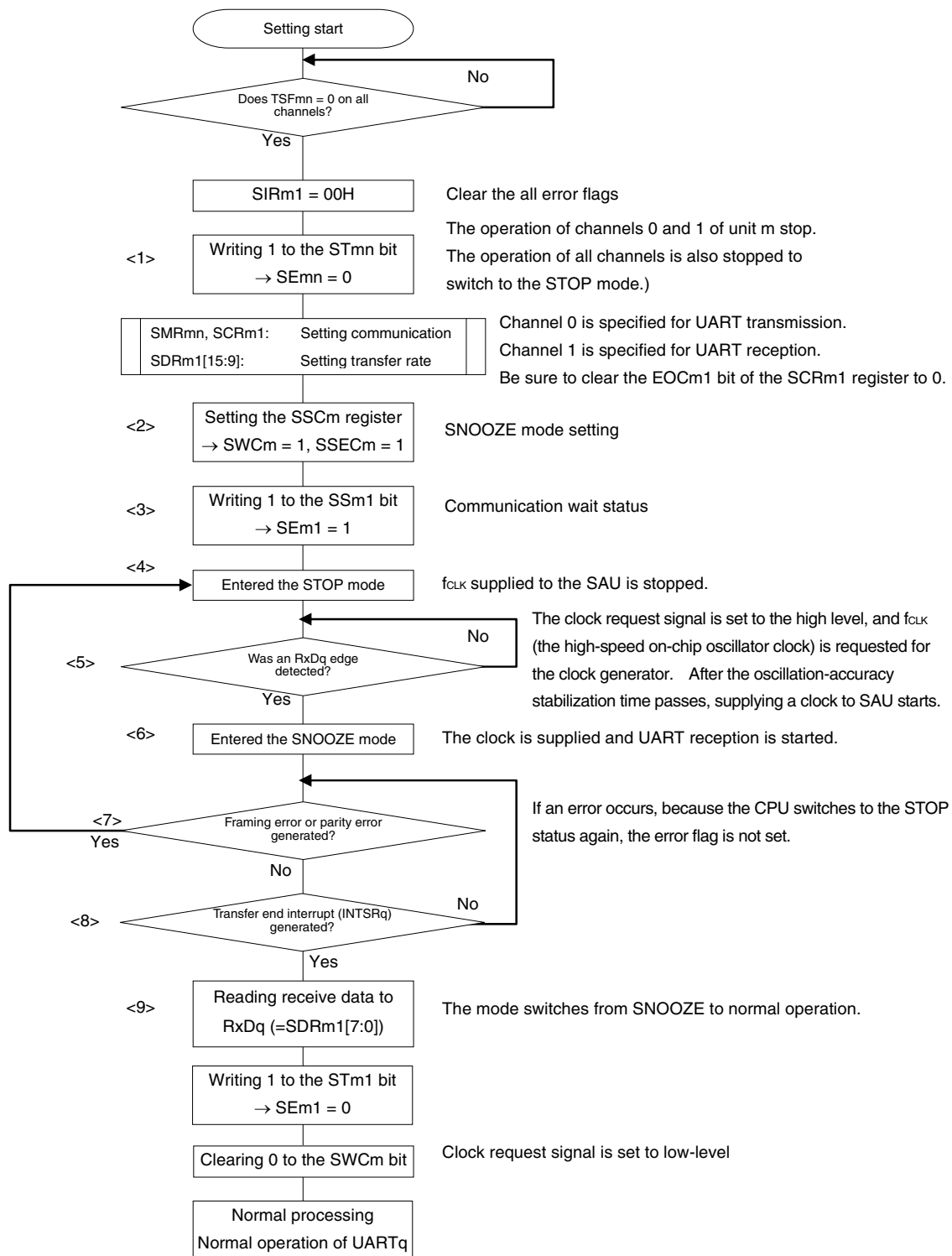
Figure 12-95. Flowchart of SNOOZE Mode Operation (Abnormal Operation <2>)
