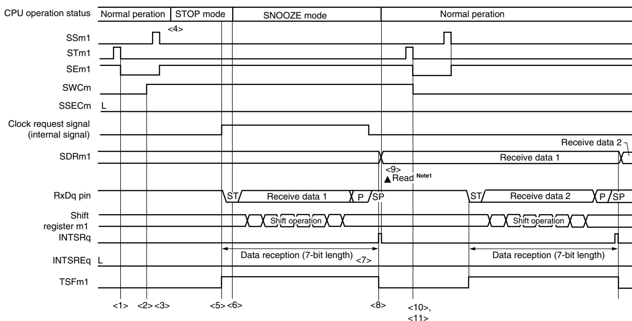
Figure 12-91. Timing Chart of SNOOZE Mode Operation (Normal operation mode)
