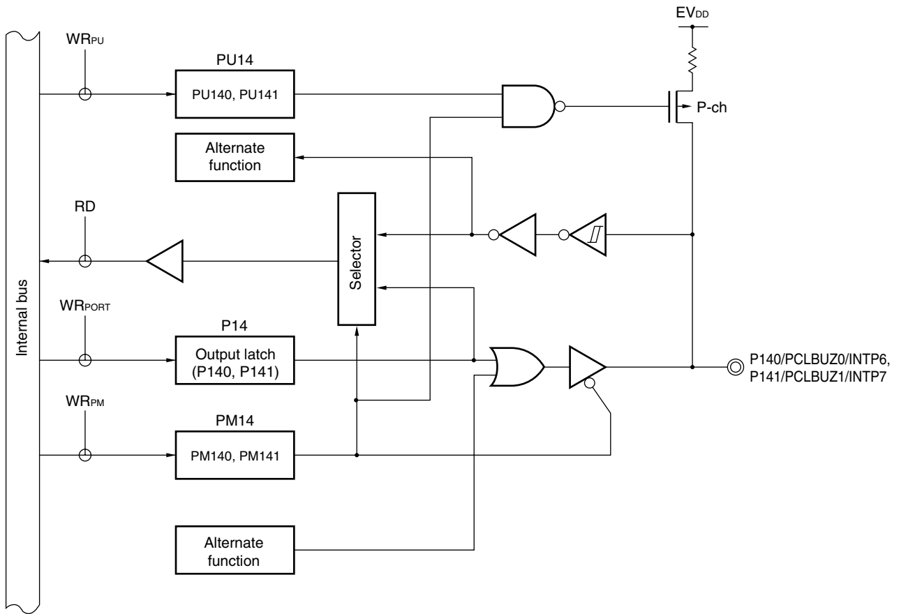
Figure 4-57. Block Diagram of P140 and P141
