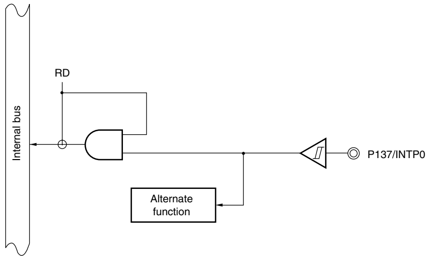
Figure 4-56. Block Diagram of P137
