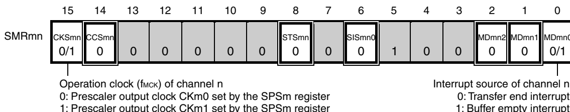
Figure 12-34. Example of Contents of Registers for Master Reception of 3-Wire Serial I/O (CSI00, CSI01, CSI10, CSI11, CSI20, CSI21, CSI30, CSI31) (1/2)
