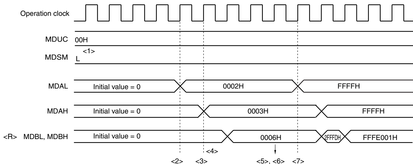
Figure 14-6. Timing Diagram of Multiplication (Unsigned) Operation (2 × 3 = 6)
