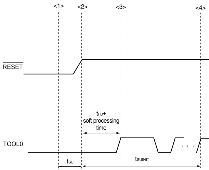
Figure 25-8. Setting of Flash Memory Programming Mode
