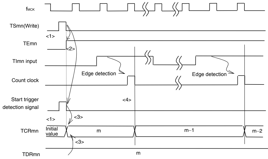
Figure 6-24. Start Timing (In Event Counter Mode)
