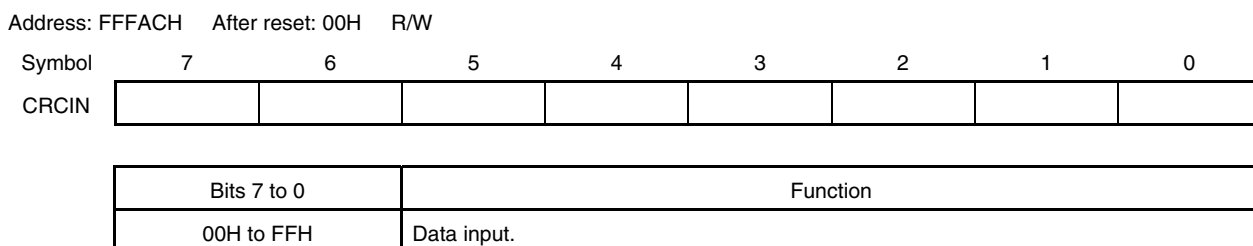
Figure 22-4. Format of CRC Input Register (CRCIN)
