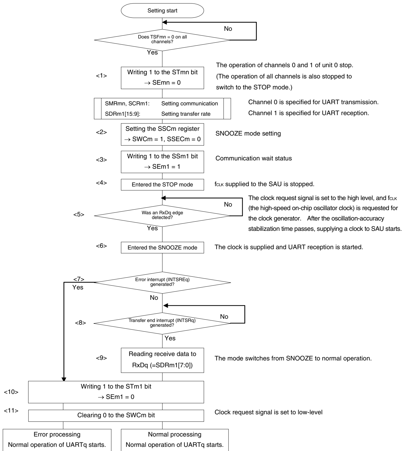
Figure 12-93. Flowchart of SNOOZE Mode Operation (Normal Operation/Abnormal Operation <1>)
