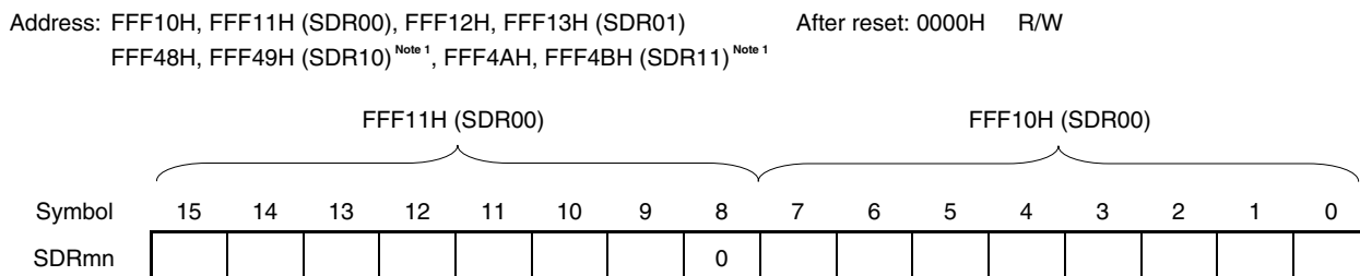
Figure 12-9. Format of Serial Data Register mn (SDRmn)
