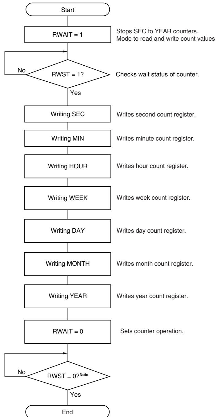
Figure 7-20. Procedure for Writing Real-time Clock
