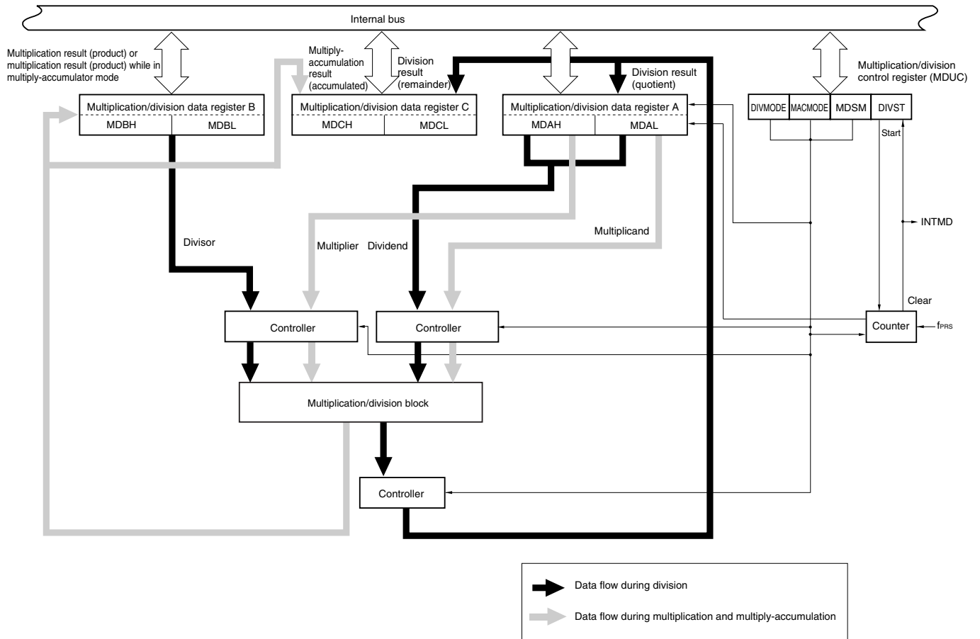
Figure 14-1. Block Diagram of Multiplier and Divider/Multiply-Accumulator
