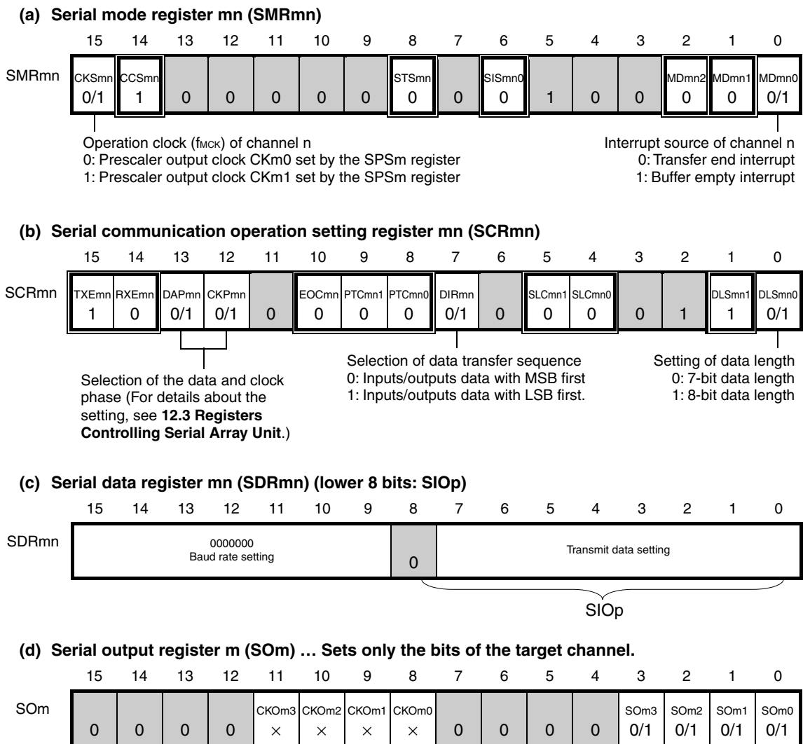
Figure 12-50. Example of Contents of Registers for Slave Transmission of 3-Wire Serial I/O (CSI00, CSI01, CSI10, CSI11, CSI20, CSI21, CSI30, CSI31) (1/2)
