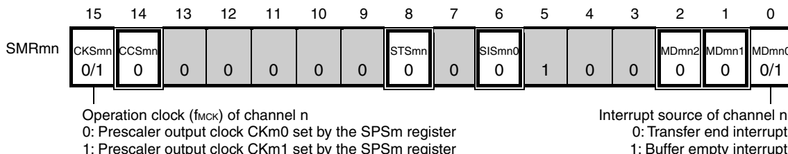
Figure 12-26. Example of Contents of Registers for Master Transmission of 3-Wire Serial I/O (CSI00, CSI01, CSI10, CSI11, CSI20, CSI21, CSI30, CSI31) (1/2)
