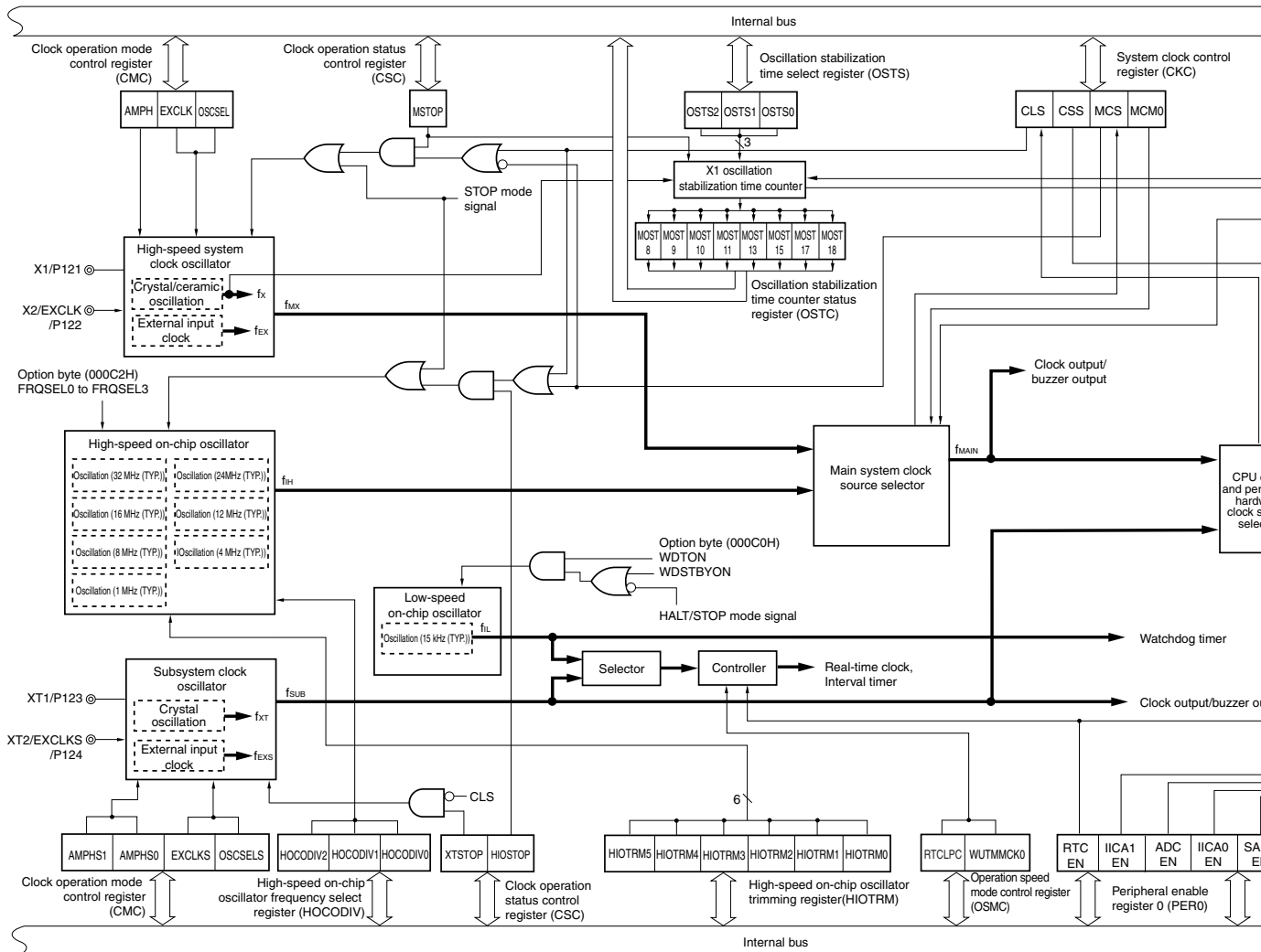
Figure 5-1. Block Diagram of Clock Generator
