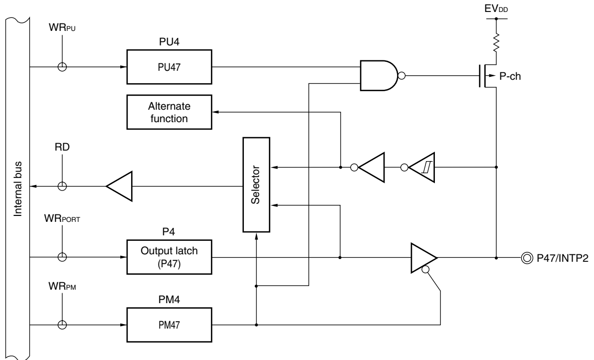
Figure 4-26. Block Diagram of P47
