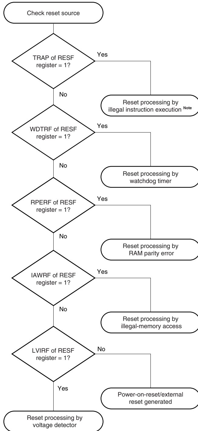
Figure 21-7. Checking reset source
