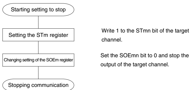
Figure 12-66. Procedure for Stopping Slave Transmission/Reception
