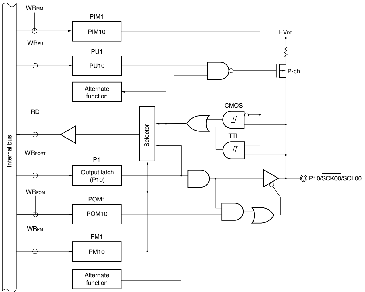
Figure 4-7. Block Diagram of P10
