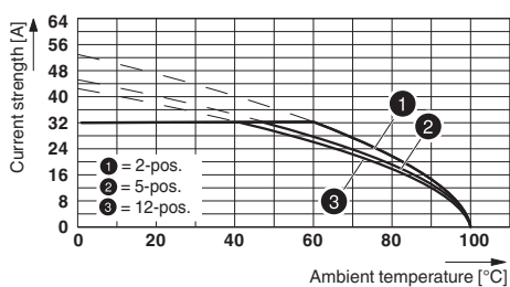
Derating curve for: PC 5/...-ST1-7,62 with PC 4/...-G-7,62
