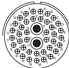
32-59 A 40 2 16 8 (Coax) RG-161/U
