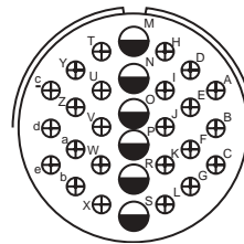
32-56 A 24 6 16 12 for #10 wire
