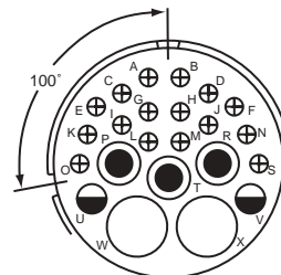
100° Rotation of 32-6
