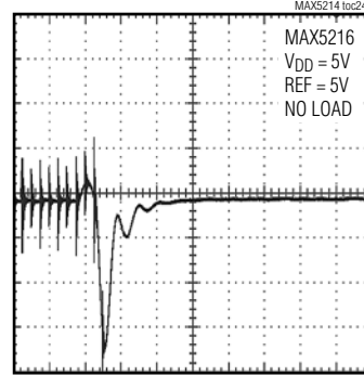
MAJOR CODE TRANSITION (0x7FFF TO 0x8000)
