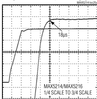
SETTLING TO \pm 0.5 LSB 14 BIT ( V_{DD} = V_{REF} = 5\text{V} , C_L = 100\text{pF} )
