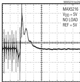
MAJOR CODE TRANSITION (0x8000 TO 0x7FFF)
