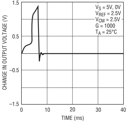
Turn-On Characteristics
