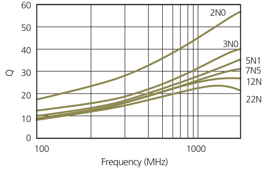
Q CHARACTERISTIC
