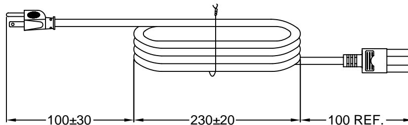
HANKING DETAIL
